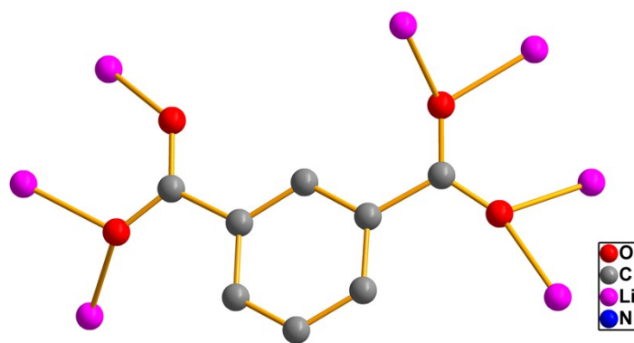
Fig. S1 Coordination mode of IPA 2- ligand.
