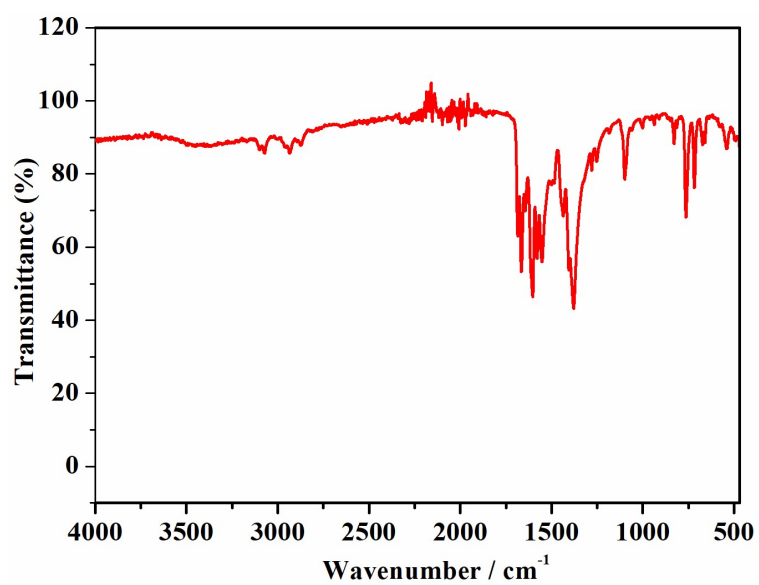
Fig. S4 IR spectrum of compound 1 .
