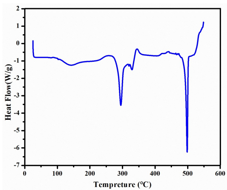
Fig. S3 DSC curve of complex 1.
