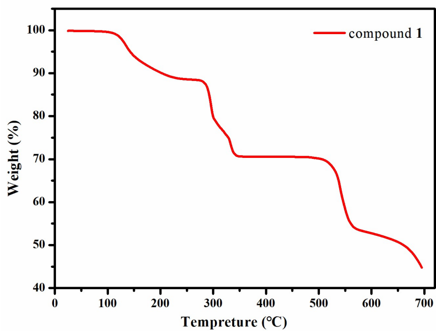
Fig. S2 Thermogravimetric profile for 1.
