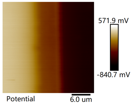
Fig.S4 KPFM surface potential distribution images of Au-Si-Al standard sample
