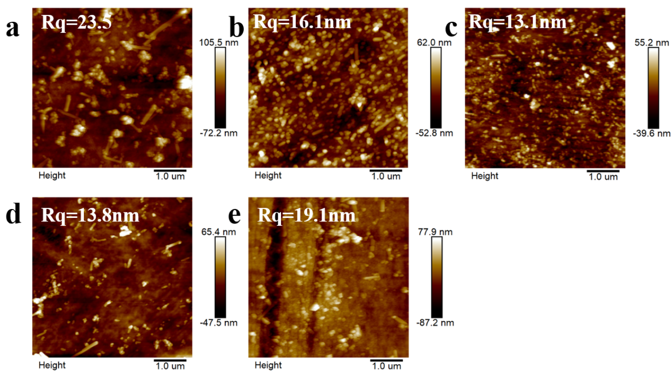
Fig.S2 AFM morphology of CuPc film and iodine doped CuPc films (a) CuPc, (b) CuPc doped with concentration of 5 wt% iodine, (c) CuPc doped with concentration of 10 wt% iodine, (d) CuPc doped with concentration of 15 wt% iodine, (e) CuPc doped with concentration of 20 wt% iodine
