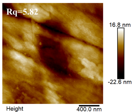
Fig.S1 AFM morphology of PET film
