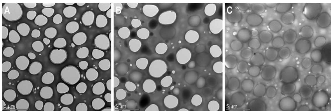
Figure S1. Overview of copper grids with and without ultrathin IL films. (A) TEM image of copper grid with no IL film. (B) TEM image of copper grid partially covered by IL film. Thick droplets can be seen next to the carbon hole after bursting of the IL films. (C) TEM image of copper grid fully covered by IL film.
