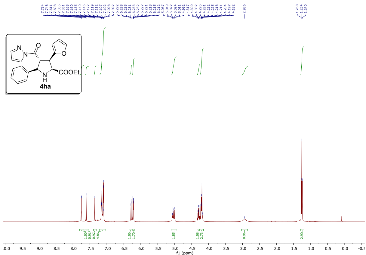
1 H NMR (500 MHz, CDCl 3 ) of compound 4ha
