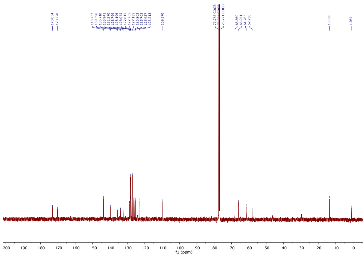
13 C NMR (125 MHz, CDCl 3 ) of compound 4ja
