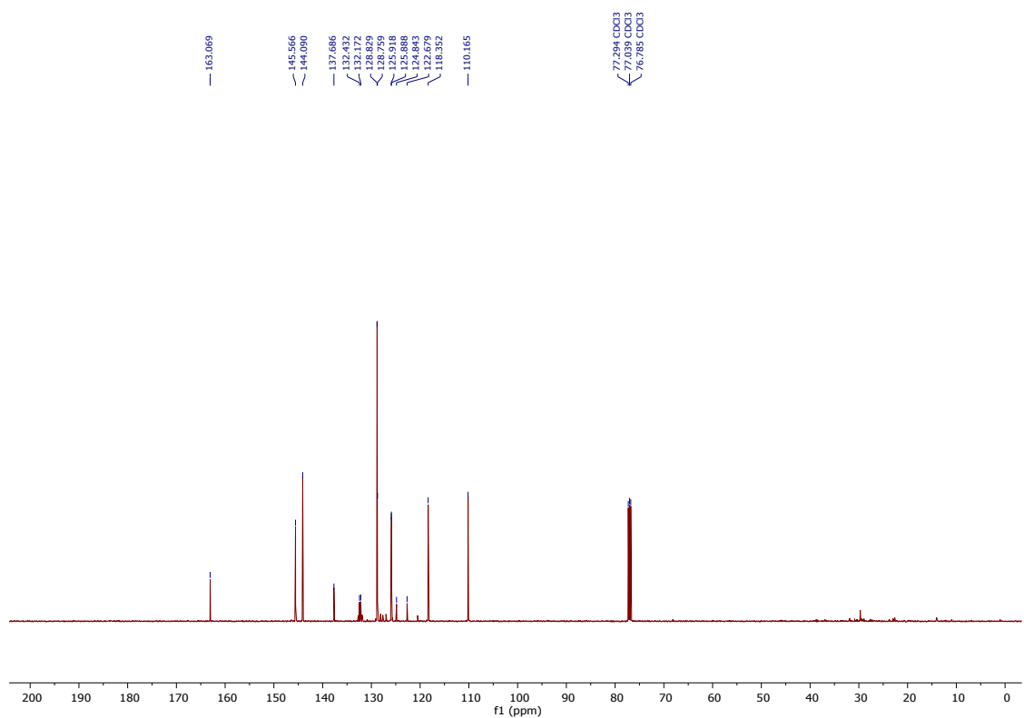
^{13}\text{C} NMR (125 MHz, \text{CDCl}_3 ) of compound 2e
