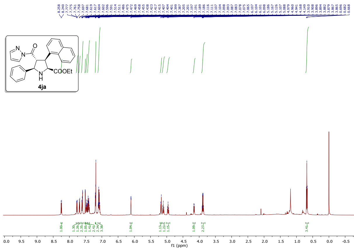
1 H NMR (500 MHz, CDCl 3 ) of compound 4ja
