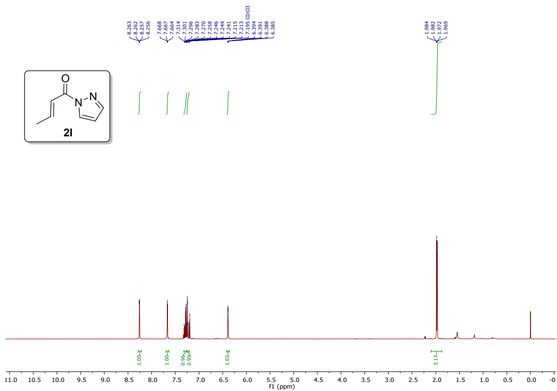
1 H NMR (500 MHz, CDCl 3 ) of compound 2I
