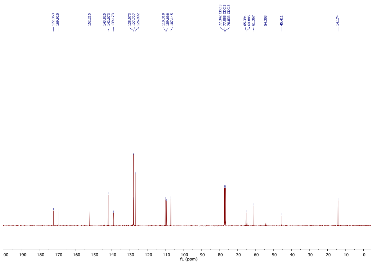
13 C NMR (125 MHz, CDCl 3 ) of compound 4ha
