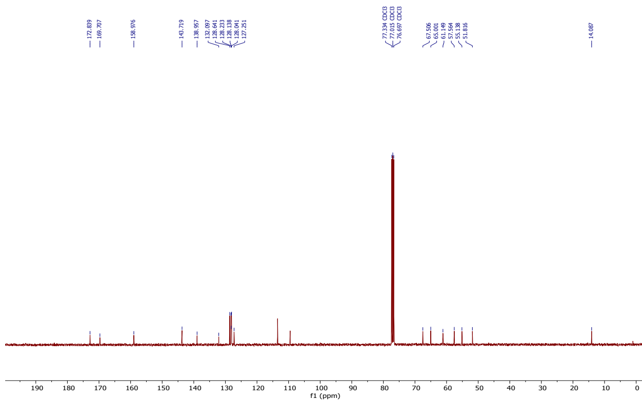
13 C NMR (100 MHz, CDCl 3 ) of compound 4ac
