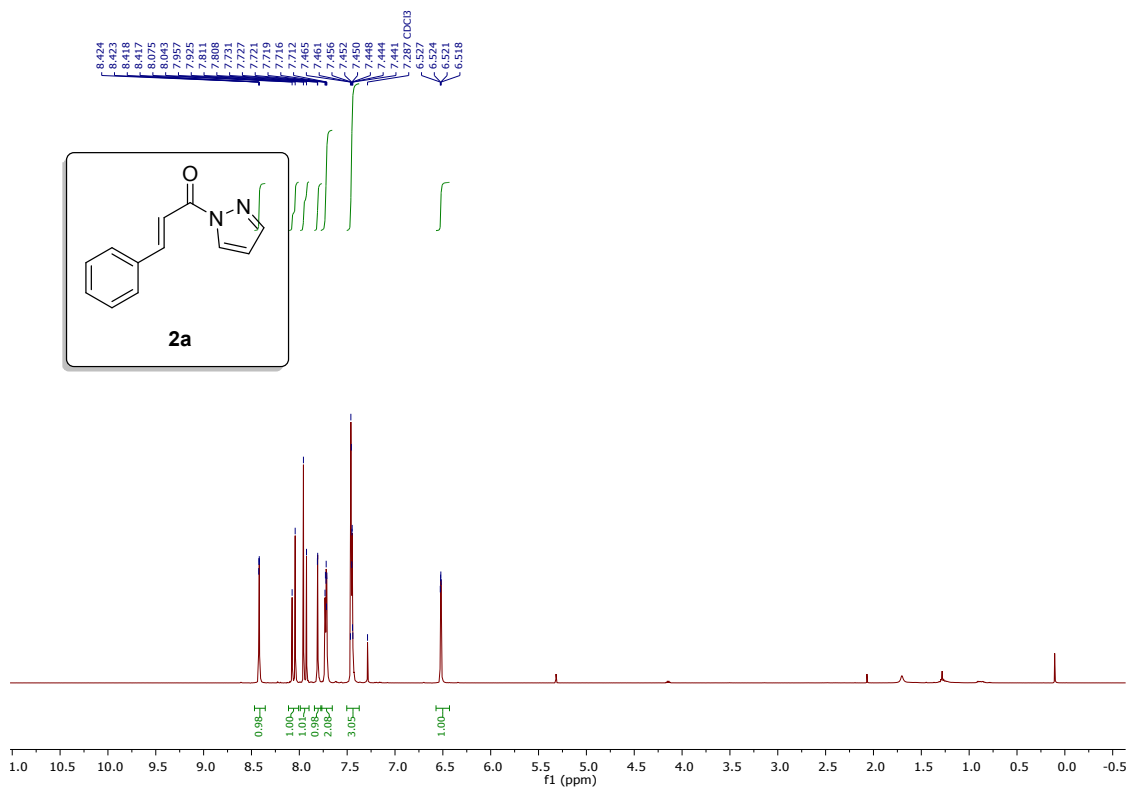
1 H NMR (500 MHz, CDCl 3 ) of compound 2a
