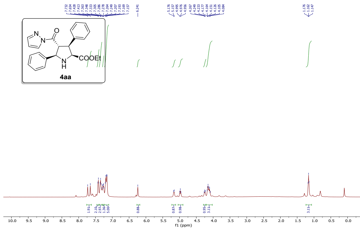
1 H NMR (500 MHz, CDCl 3 ) of compound 4aa
