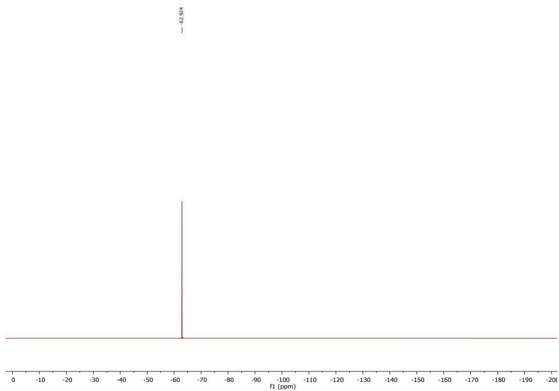
^{19}\text{F} NMR (470 MHz, \text{CDCl}_3 ) of compound 2e
