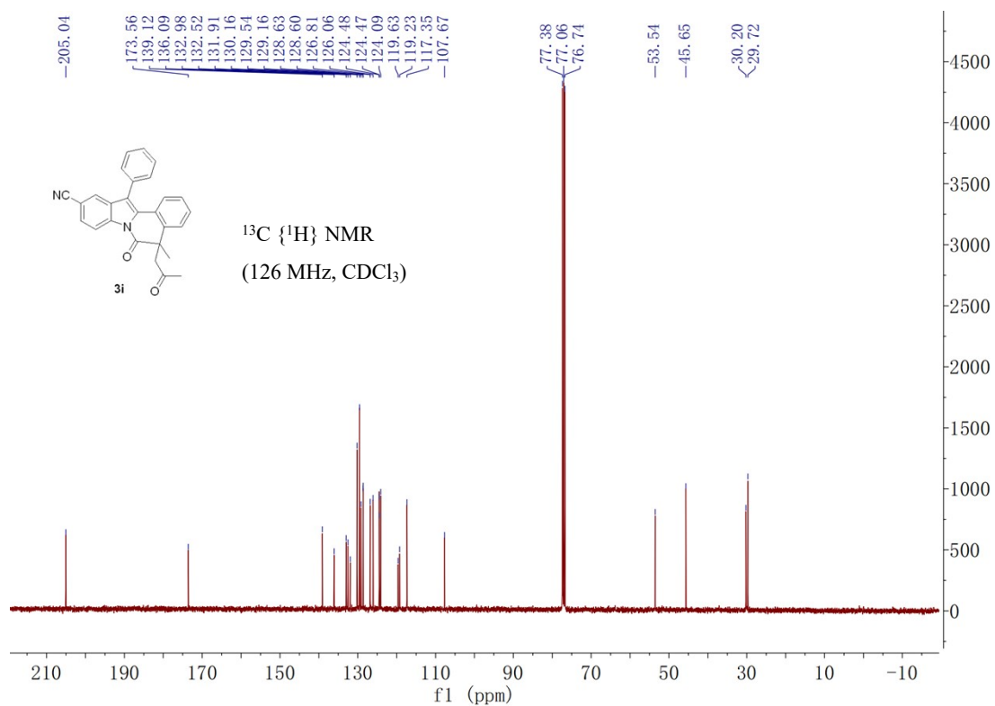
5-methyl-6-oxo-5-(2-oxo-2-phenylethyl)-12-phenyl-5,6-dihydroindolo[2,1-a]isoquinoline-10-carbonitrile 3j
