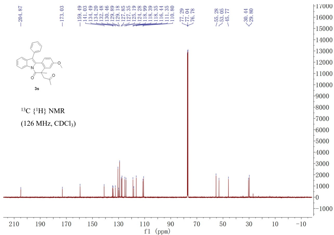
3-methoxy-5-methyl-5-(2-oxo-2-phenylethyl)-12-phenylindolo[2,1-a]isoquinolin-6(5H)-one 3t
