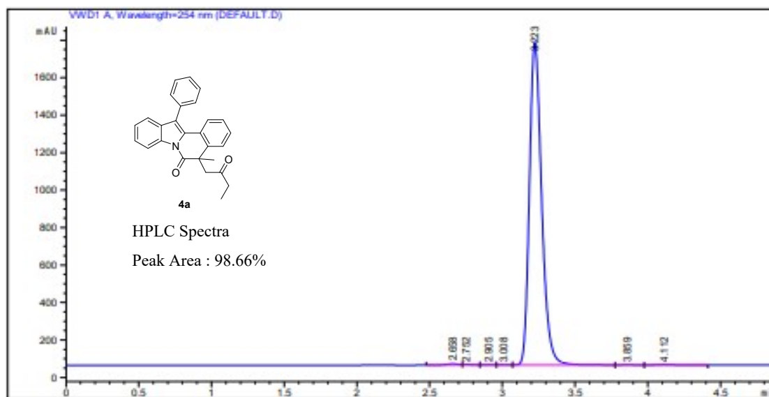
5-(2-(2-methoxyphenyl)-2-oxoethyl)-5-methyl-12-phenylindolo[2,1-a]isoquinolin-6(5H)-one 4b
