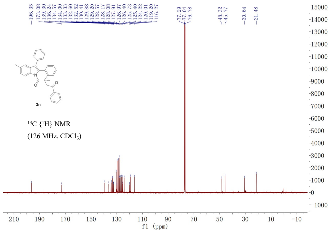
3,5-dimethyl-5-(2-oxopropyl)-12-phenylindolo[2,1-a]isoquinolin-6(5H)-one 3o
