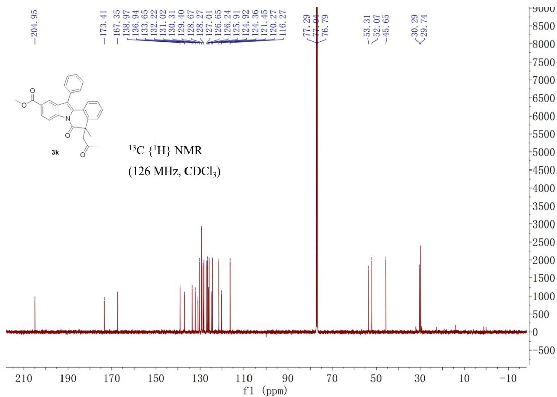
methyl 5-methyl-6-oxo-5-(2-oxo-2-phenylethyl)-12-phenyl-5,6-dihydroindolo[2,1-a]isoquinoline-10-carboxylate 3k
