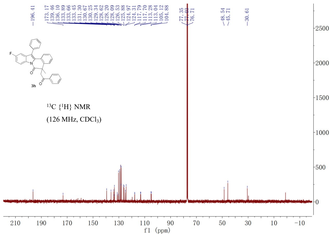
10-isocyano-5-methyl-5-(2-oxopropyl)-12-phenylindolo[2,1-a]isoquinolin-6(5H)-one 3i
