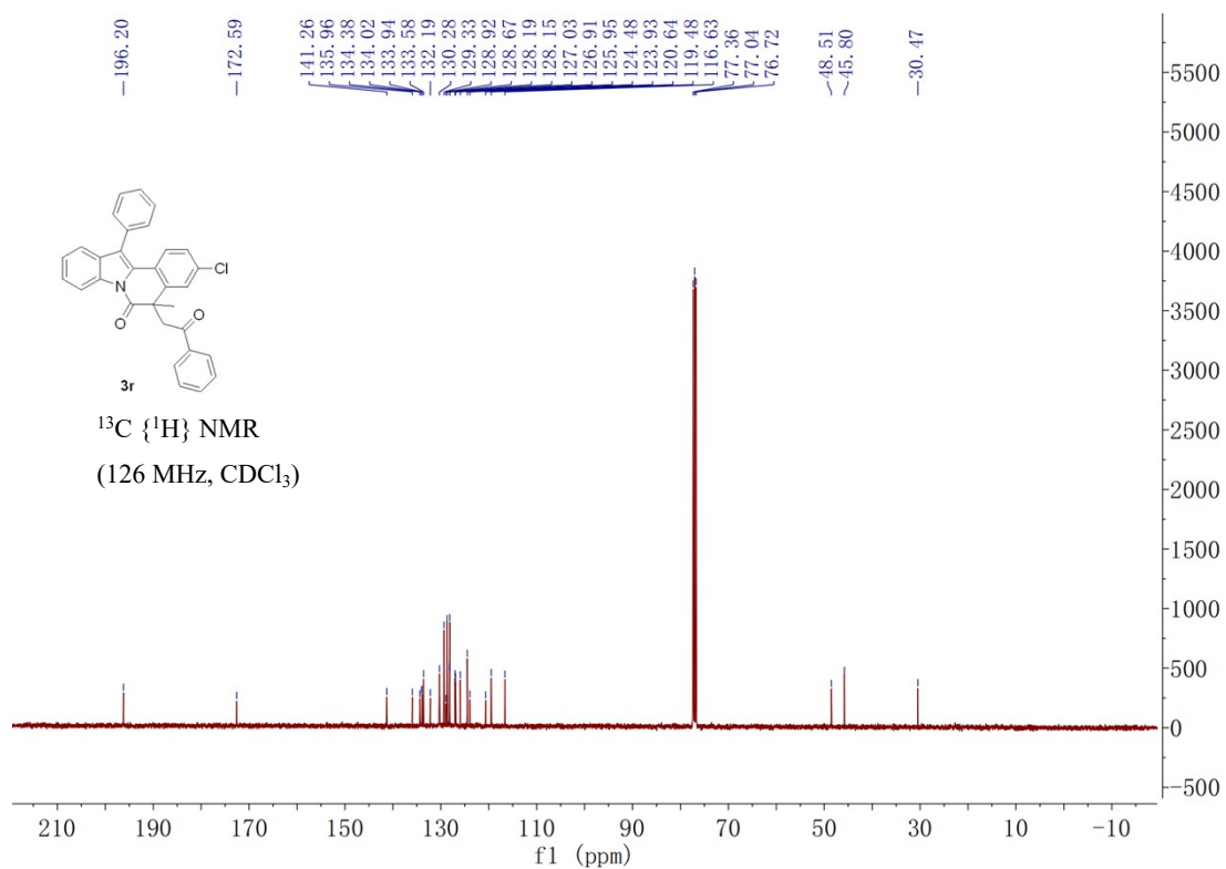
3-methoxy-5-methyl-5-(2-oxopropyl)-12-phenylindolo[2,1-a]isoquinolin-6(5H)-one 3s
