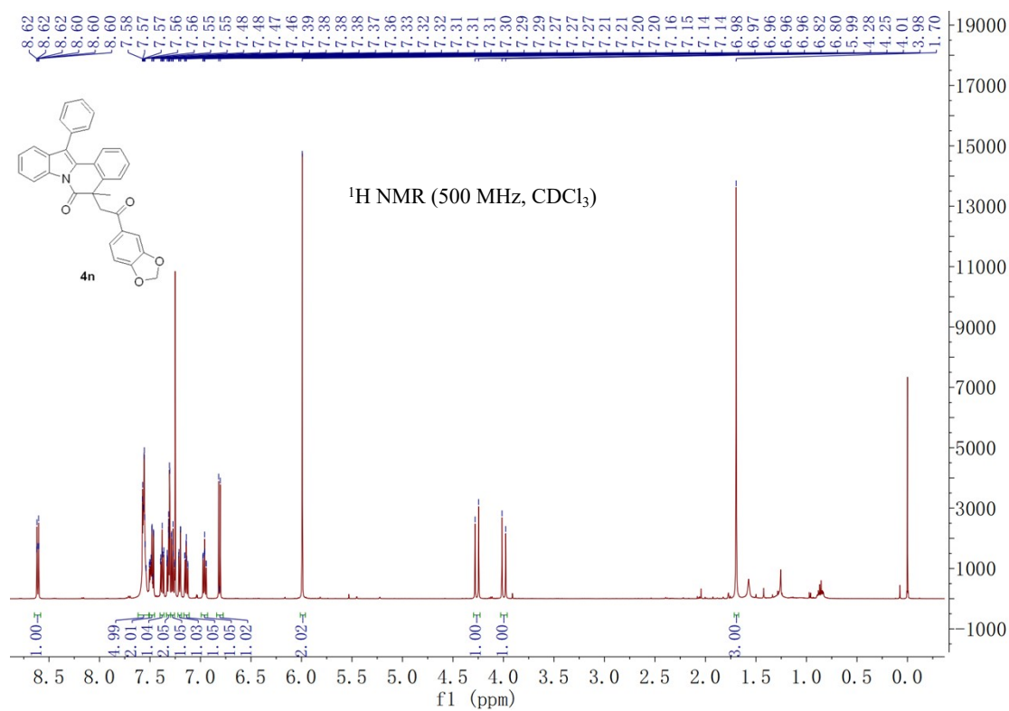
5-(2-(benzo[d][1,3]dioxol-5-yl)-2-oxoethyl)-5-methyl-12-phenylindolo[2,1-a]isoquinolin-6(5H)-one 4n
