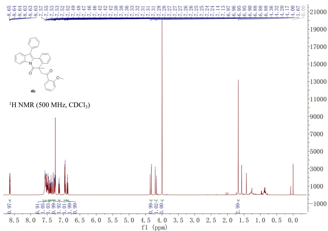
5-(2-(2-methoxyphenyl)-2-oxoethyl)-5-methyl-12-phenylindolo[2,1-a]isoquinolin-6(5H)-one 4b
