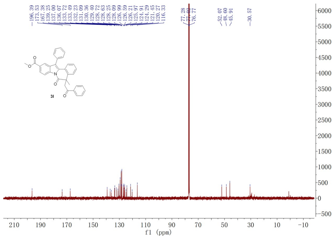
5,10-dimethyl-5-(2-oxopropyl)-12-phenylindolo[2,1-a]isoquinolin-6(5H)-one 3m
