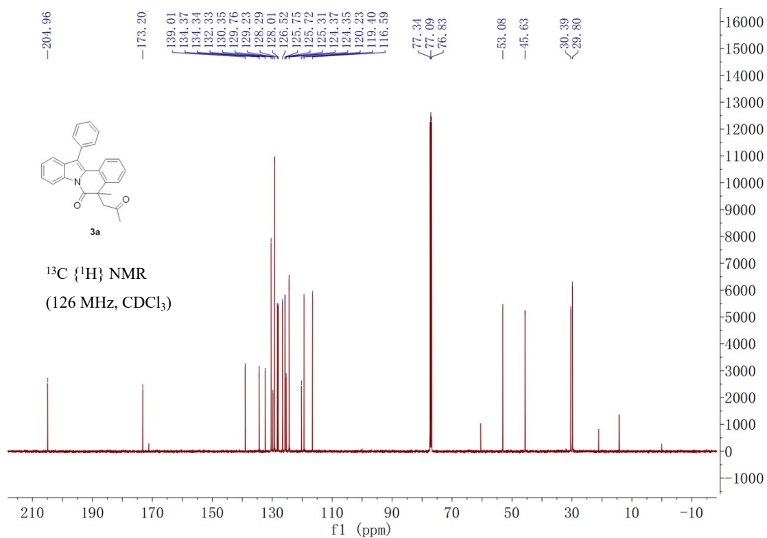
5-methyl-5-(2-oxo-2-phenylethyl)-12-phenylindolo[2,1-a]isoquinolin-6(5H)-one 3b
