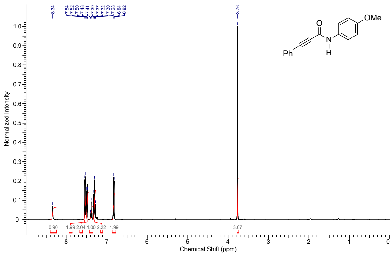
1 H NMR spectrum of the compound 4ab
