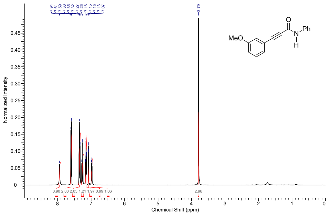
1 H NMR spectrum of the compound 4ka
