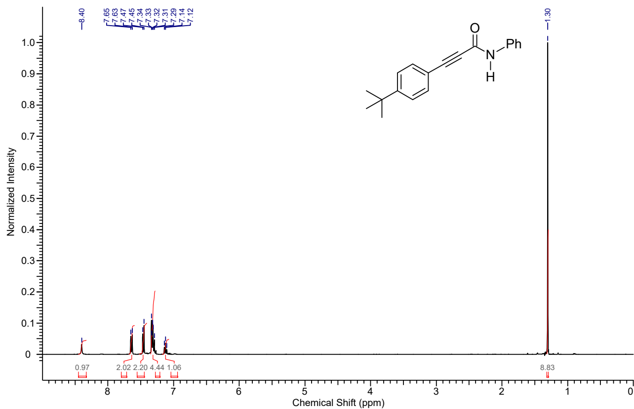
^1\text{H} NMR spectrum of the compound 4da
