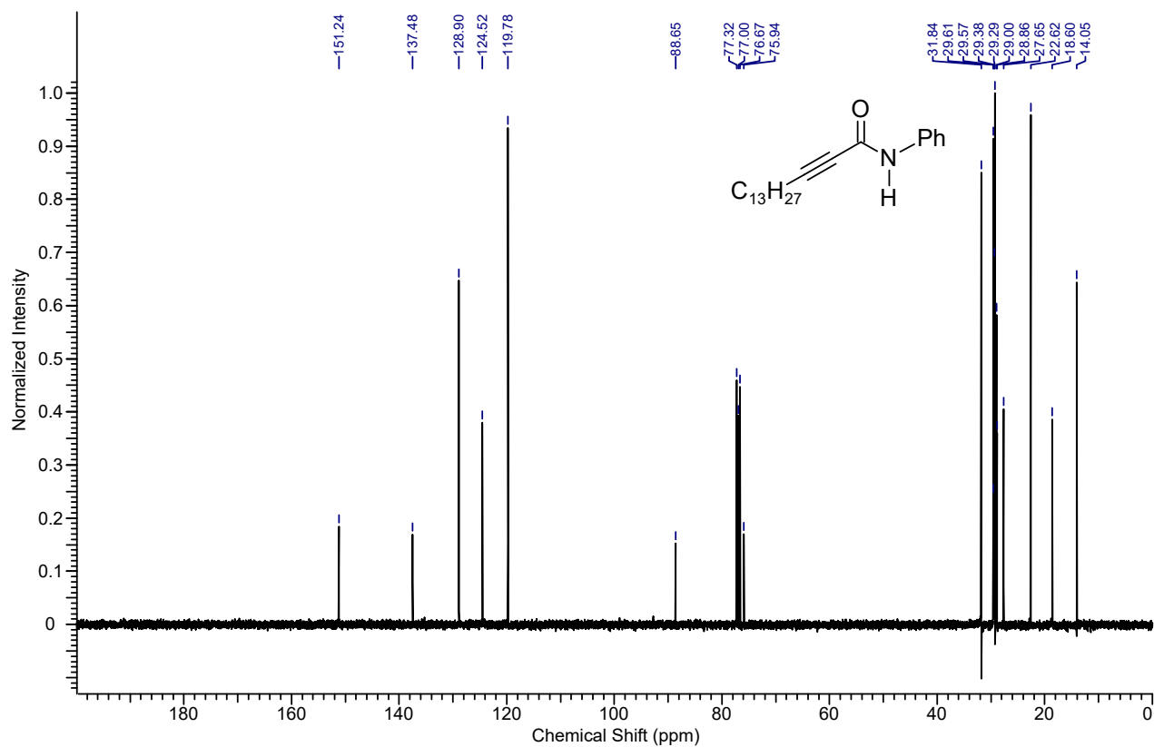
13 C NMR spectrum of the compound 7b
