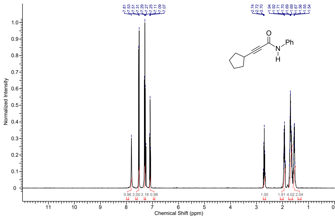
1 H NMR spectrum of the compound 7h
