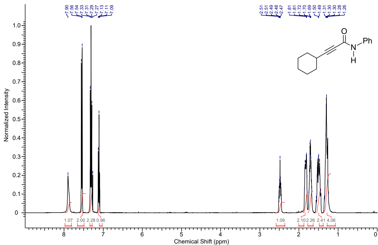
1 H NMR spectrum of the compound 7g
