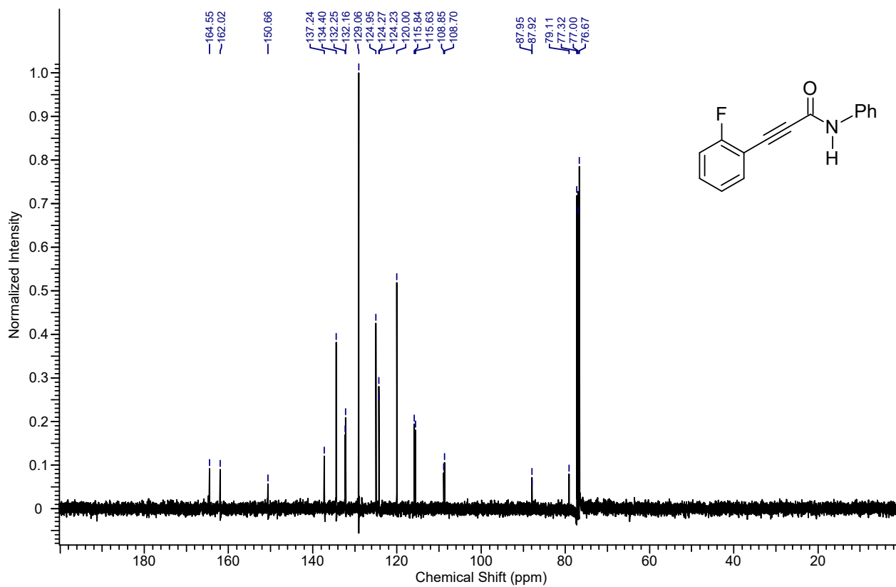
13 C NMR spectrum of the compound 4na
