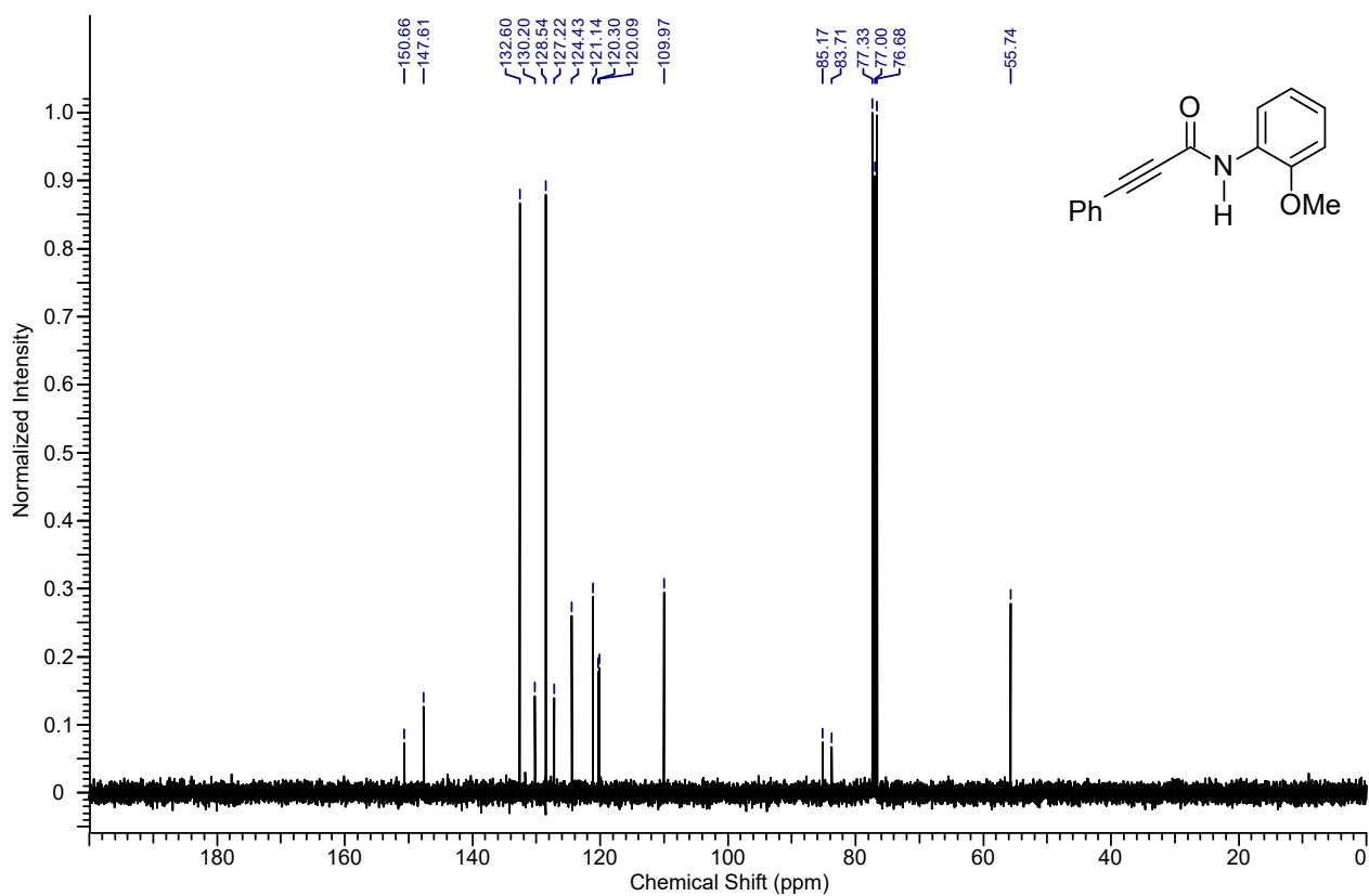
13 C NMR spectrum of the compound 4aj
