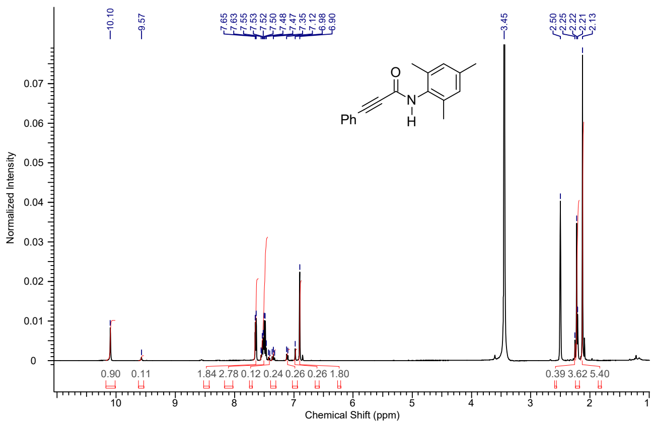
1 H NMR spectrum of the compound 4am (a 9:1 mixture of rotamers)
