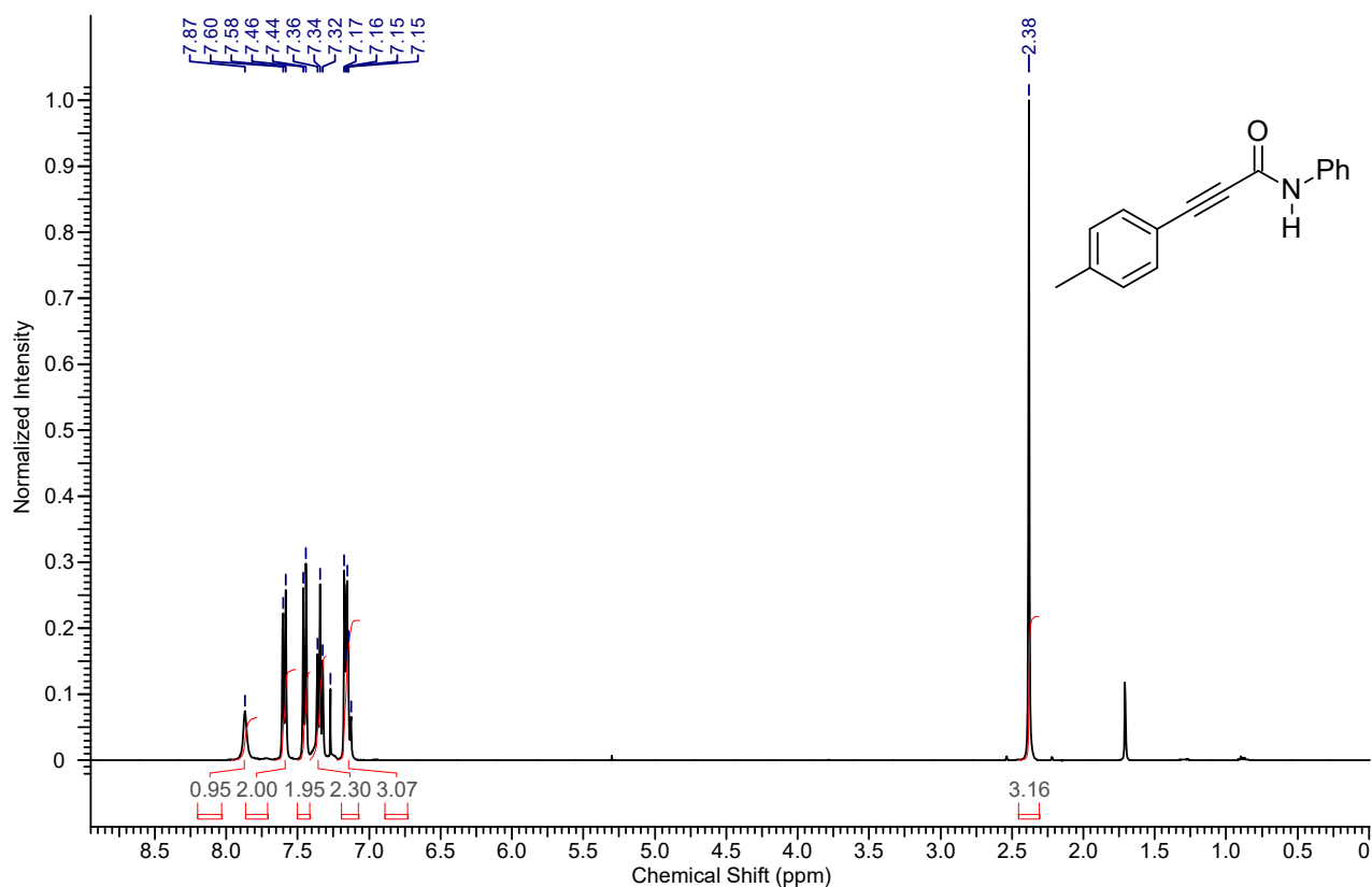
1 H NMR spectrum of the compound 4ca
