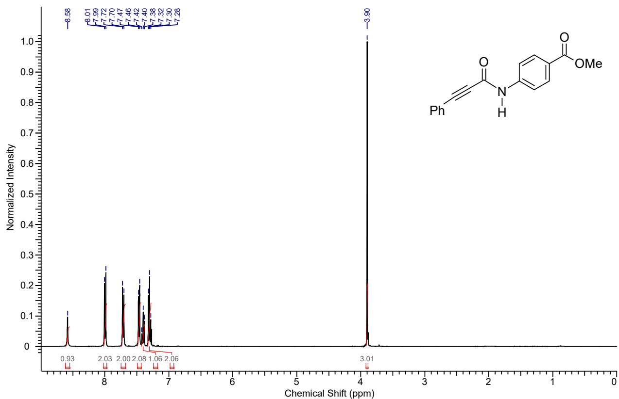
^1\text{H} NMR spectrum of the compound 4ah
