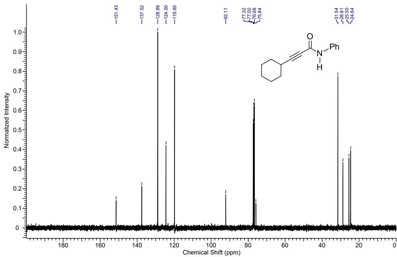
13 C NMR spectrum of the compound 7g
