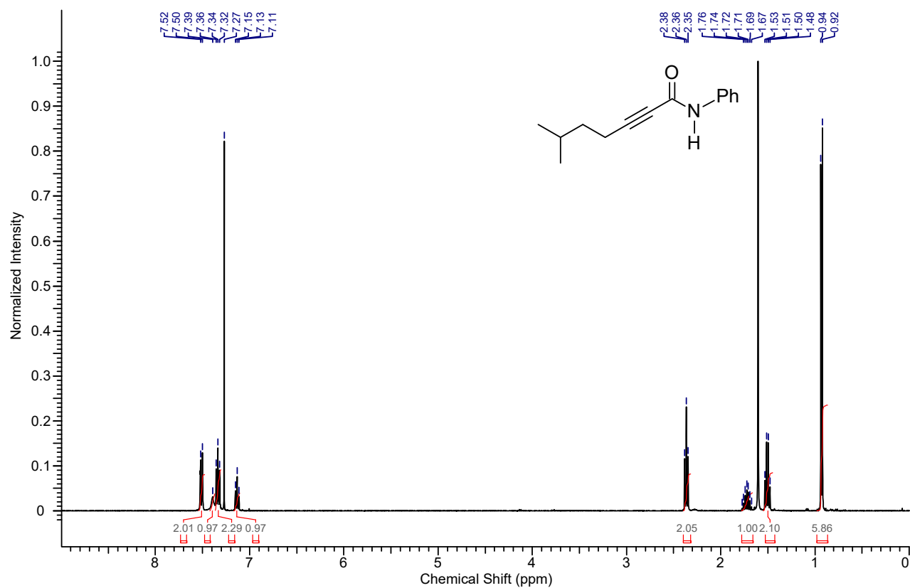
1 H NMR spectrum of the compound 7c
