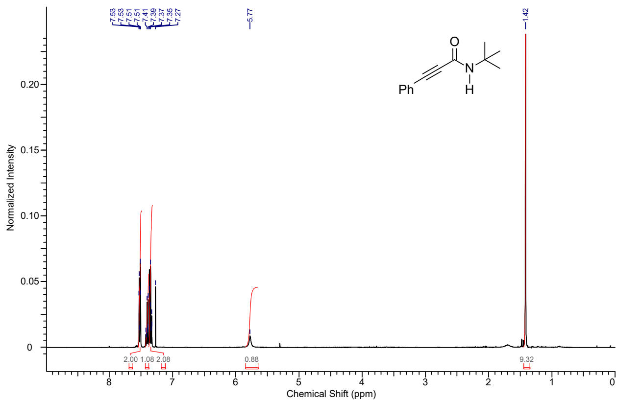
1 H NMR spectrum of the compound 4as
