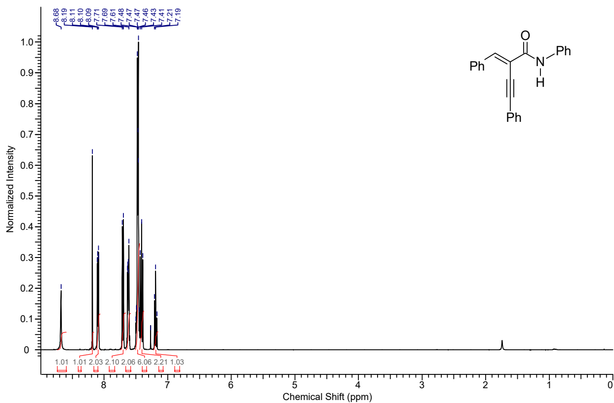
1 H NMR spectrum of the compound 5aa
