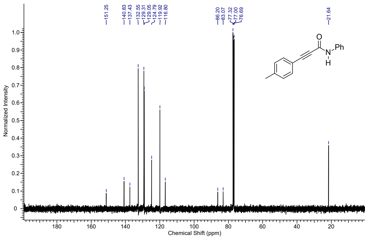
13 C NMR spectrum of the compound 4ca
