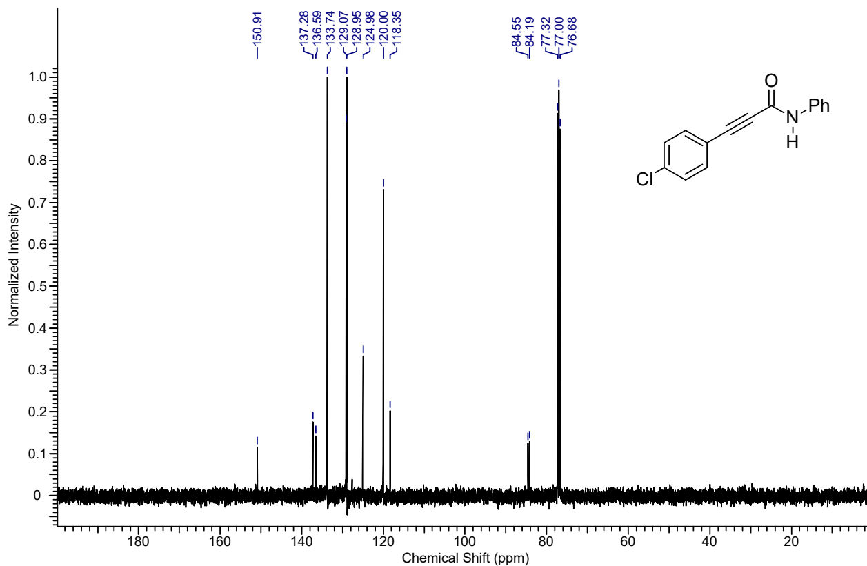
13 C NMR spectrum of the compound 4fa
