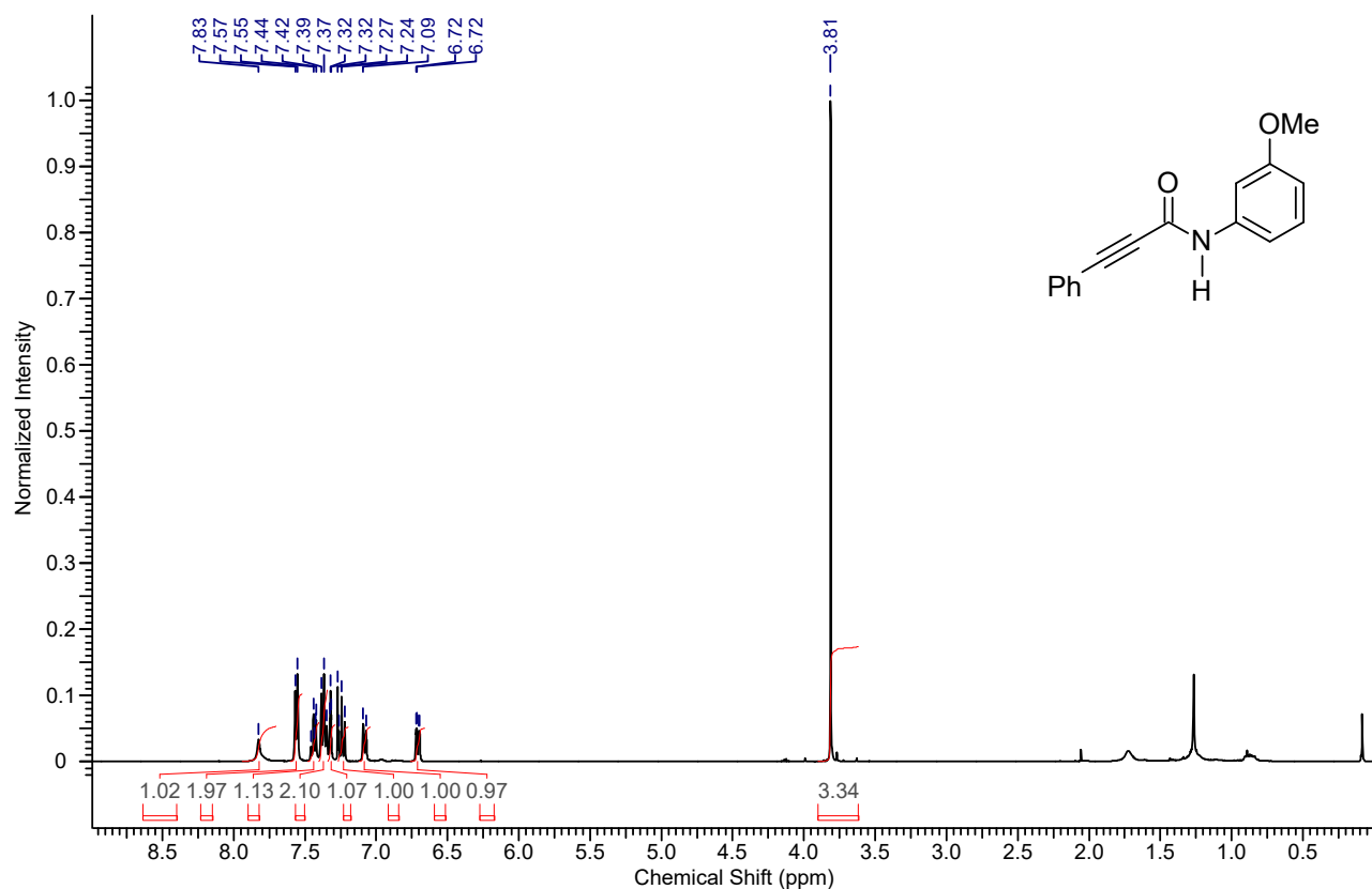
1 H NMR spectrum of the compound 4al
