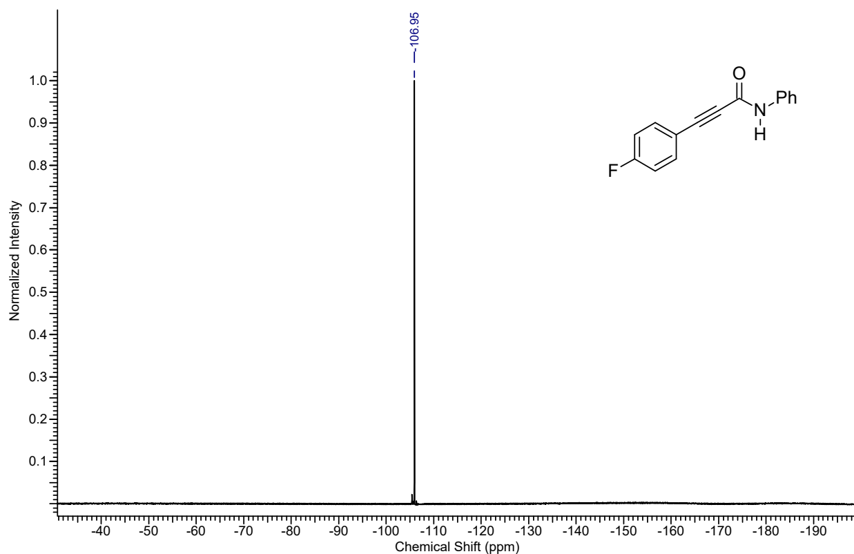
19 F NMR spectrum of the compound 4ea
