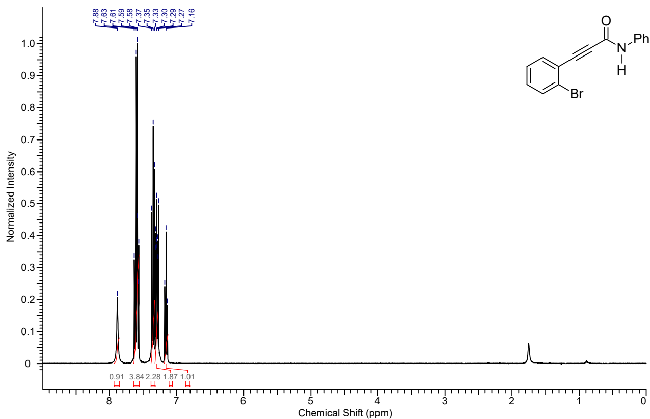
1 H NMR spectrum of the compound 4pa
