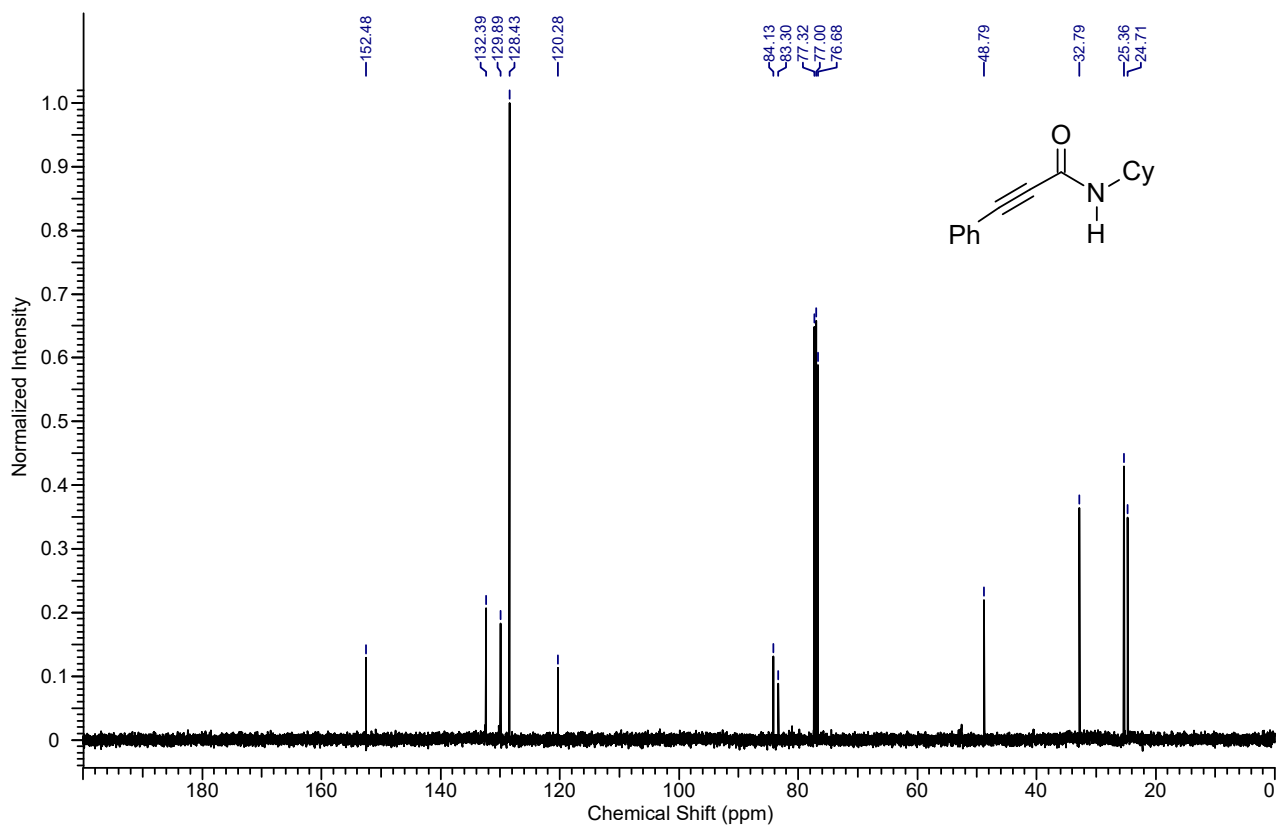
13 C NMR spectrum of the compound 4ar
