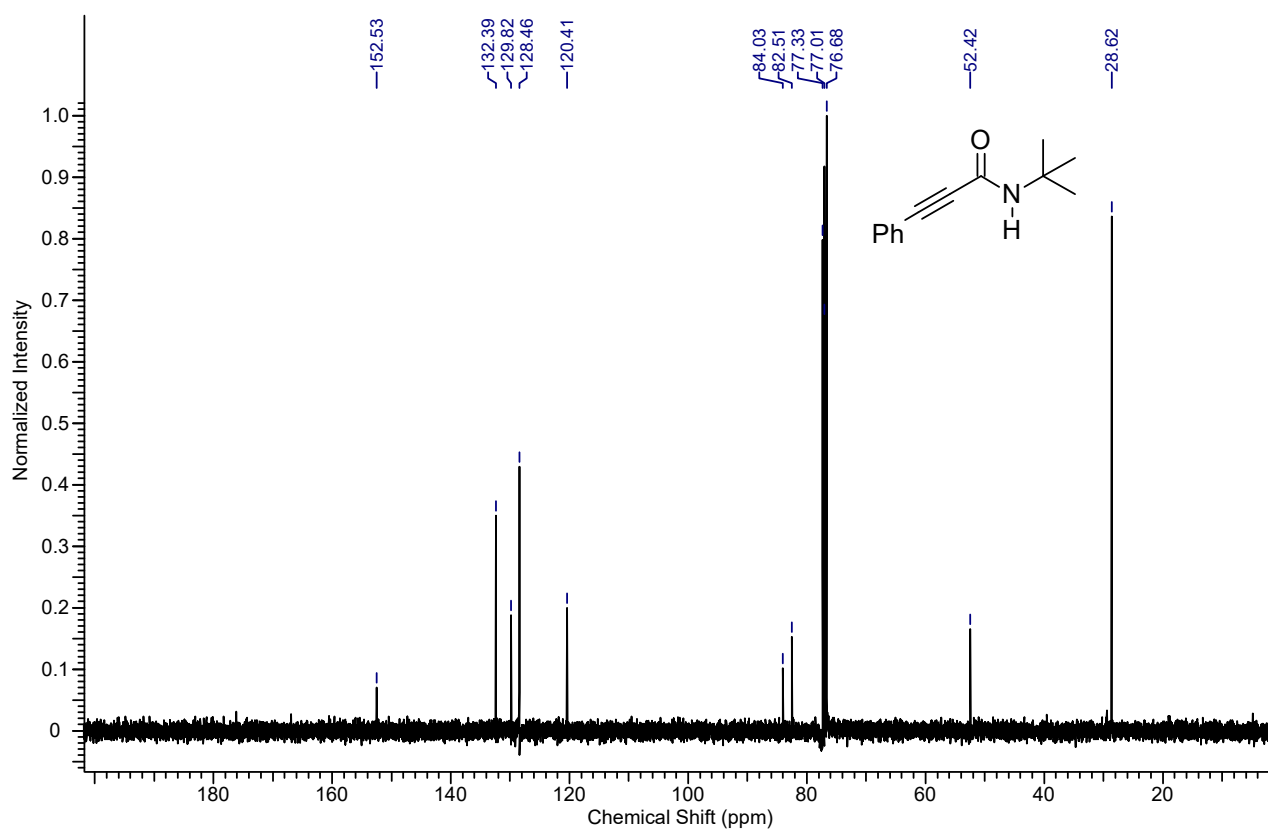
13 C NMR spectrum of the compound 4as
