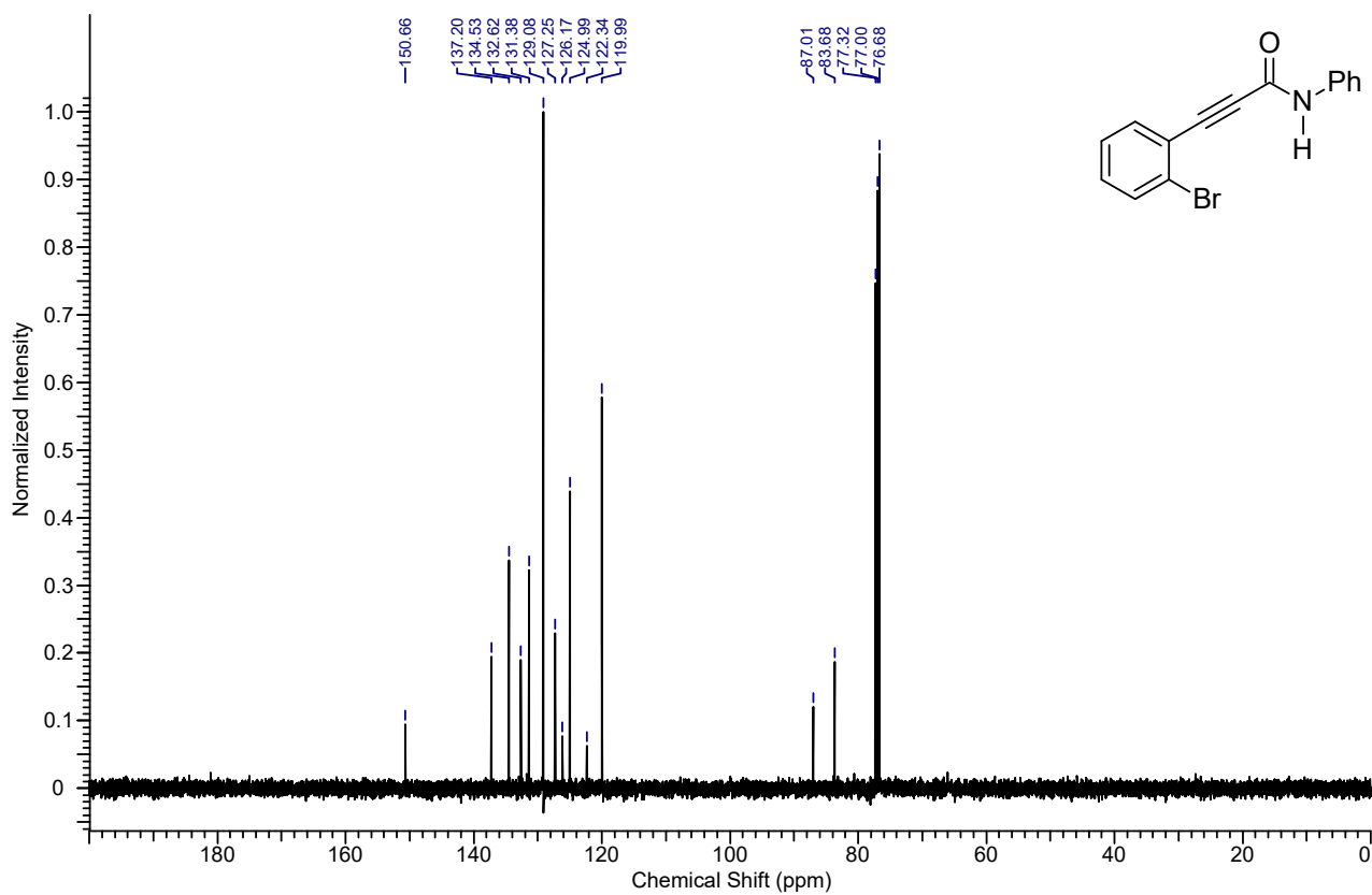
13 C NMR spectrum of the compound 4pa
