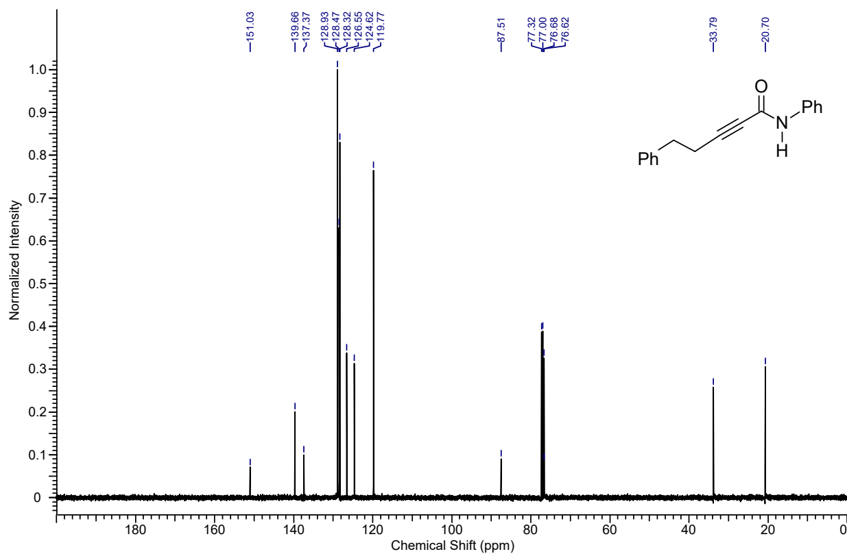
13 C NMR spectrum of the compound 7d
