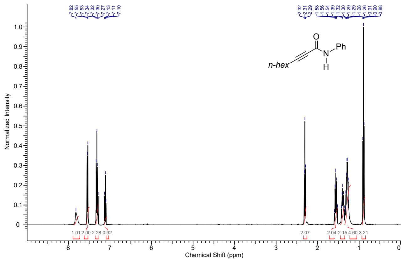
1 H NMR spectrum of the compound 7a
