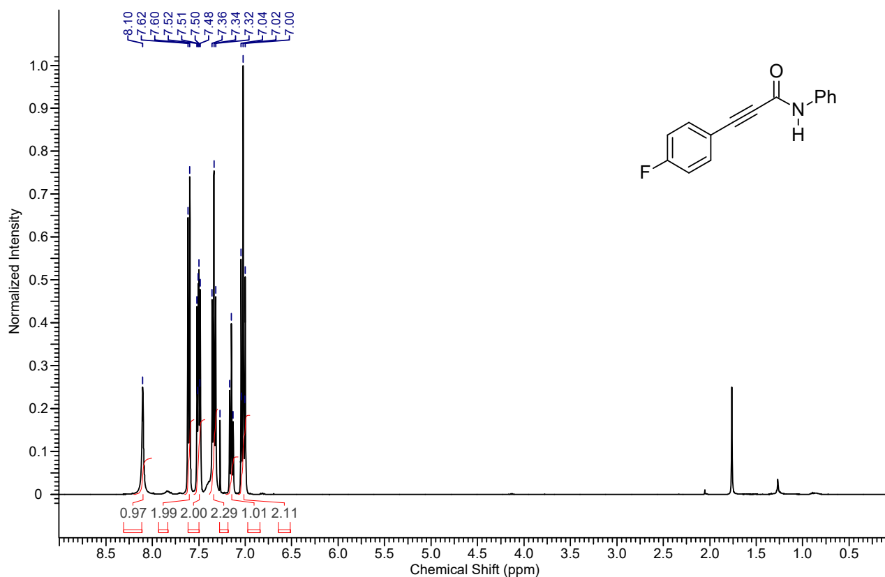
1 H NMR spectrum of the compound 4ea
