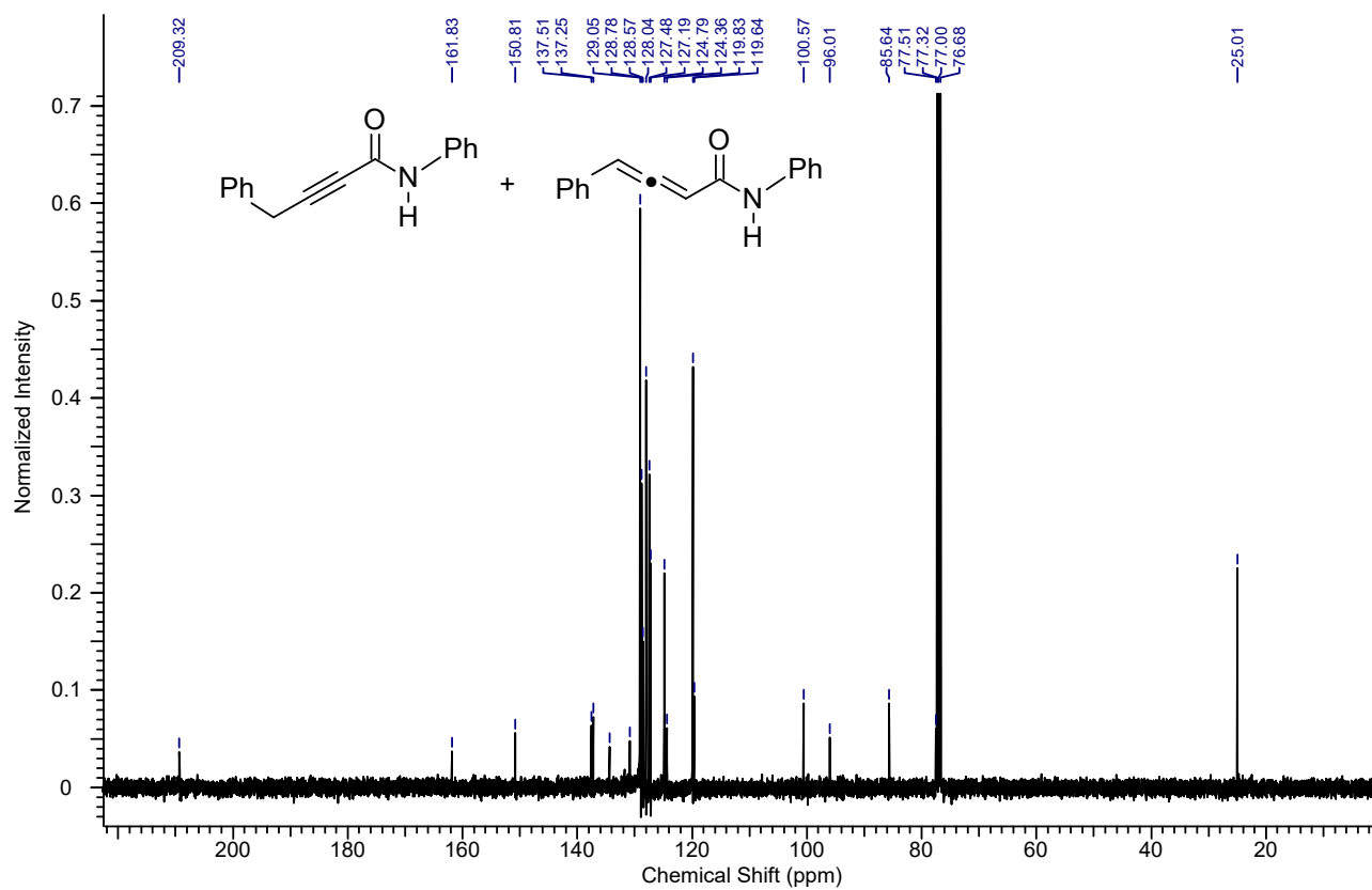
13 C NMR spectrum of the compound 7e (a 2:1 mixture of 7e and 7ea )
