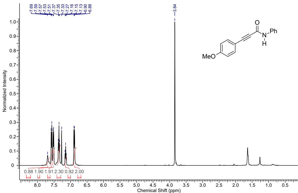
1 H NMR spectrum of the compound 4ba
