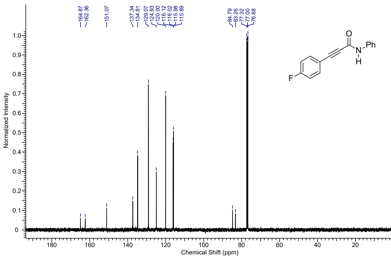
13 C NMR spectrum of the compound 4ea
