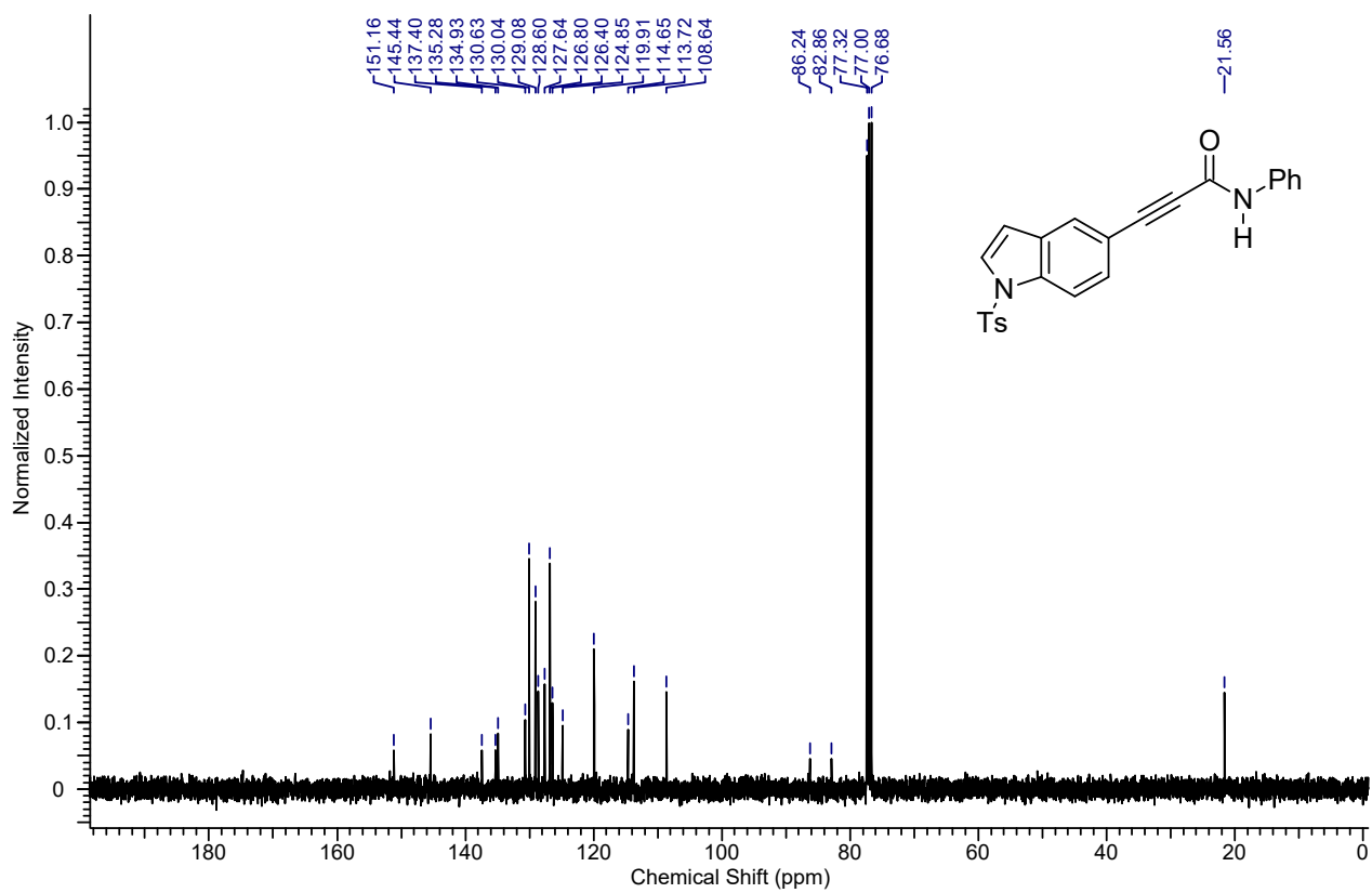
13 C NMR spectrum of the compound 4ua
