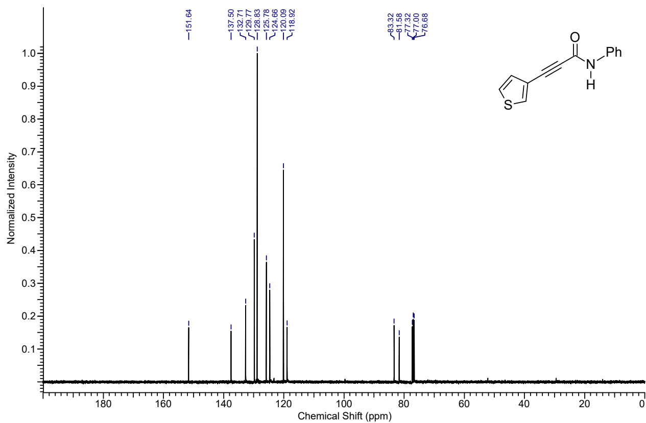
13 C NMR spectrum of the compound 4sa
