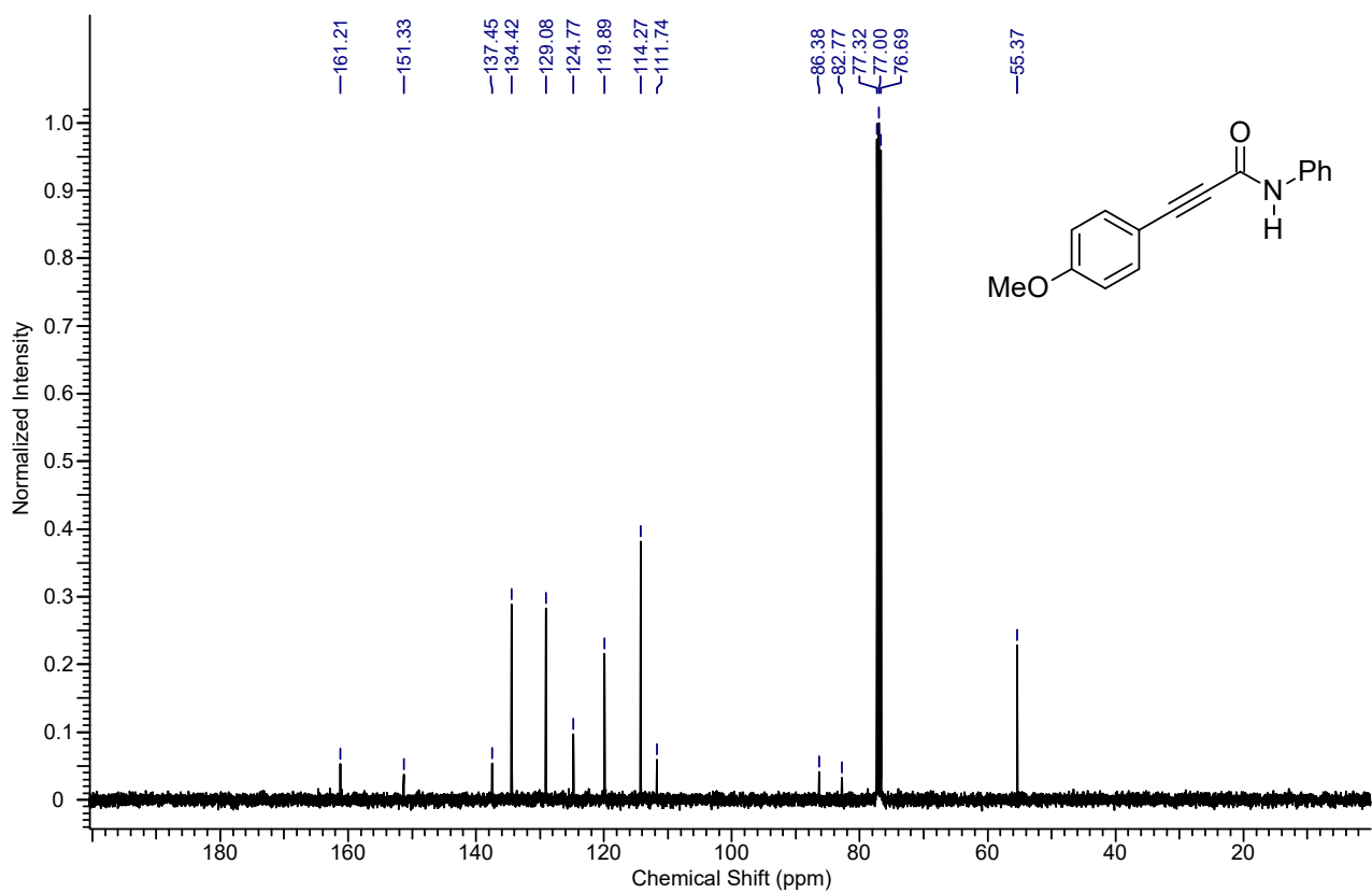
13 C NMR spectrum of the compound 4ba
