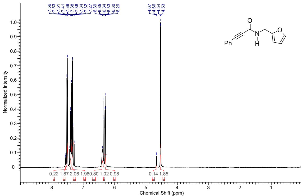
1 H NMR spectrum of the compound 4aq (a 9:1 mixture of rotamers)
