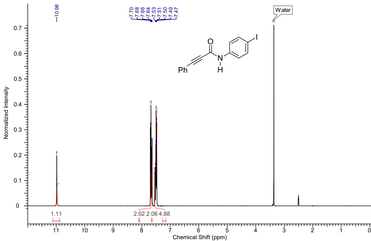
1 H NMR spectrum of the compound 4ae
