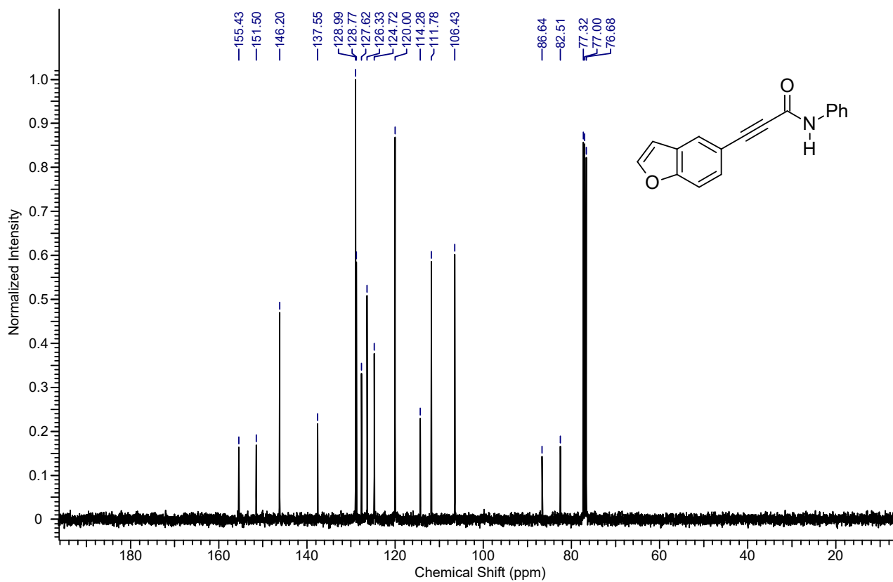
13 C NMR spectrum of the compound 4ta
