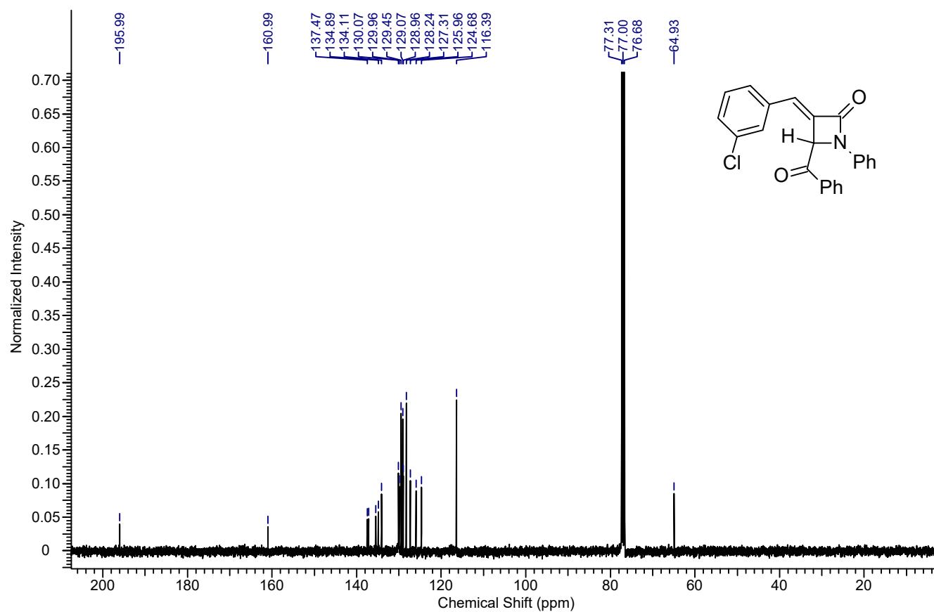
^{13}\text{C} NMR spectrum of the compound 9c
