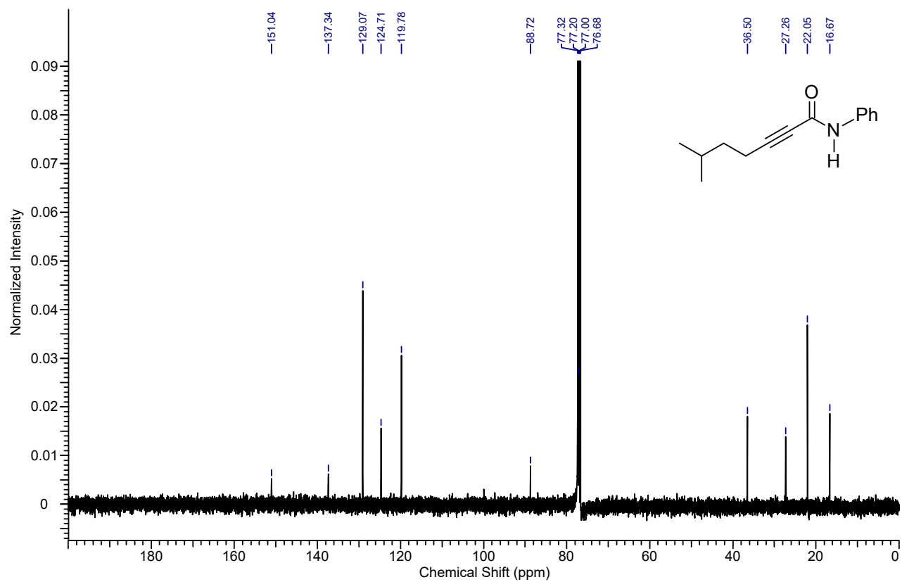
13 C NMR spectrum of the compound 7c
