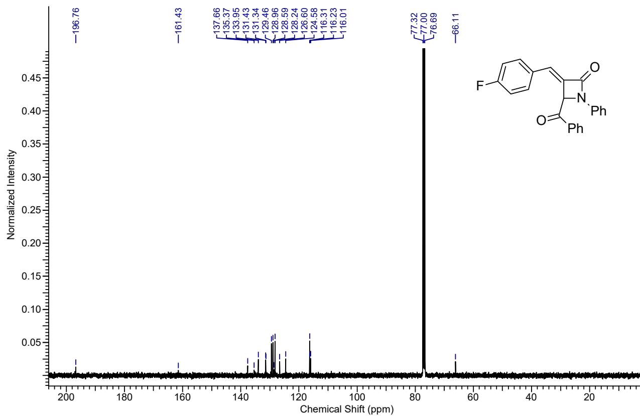
13 C NMR spectrum of the compound 9b
