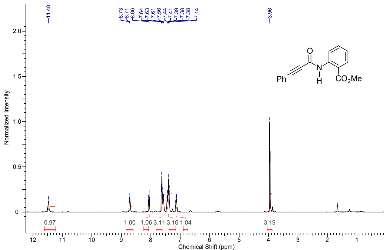
1 H NMR spectrum of the compound 4ak
