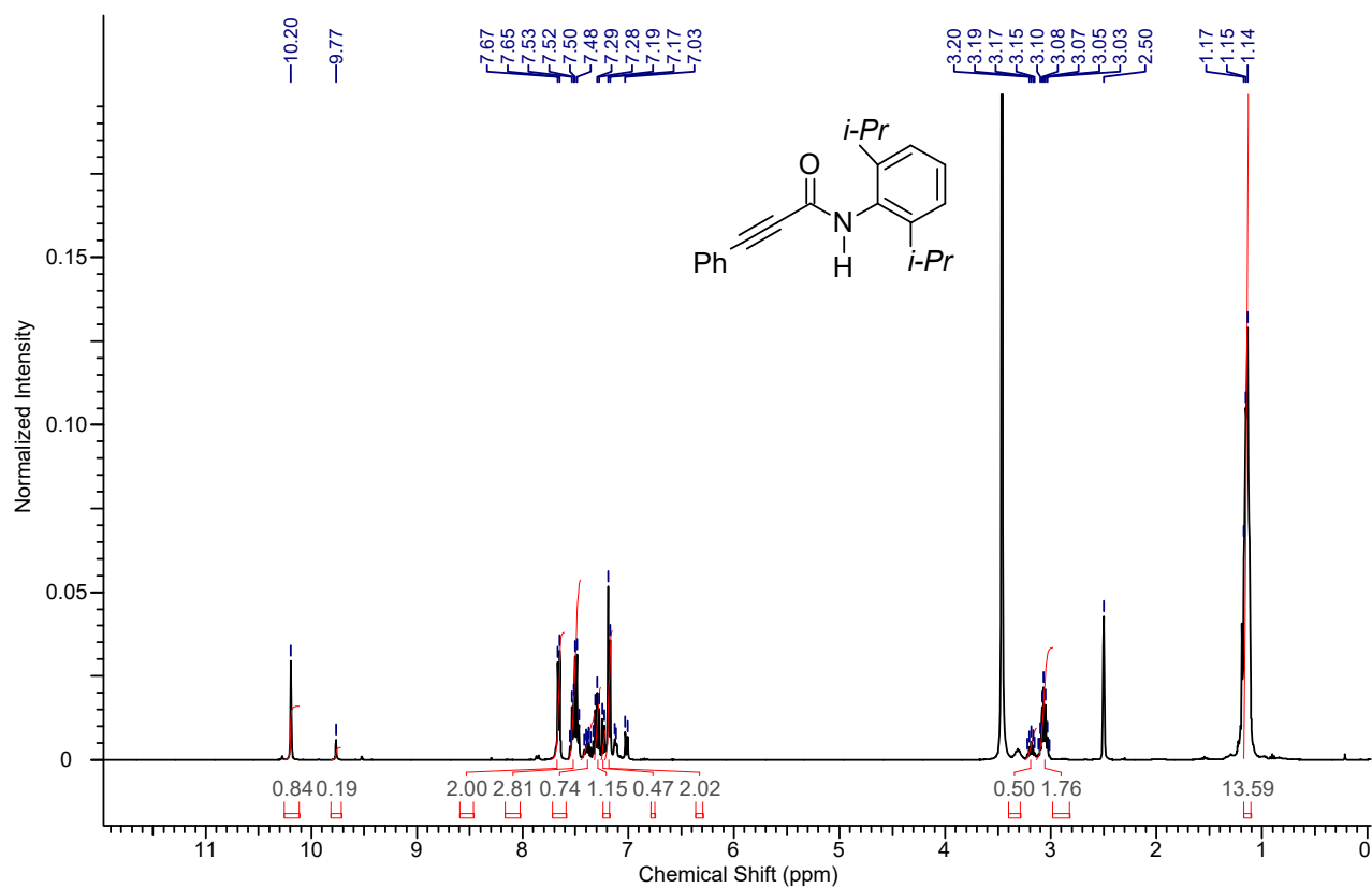
1 H NMR spectrum of the compound 4an (a 4:1 mixture of rotamers)
