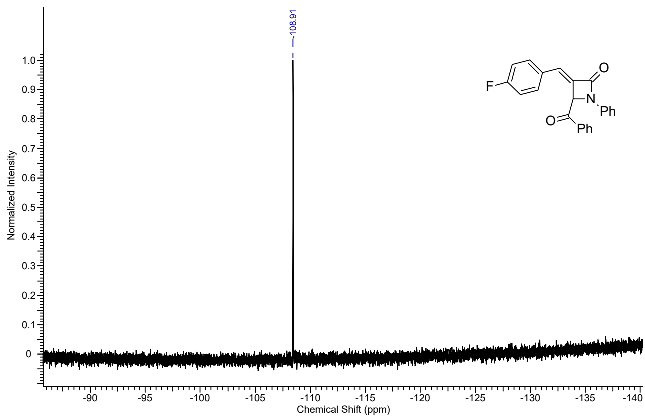
19 F NMR spectrum of the compound 9b
