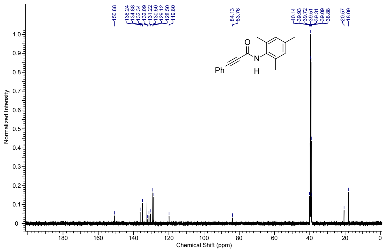
13 C NMR spectrum of the compound 4am (a 9:1 mixture of rotamers)
