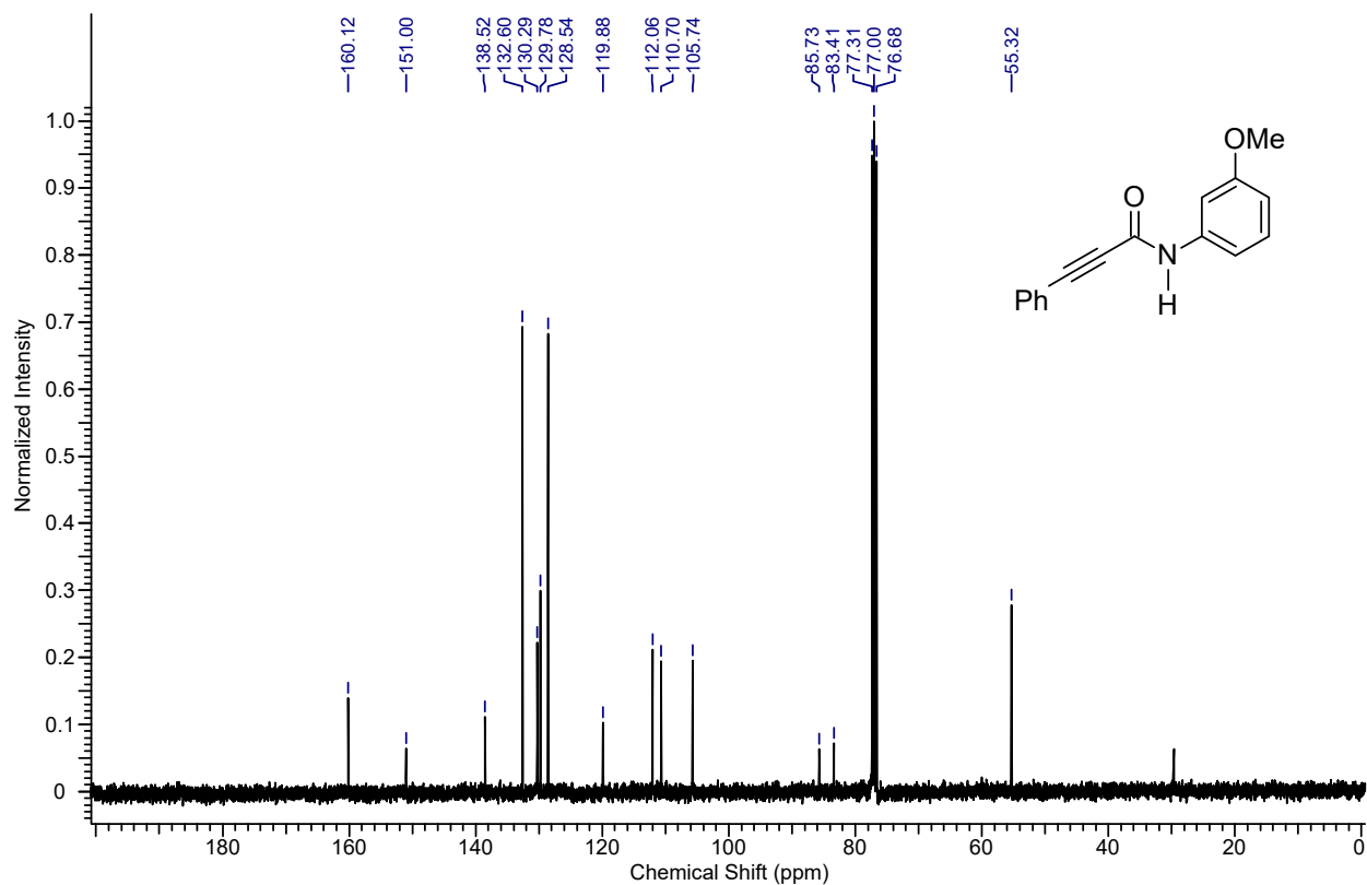
13 C NMR spectrum of the compound 4al
