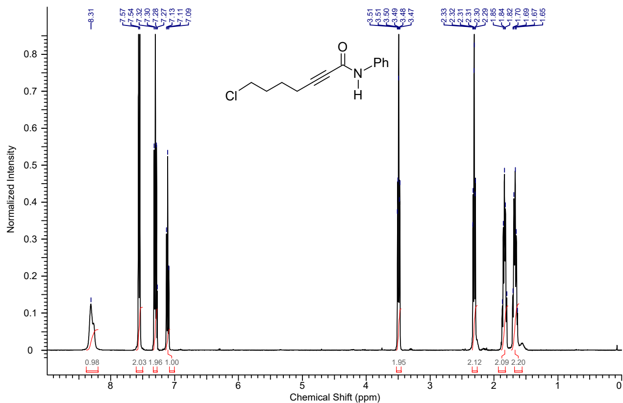
^1\text{H} NMR spectrum of the compound 7j
