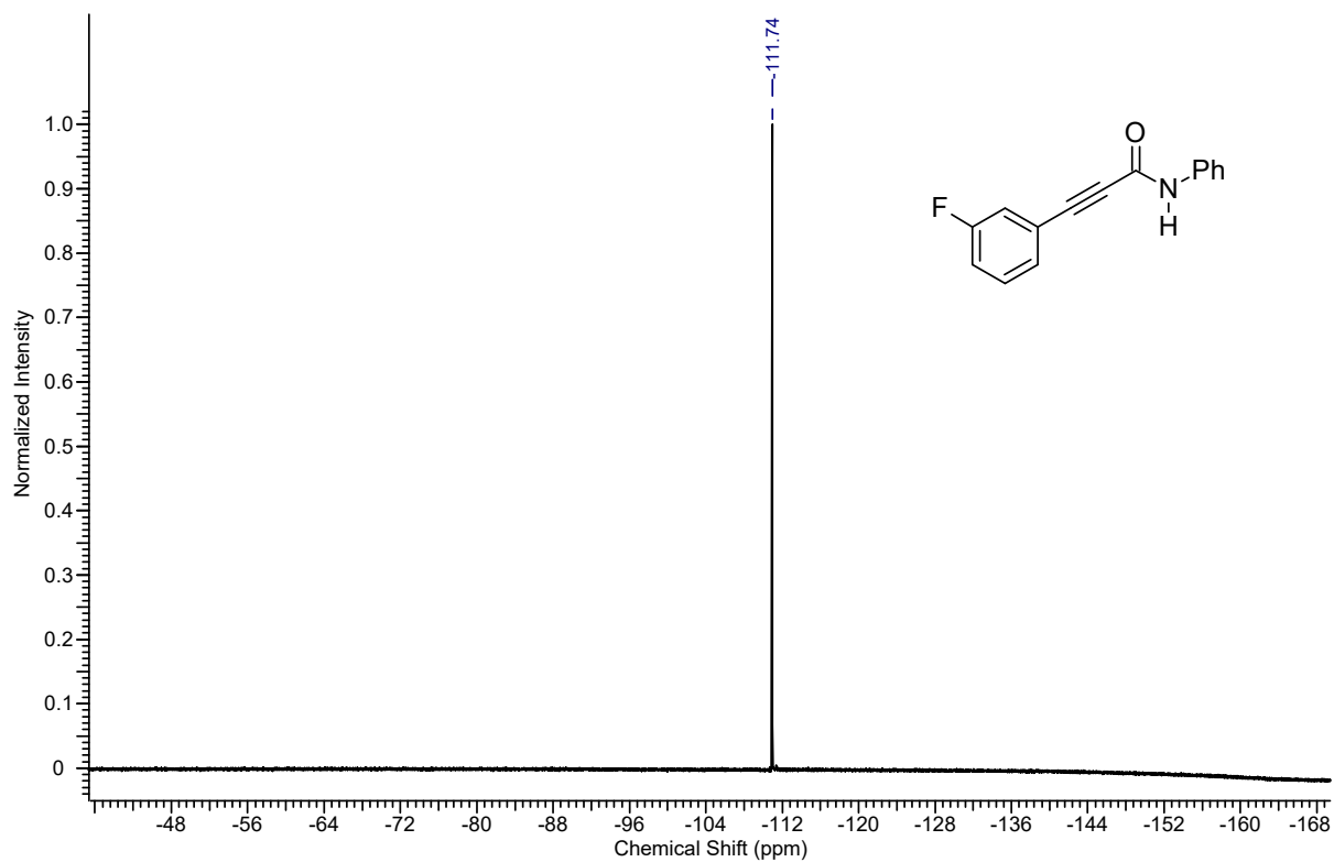
19 F NMR spectrum of the compound 4a
