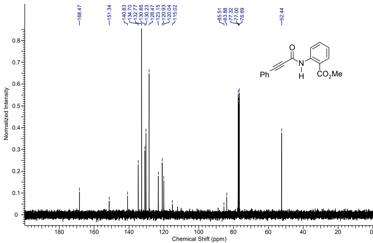
13 C NMR spectrum of the compound 4ak
