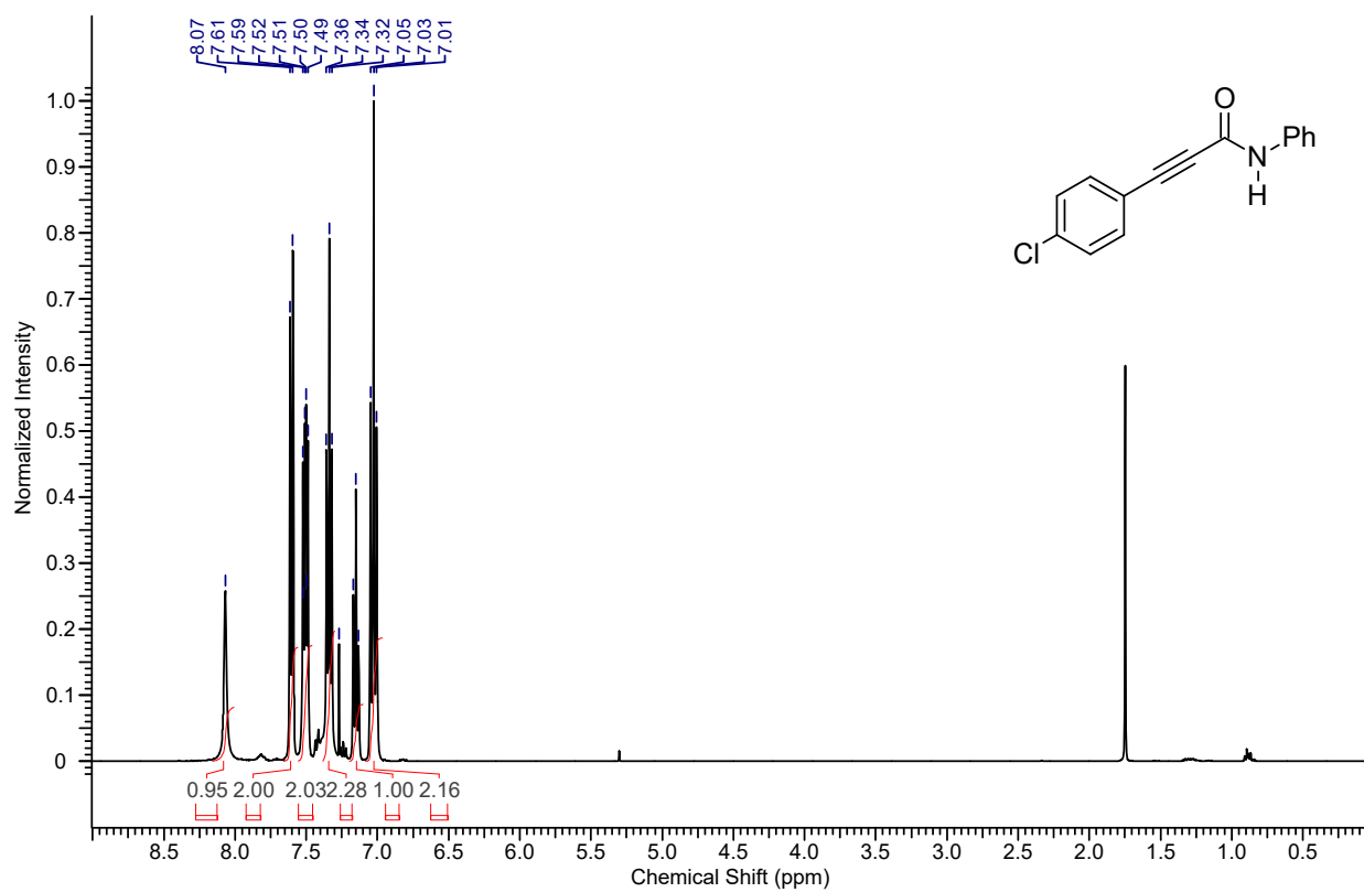
1 H NMR spectrum of the compound 4fa
