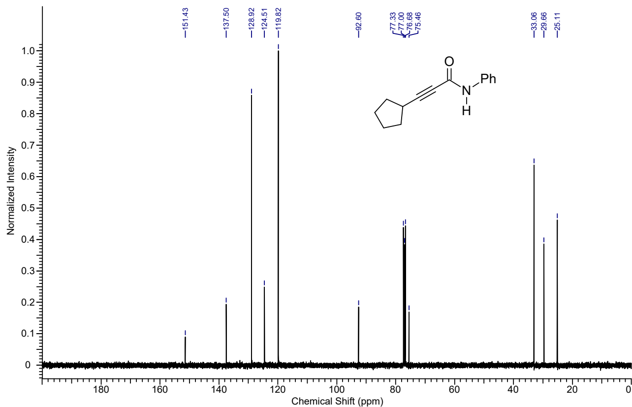
13 C NMR spectrum of the compound 7h
