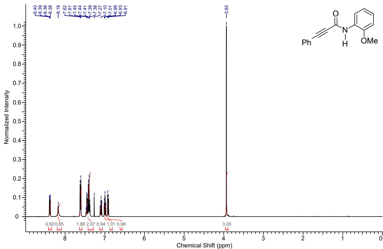
1 H NMR spectrum of the compound 4aj
