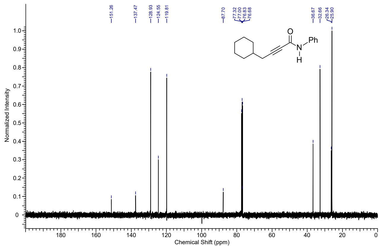
13 C NMR spectrum of the compound 7f
