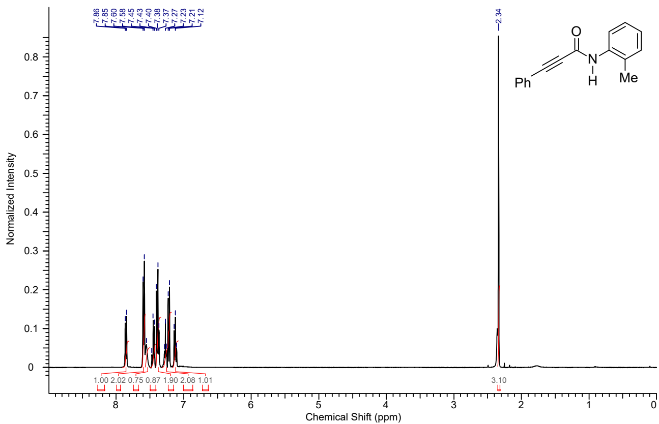
1 H NMR spectrum of the compound 4ai
