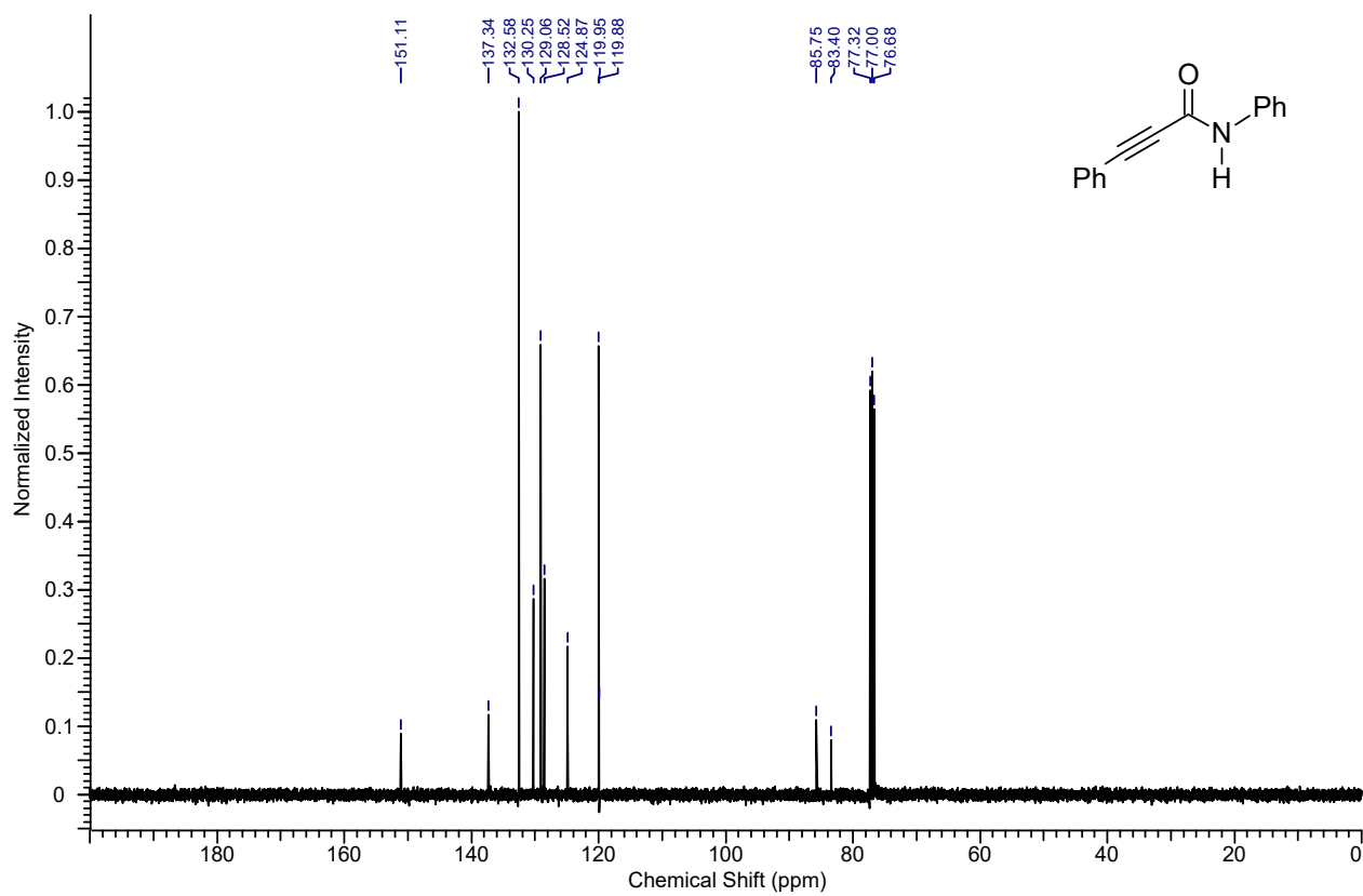
13 C NMR spectrum of the compound 4aa
