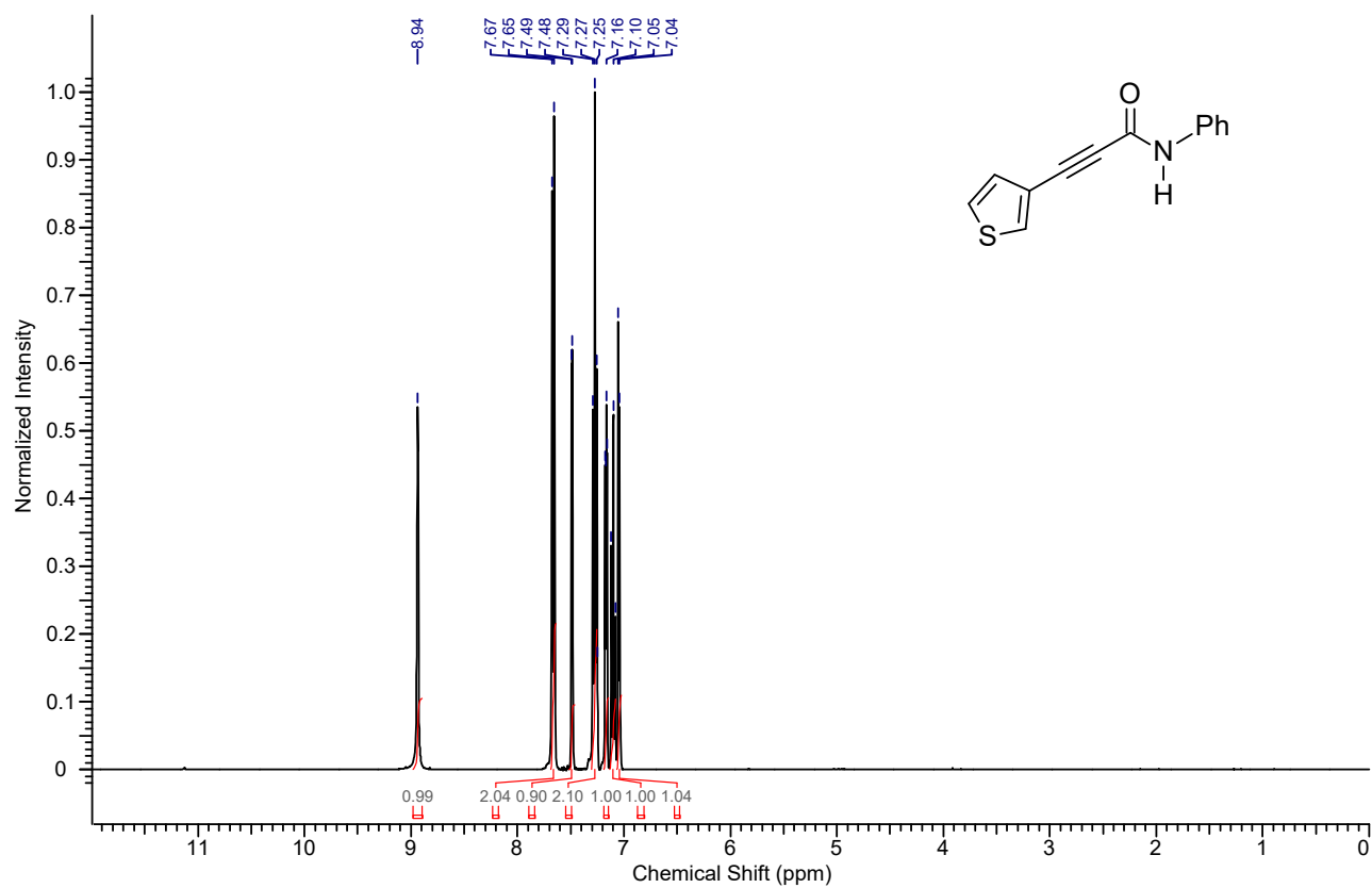
1 H NMR spectrum of the compound 4sa
