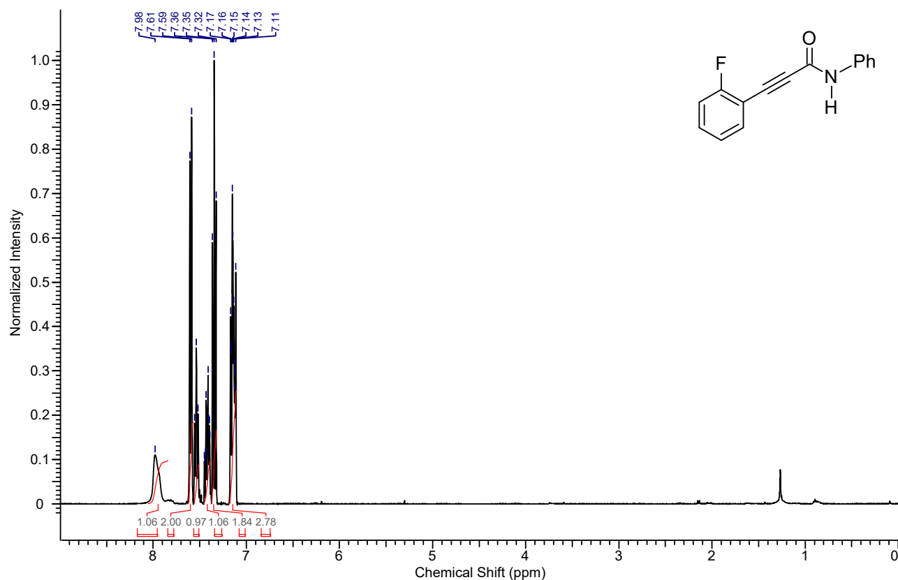
1 H NMR spectrum of the compound 4na
