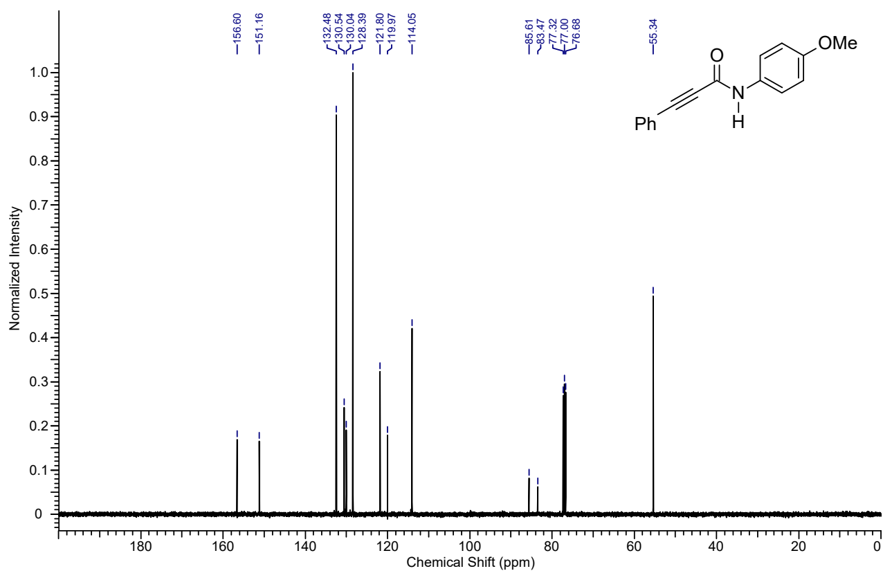
13 C NMR spectrum of the compound 4ab
