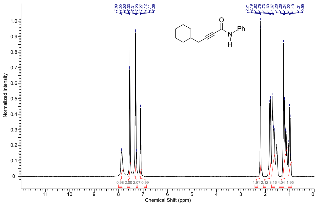
1 H NMR spectrum of the compound 7f
