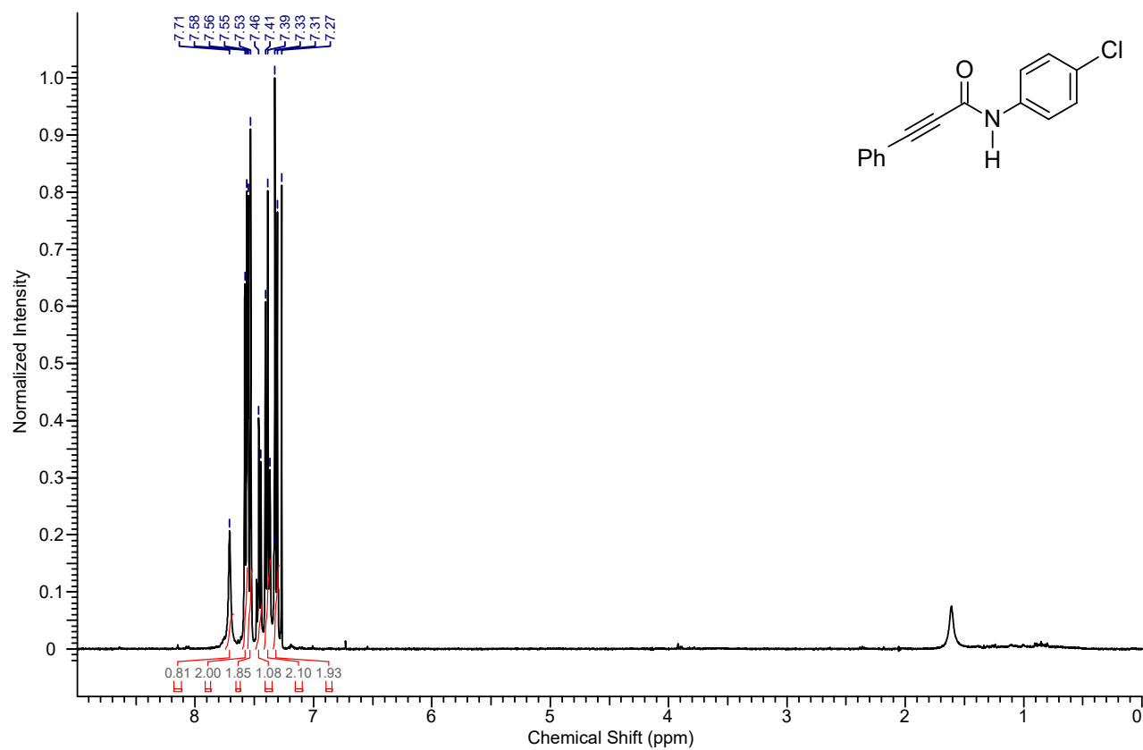
1 H NMR spectrum of the compound 4ac
