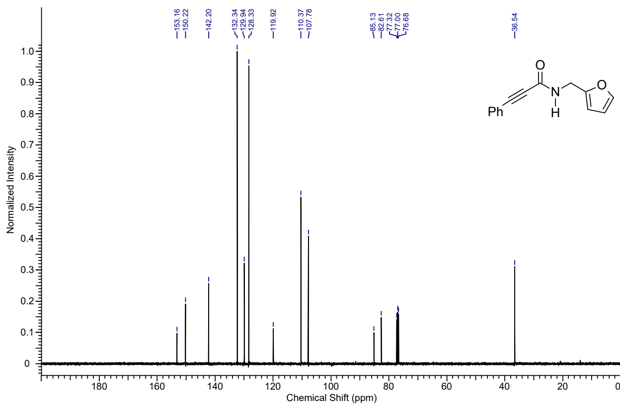
13 C NMR spectrum of the compound 4aq
