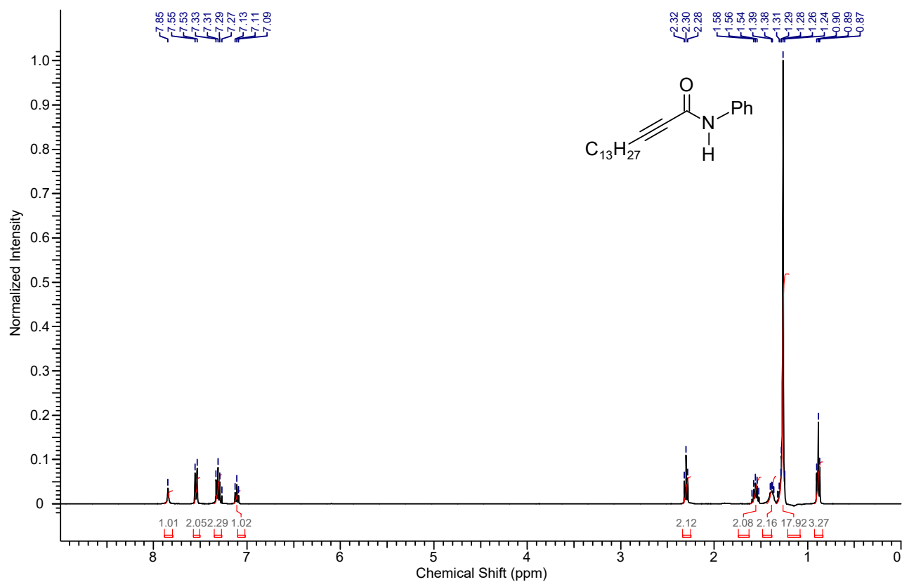
1 H NMR spectrum of the compound 7b
