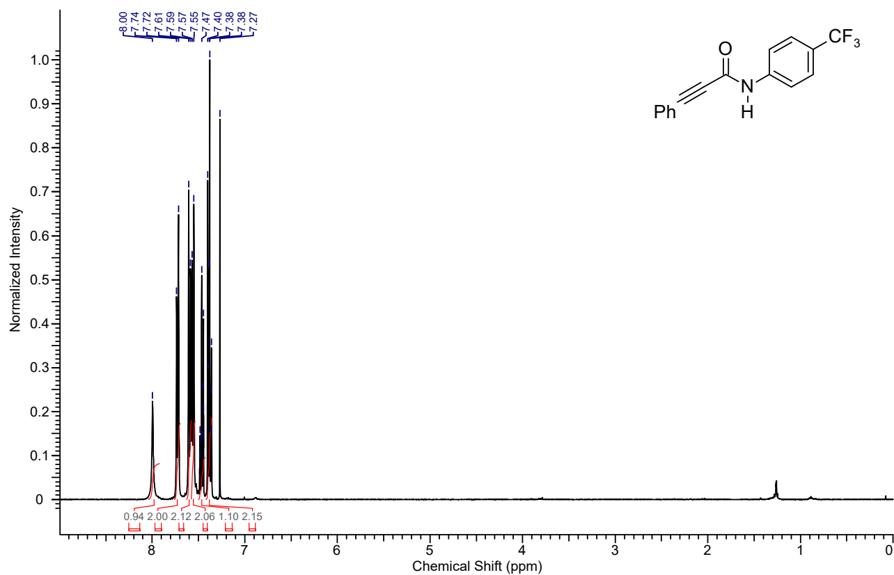
1 H NMR spectrum of the compound 4ag
