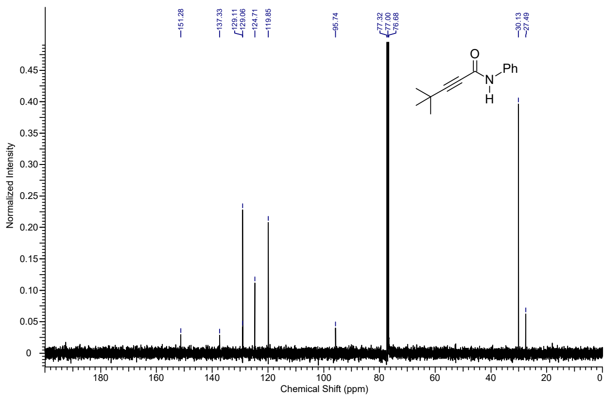
13 C NMR spectrum of the compound 7i
