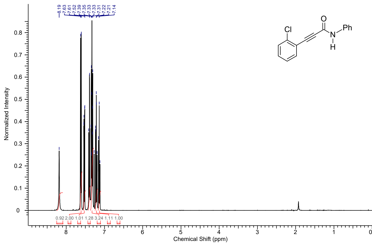
1 H NMR spectrum of the compound 40a
