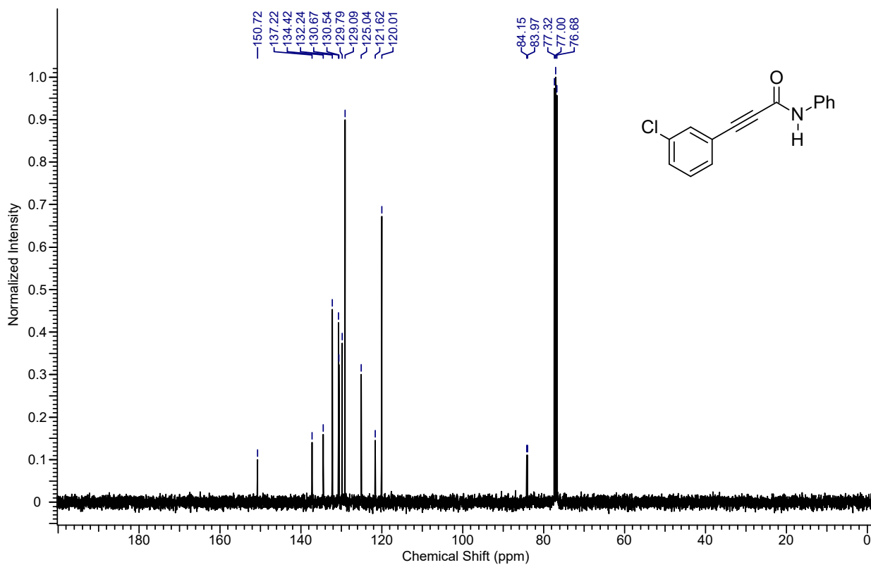
13 C NMR spectrum of the compound 4ma
