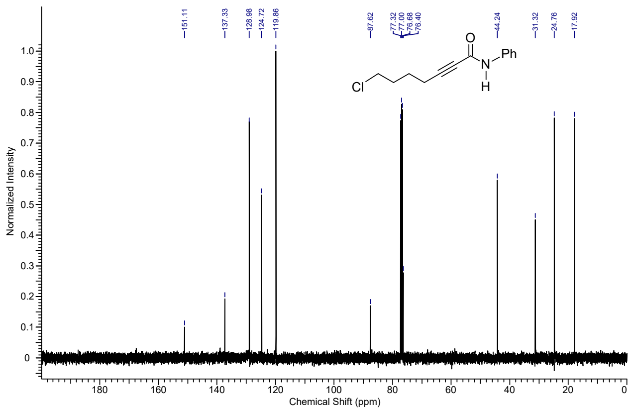
^{13}\text{C} NMR spectrum of the compound 7j
