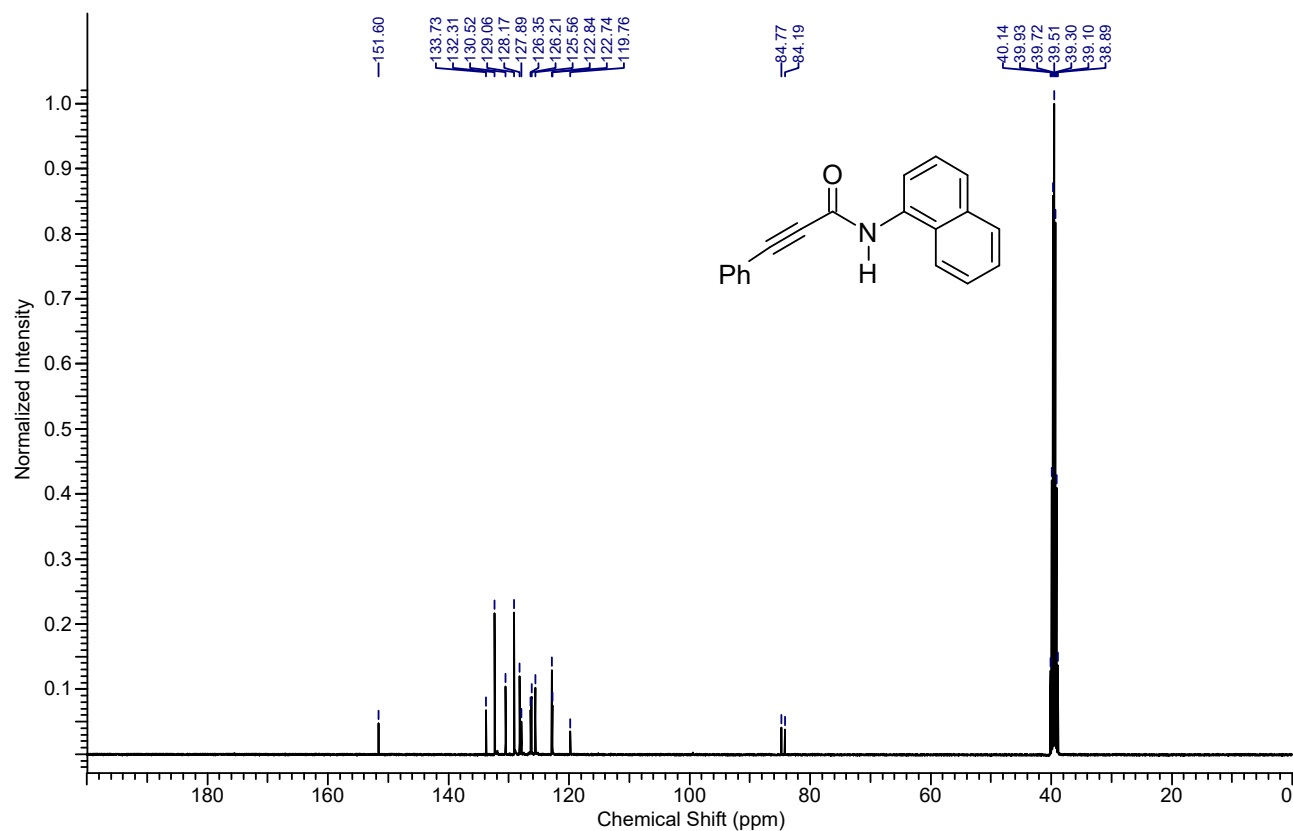
13 C NMR spectrum of the compound 4ao
