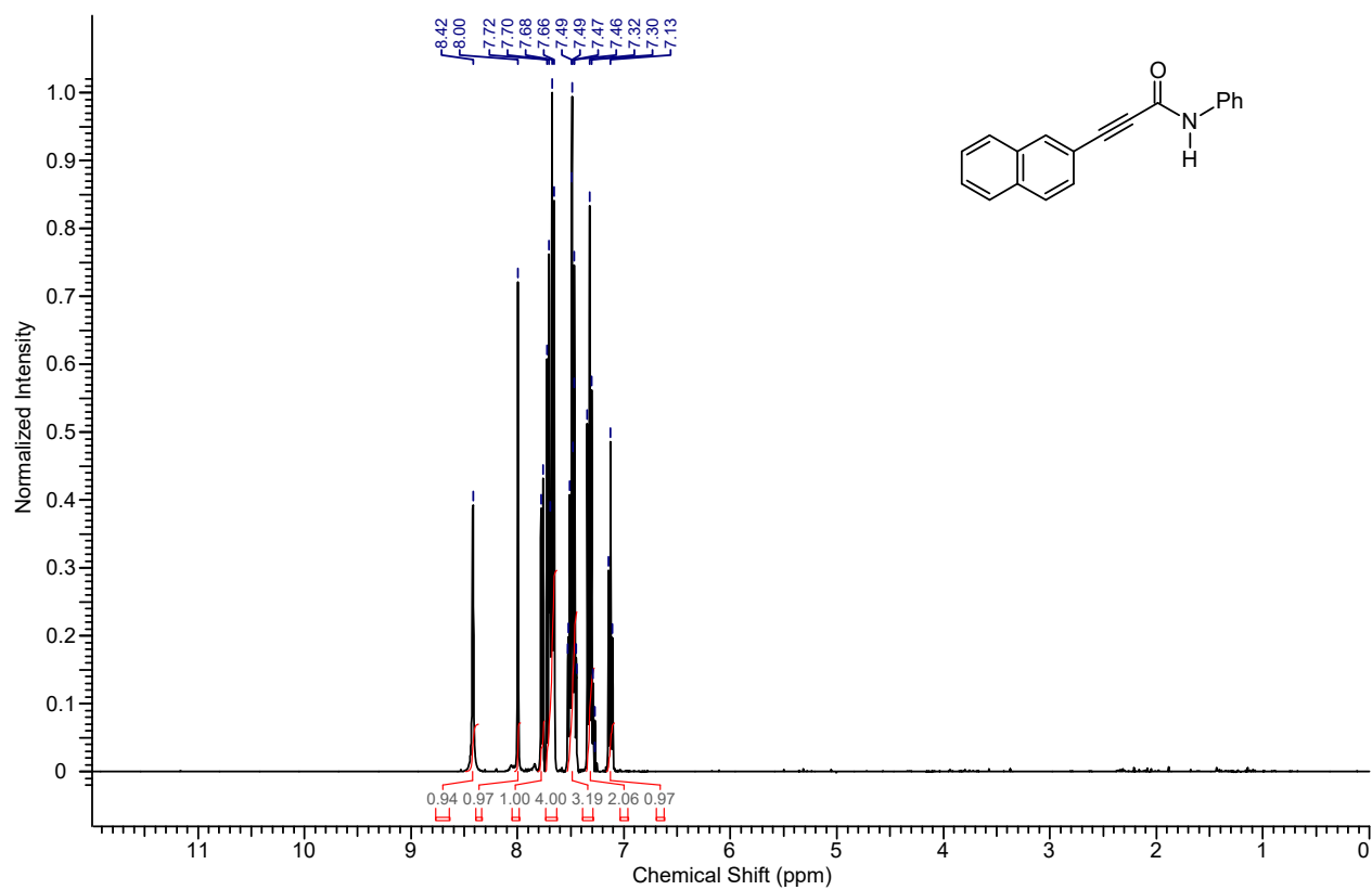
1 H NMR spectrum of the compound 4ra
