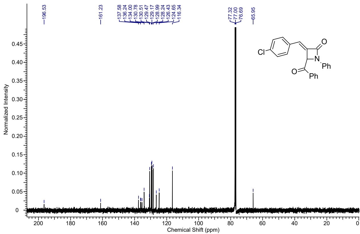
13 C NMR spectrum of the compound 9a
