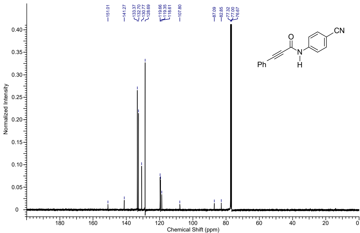
13 C NMR spectrum of the compound 4af
