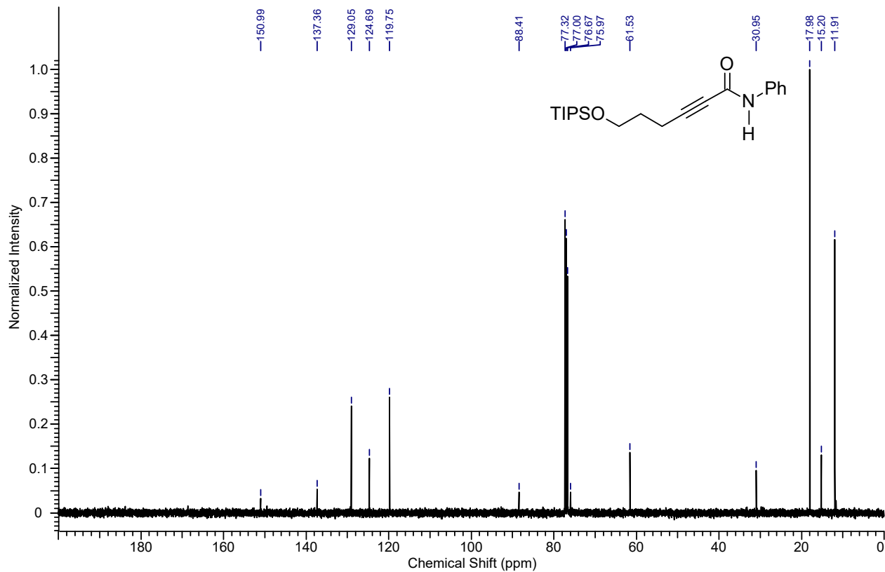
13 C NMR spectrum of the compound 7k
