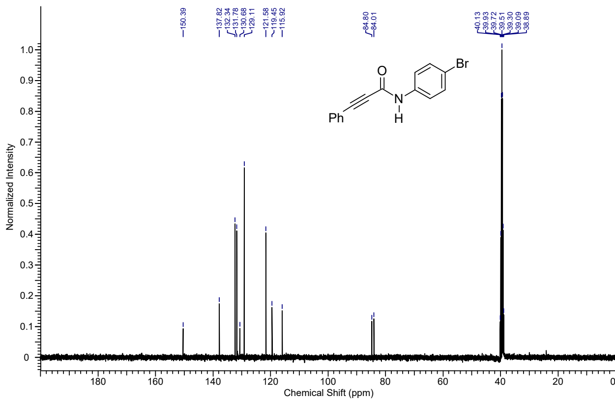
13 C NMR spectrum of the compound 4ad
