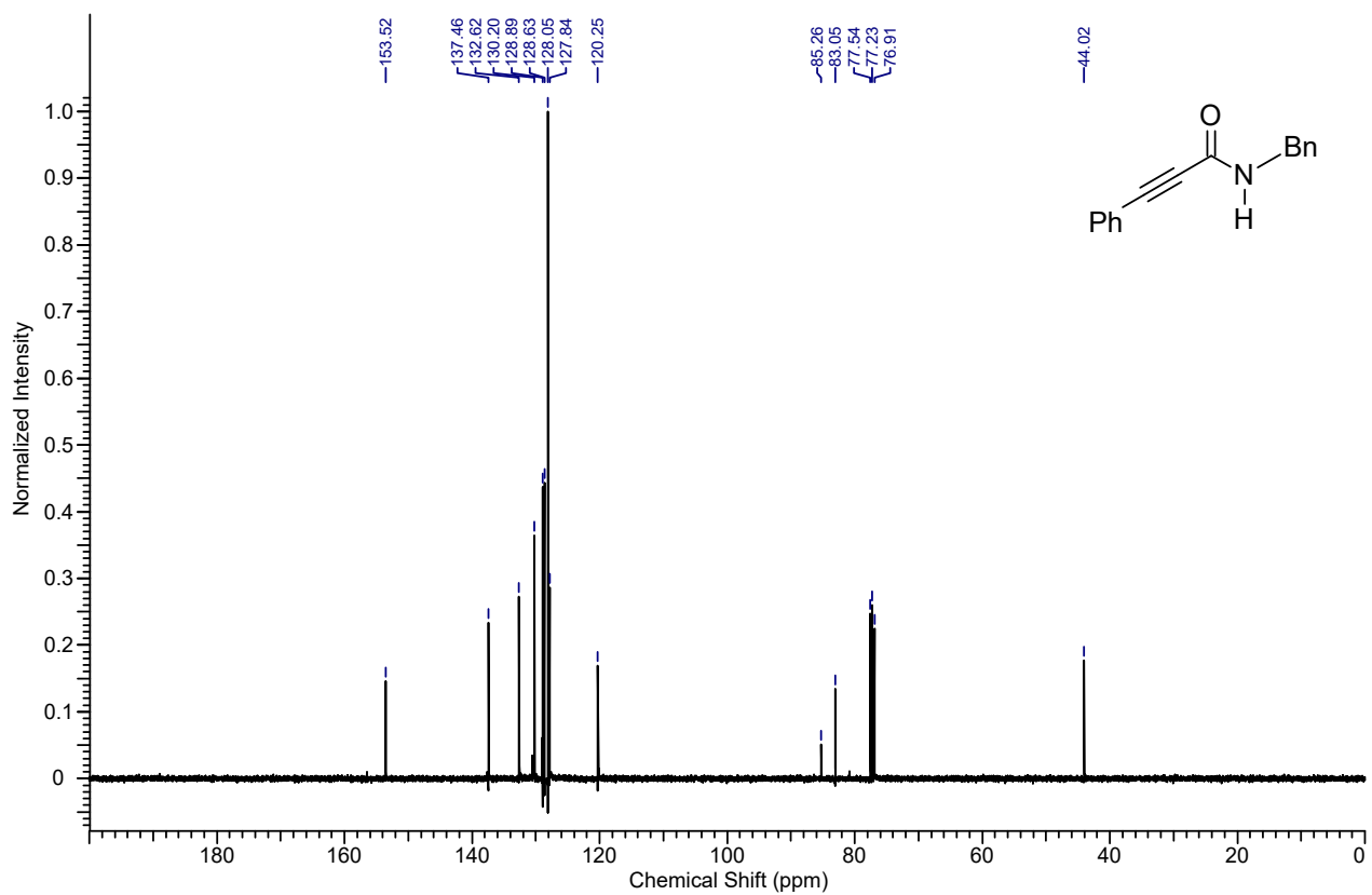
13 C NMR spectrum of the compound 4ap
