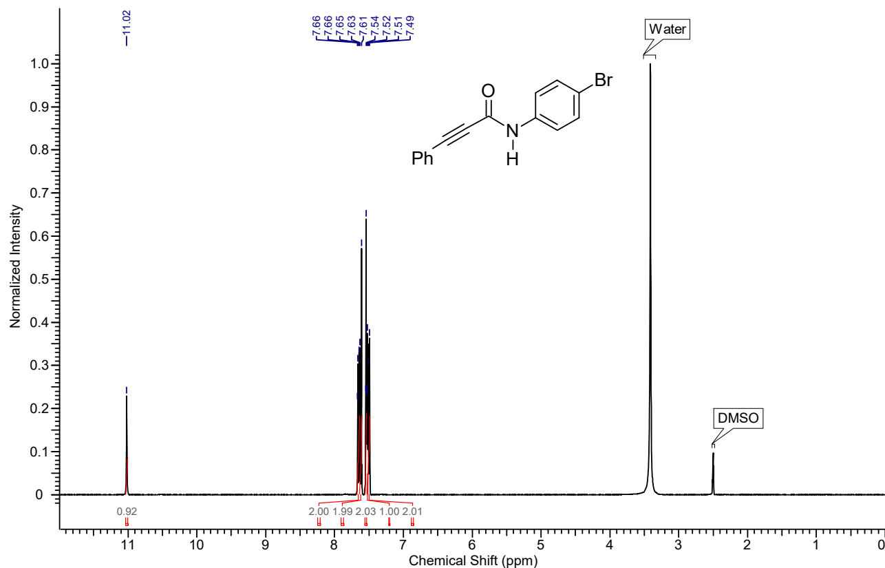
1 H NMR spectrum of the compound 4ad
