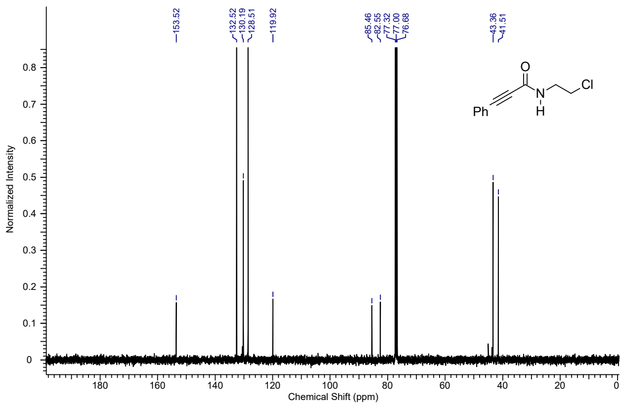
13 C NMR spectrum of the compound 4at
