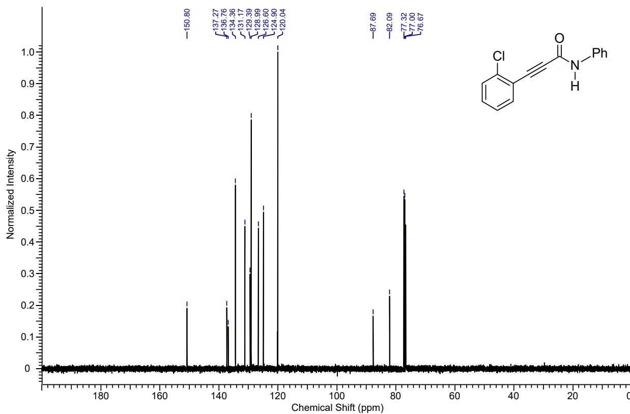
13 C NMR spectrum of the compound 40a
