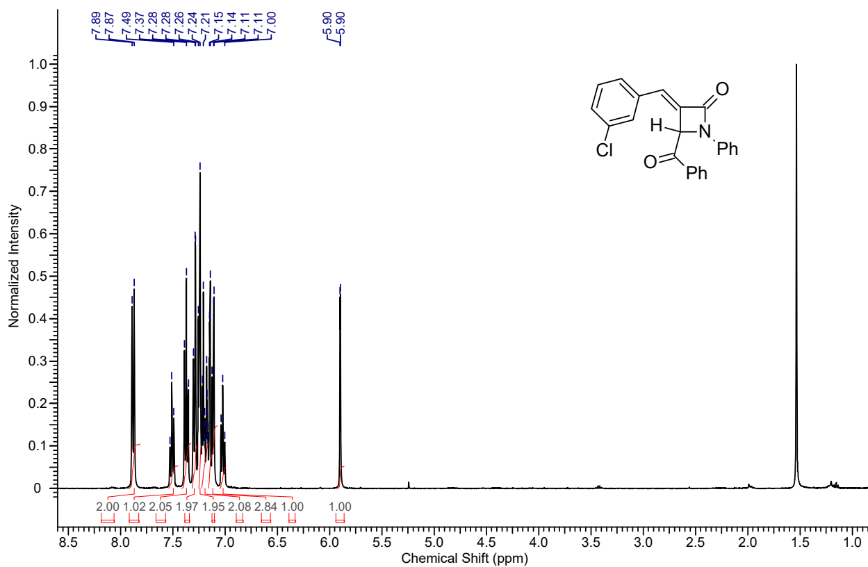
1 H NMR spectrum of the compound 9c
