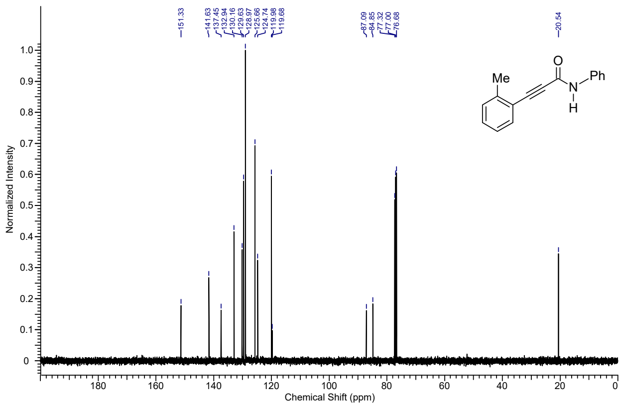
13 C NMR spectrum of the compound 4qa
