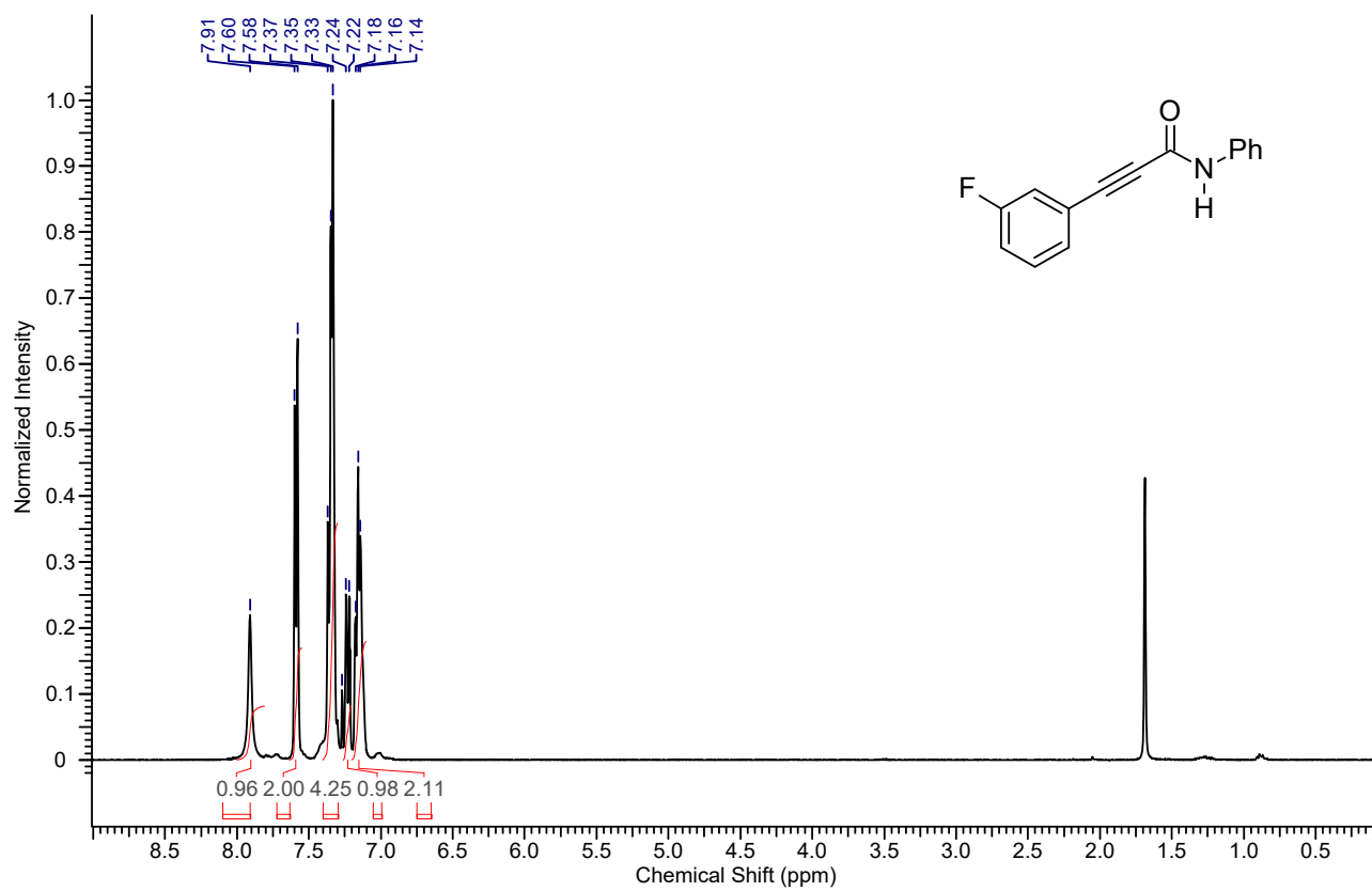
1 H NMR spectrum of the compound 4la
