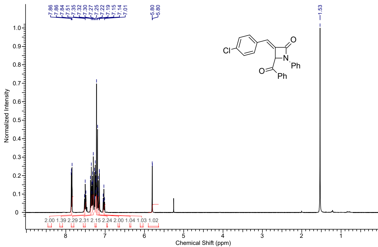
1 H NMR spectrum of the compound 9a
