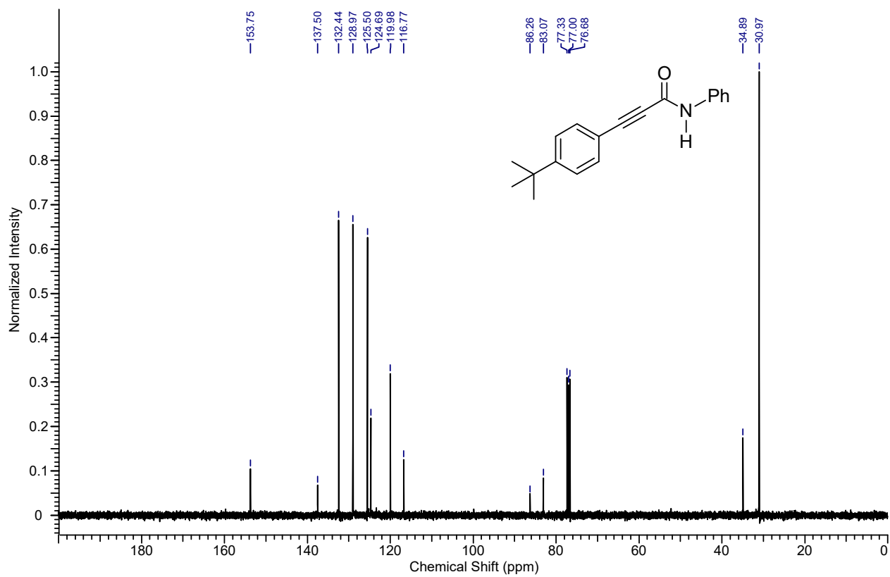
^{13}\text{C} NMR spectrum of the compound 4da
