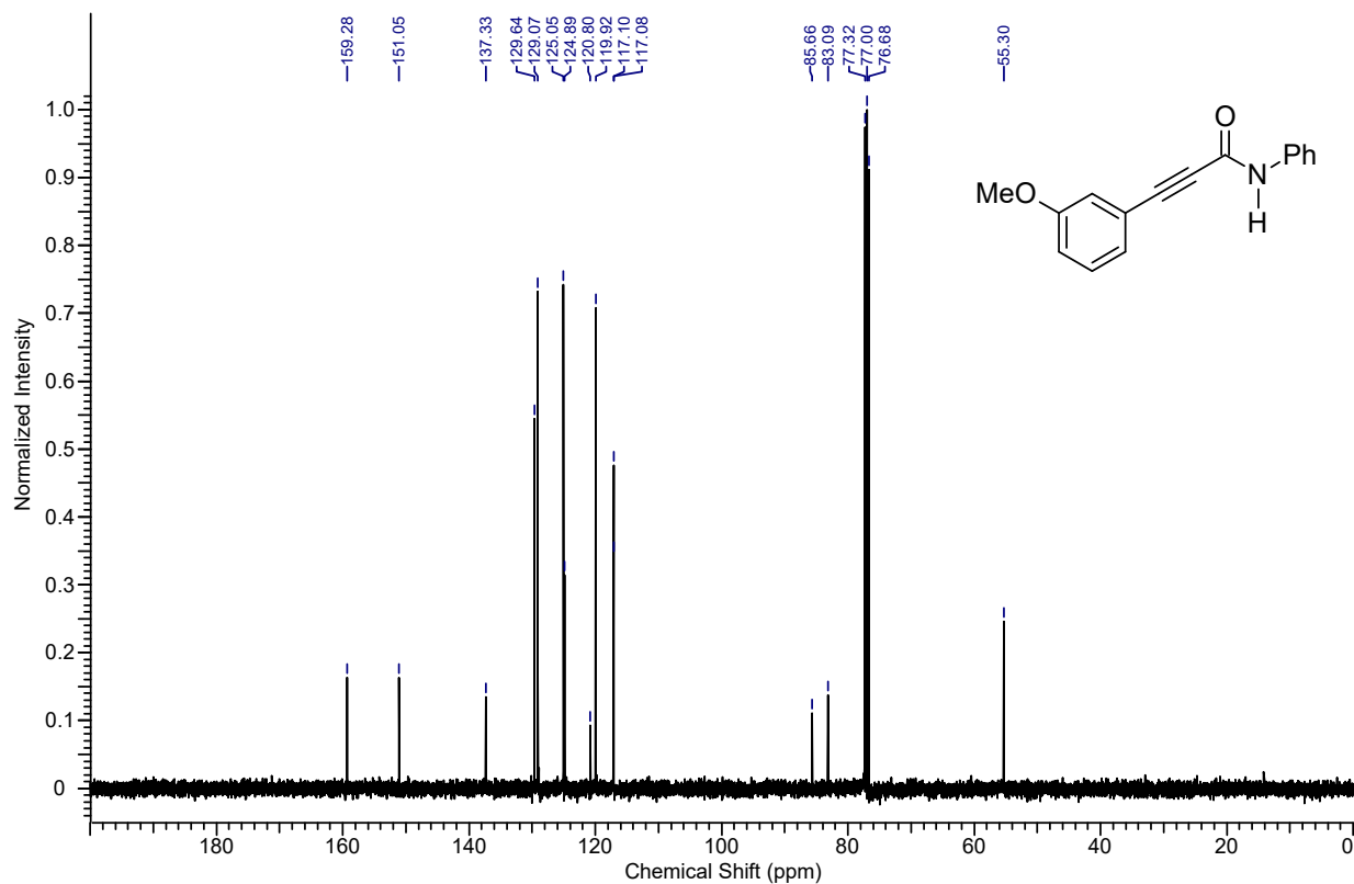
13 C NMR spectrum of the compound 4ka
