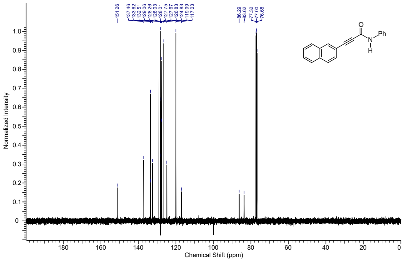
13 C NMR spectrum of the compound 4ra
