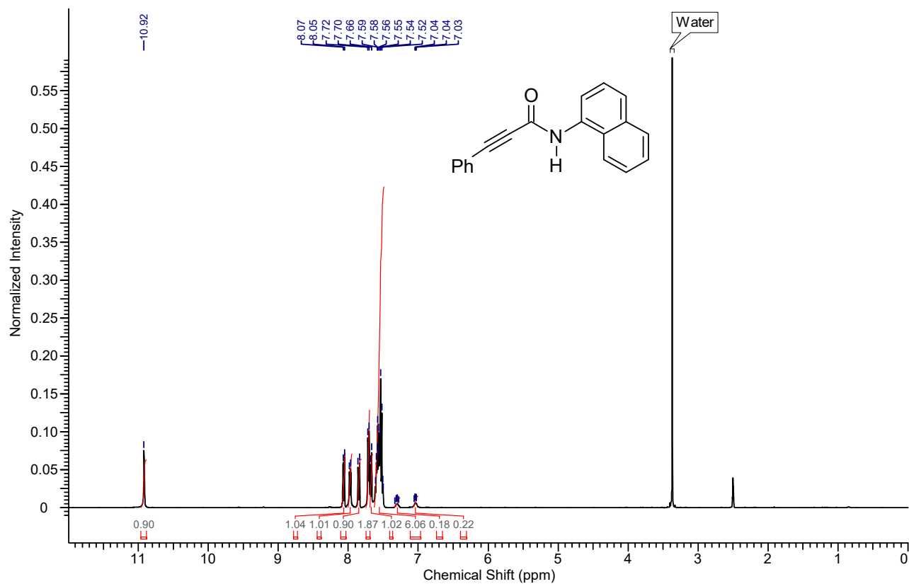
1 H NMR spectrum of the compound 4ao (a 5:1 mixture of rotamers)
