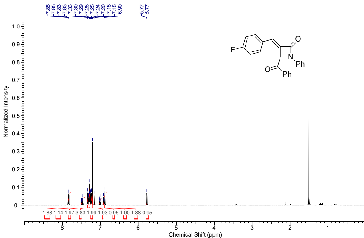
1 H NMR spectrum of the compound 9b
