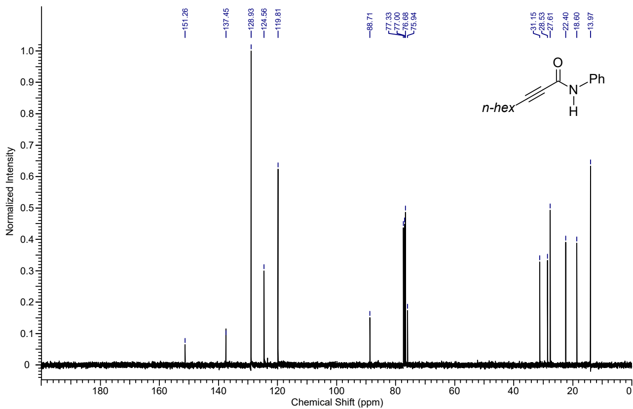
13 C NMR spectrum of the compound 7a
