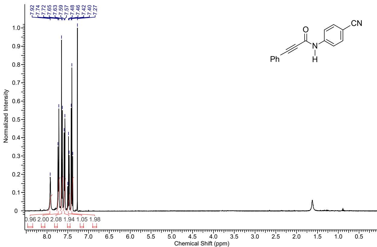
1 H NMR spectrum of the compound 4af
