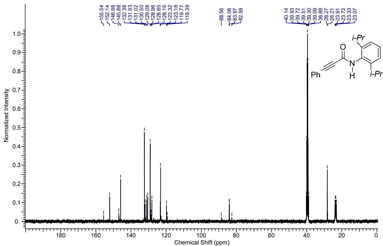
13 C NMR spectrum of the compound 4an (a 4:1 mixture of rotamers)
