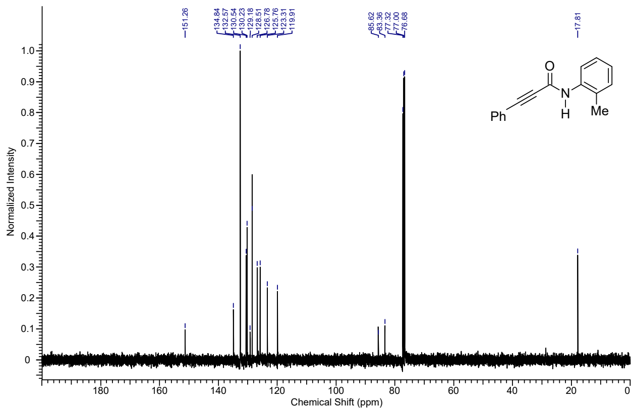
13 C NMR spectrum of the compound 4ai
