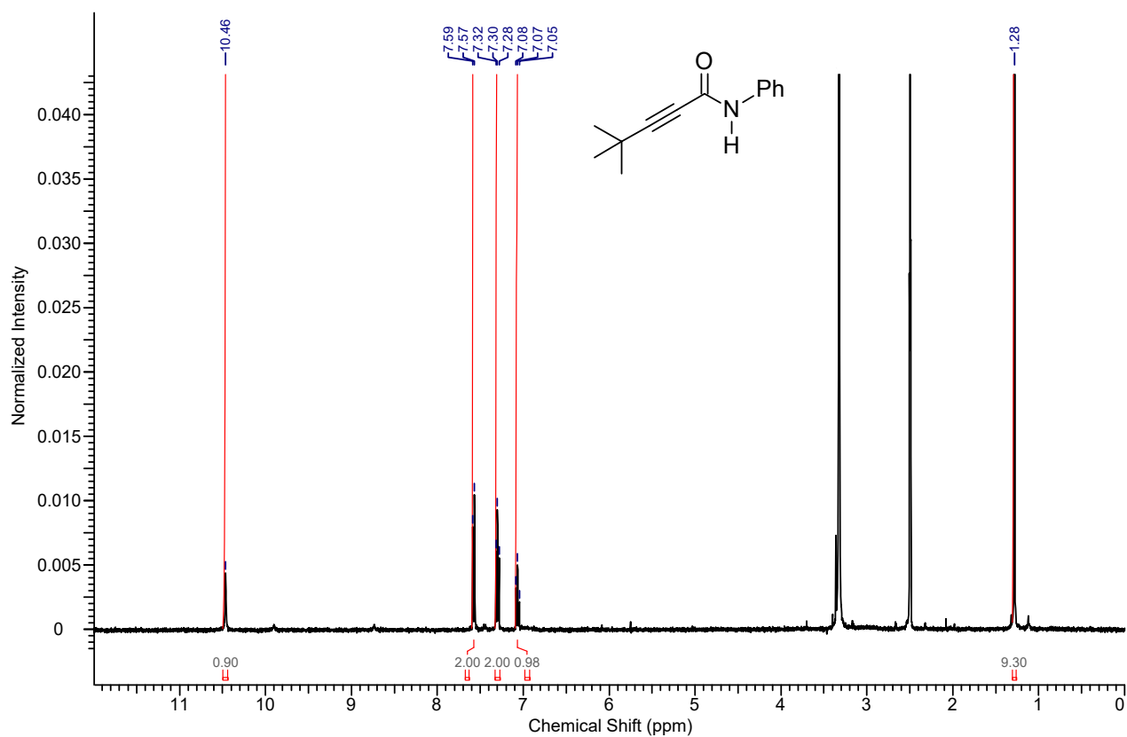
1 H NMR spectrum of the compound 7i
