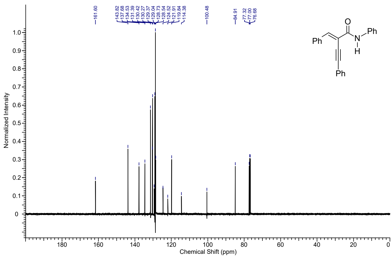
13 C NMR spectrum of the compound 5aa
