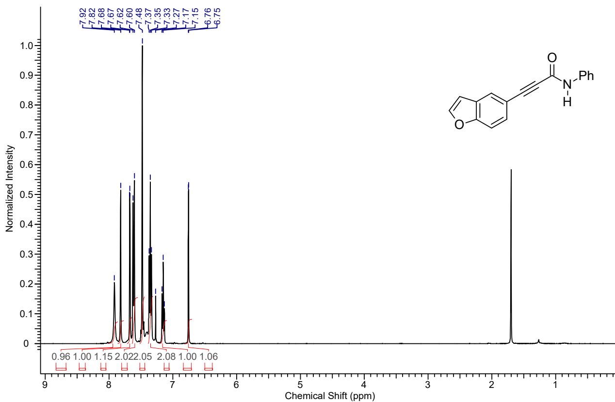
1 H NMR spectrum of the compound 4ta
