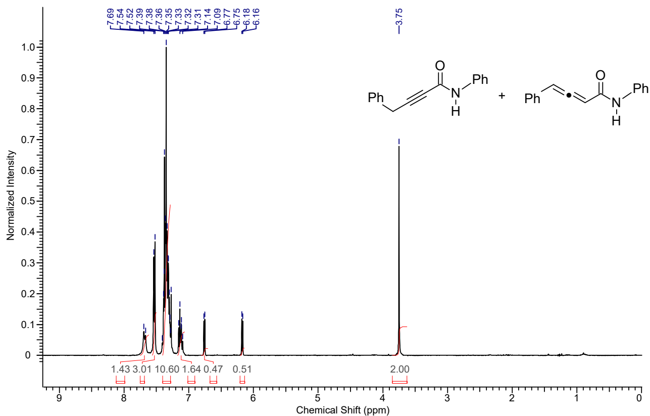
1 H NMR spectrum of the compound 7e (a 2:1 mixture of 7e and 7ea )
