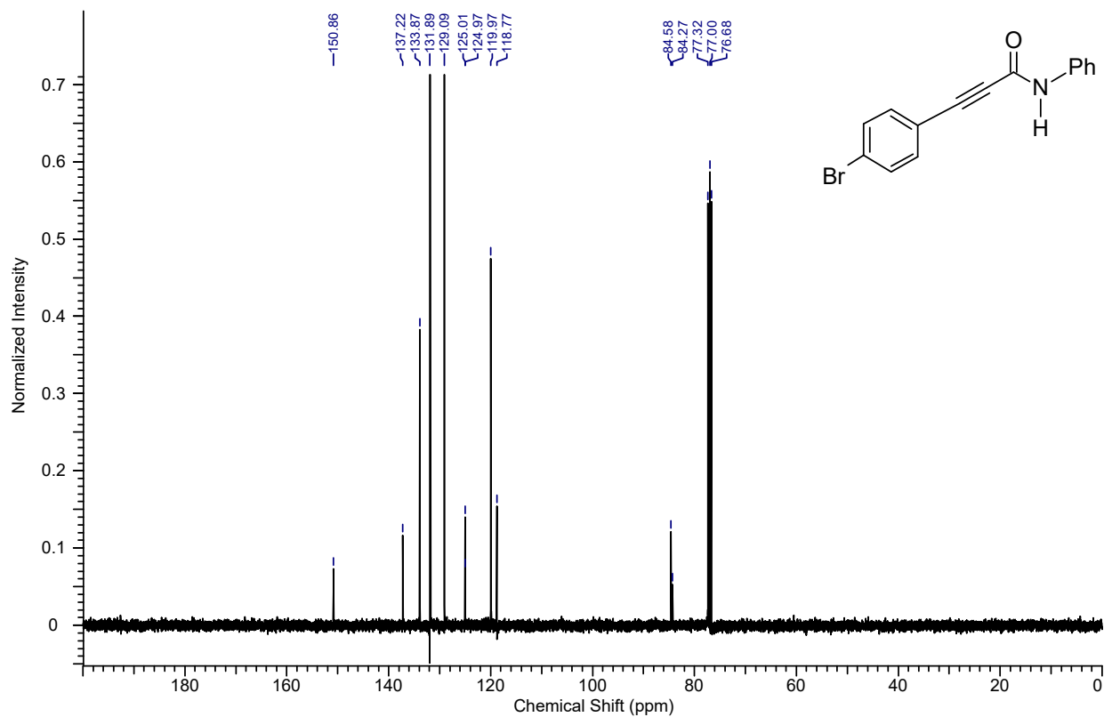
13 C NMR spectrum of the compound 4ga
