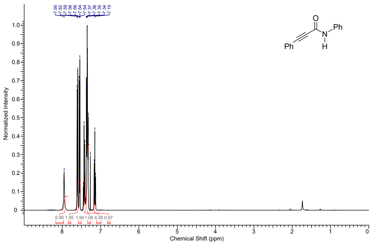
1 H NMR spectrum of the compound 4aa
