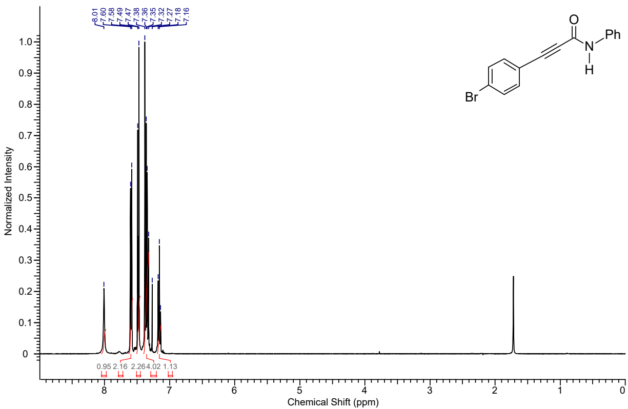
1 H NMR spectrum of the compound 4ga
