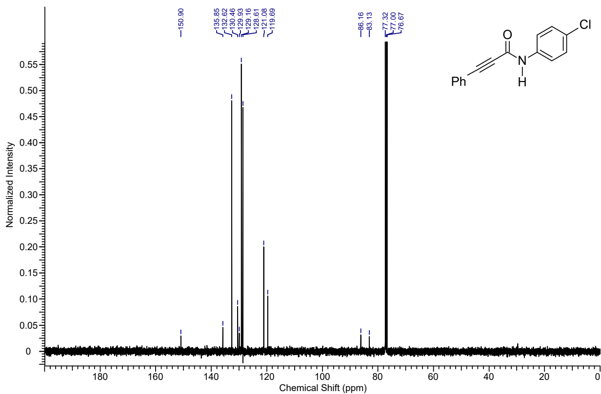
13 C NMR spectrum of the compound 4ac
