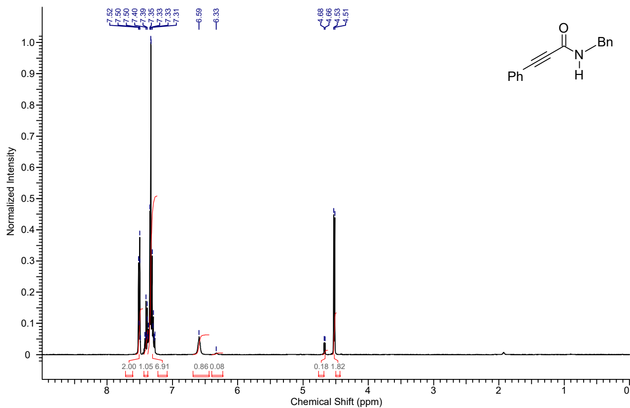
1 H NMR spectrum of the compound 4ap (a 9:1 mixture of rotamers)
