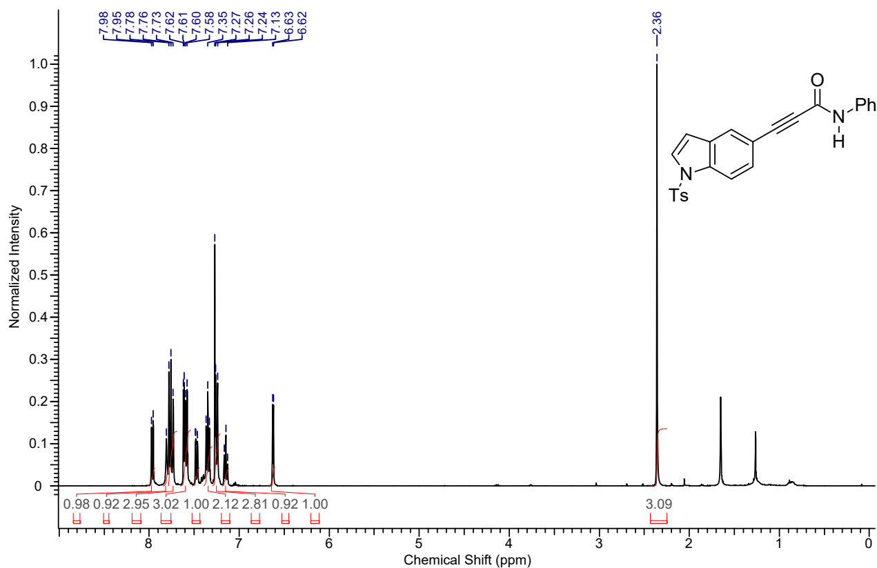
1 H NMR spectrum of the compound 4ua
