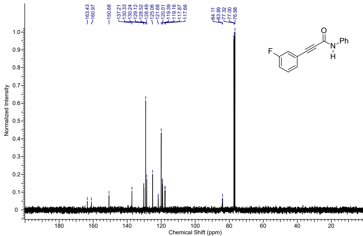
13 C NMR spectrum of the compound 4a
