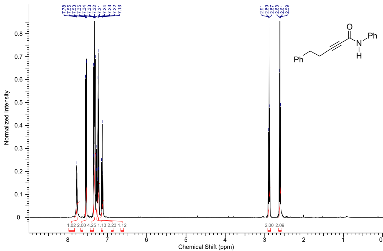
1 H NMR spectrum of the compound 7d
