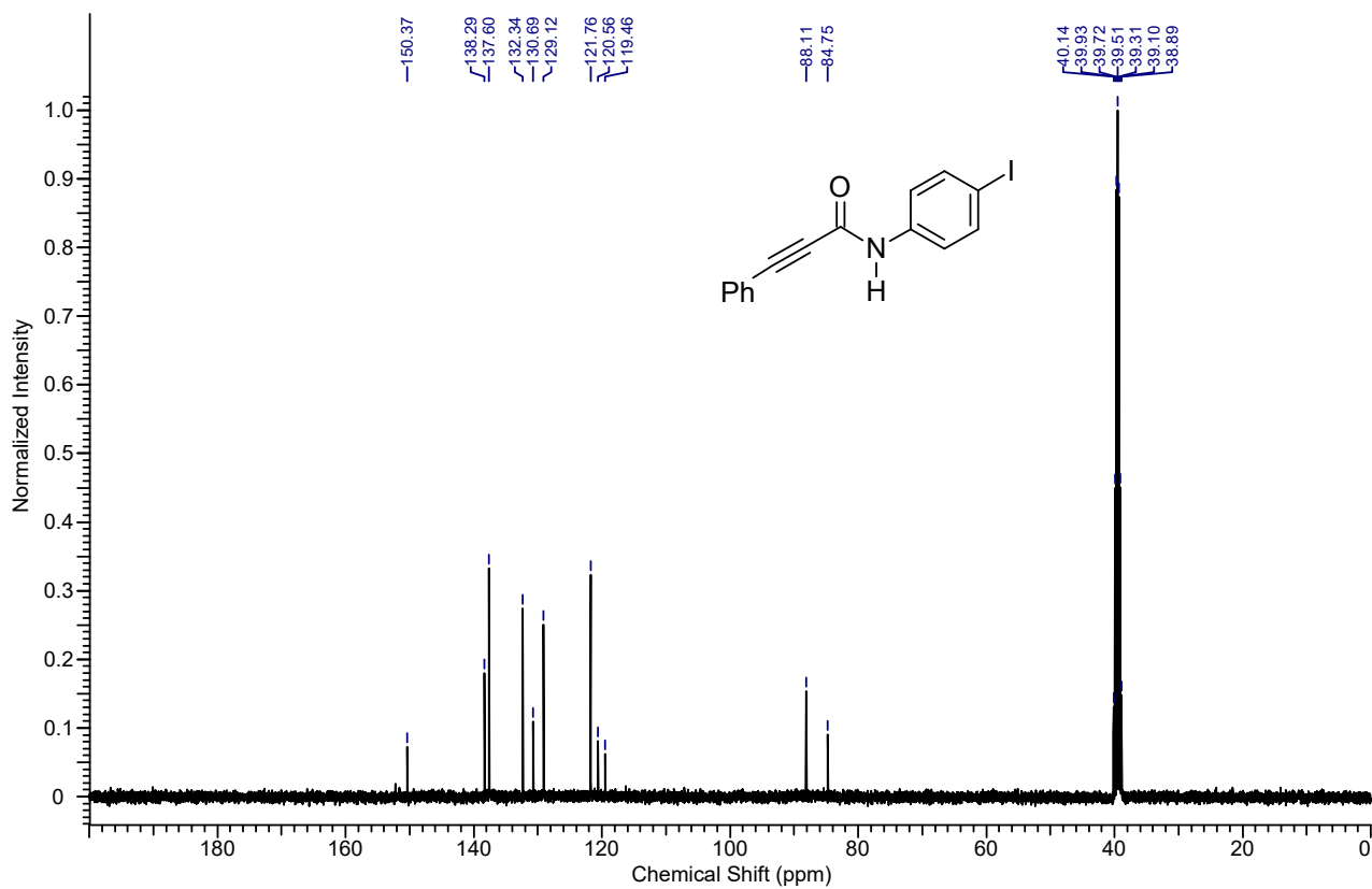
13 C NMR spectrum of the compound 4ae
