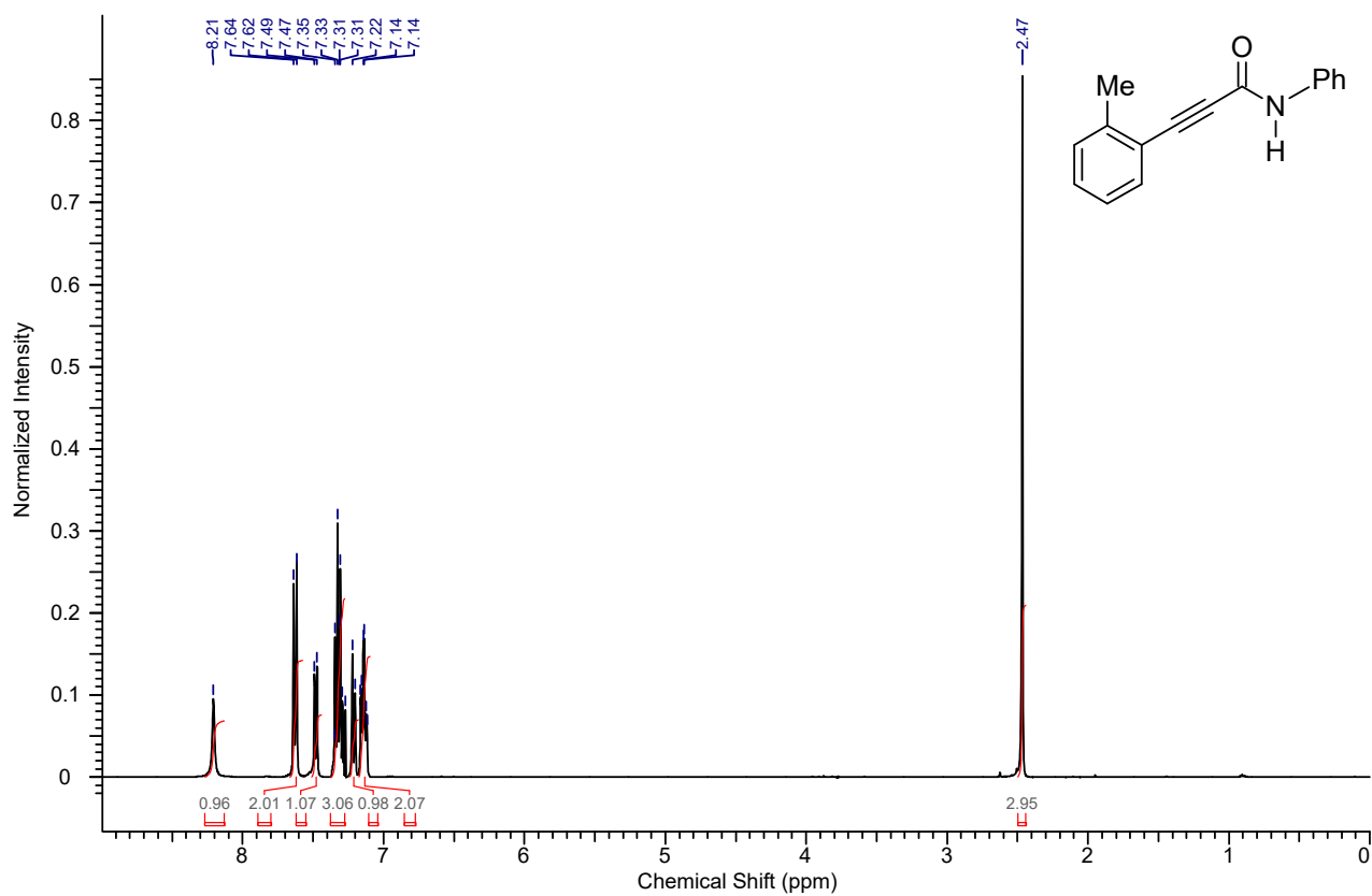
1 H NMR spectrum of the compound 4qa
