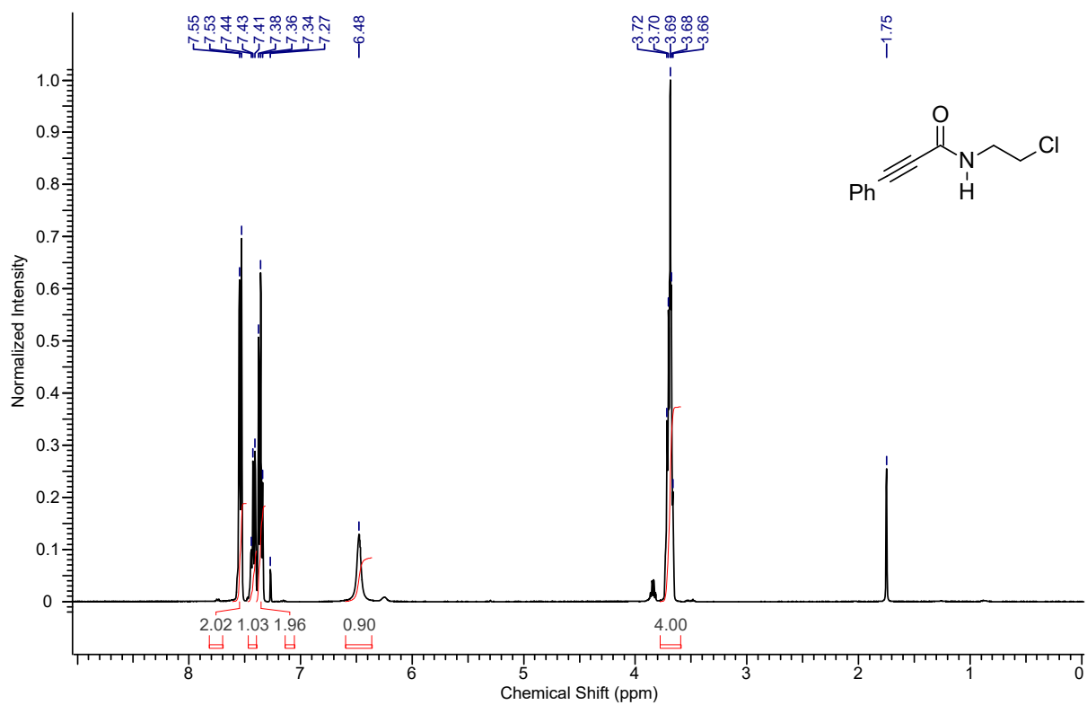
1 H NMR spectrum of the compound 4at
