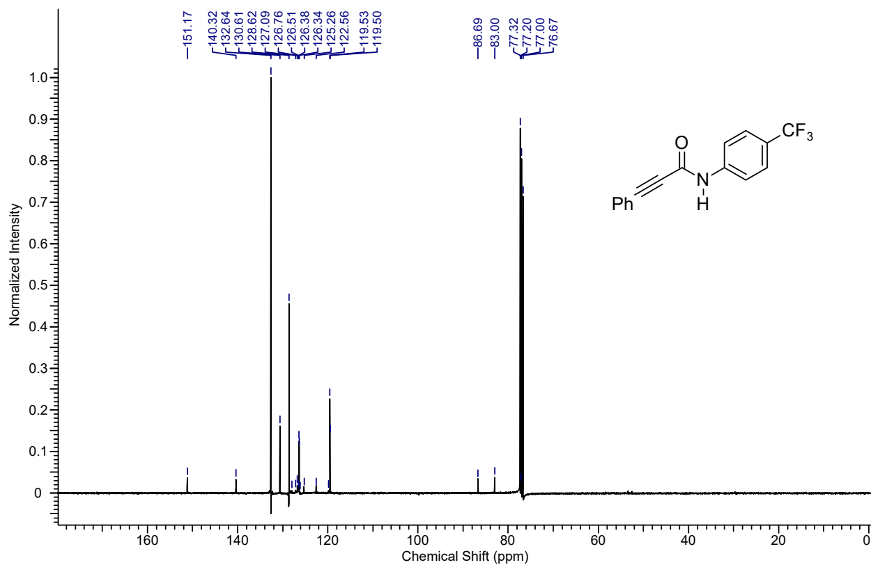
13 C NMR spectrum of the compound 4ag
