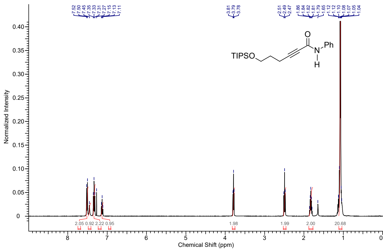
1 H NMR spectrum of the compound 7k
