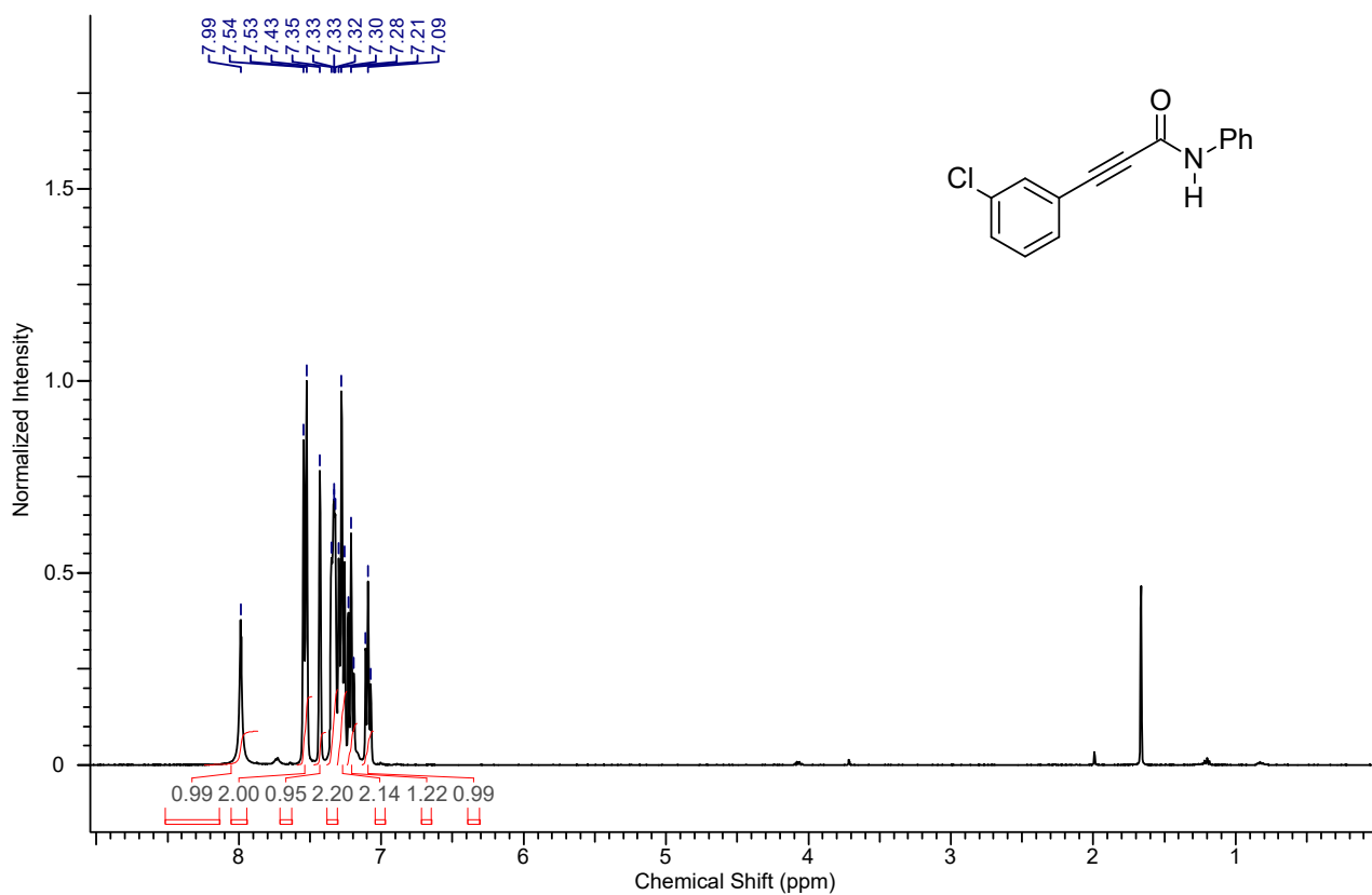
1 H NMR spectrum of the compound 4ma
