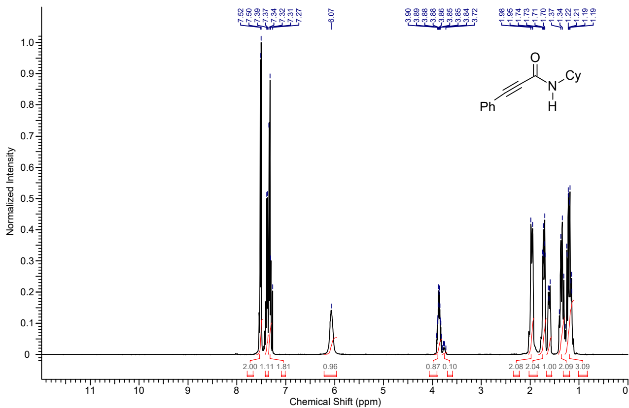
1 H NMR spectrum of the compound 4ar (a 9:1 mixture of rotamers)
