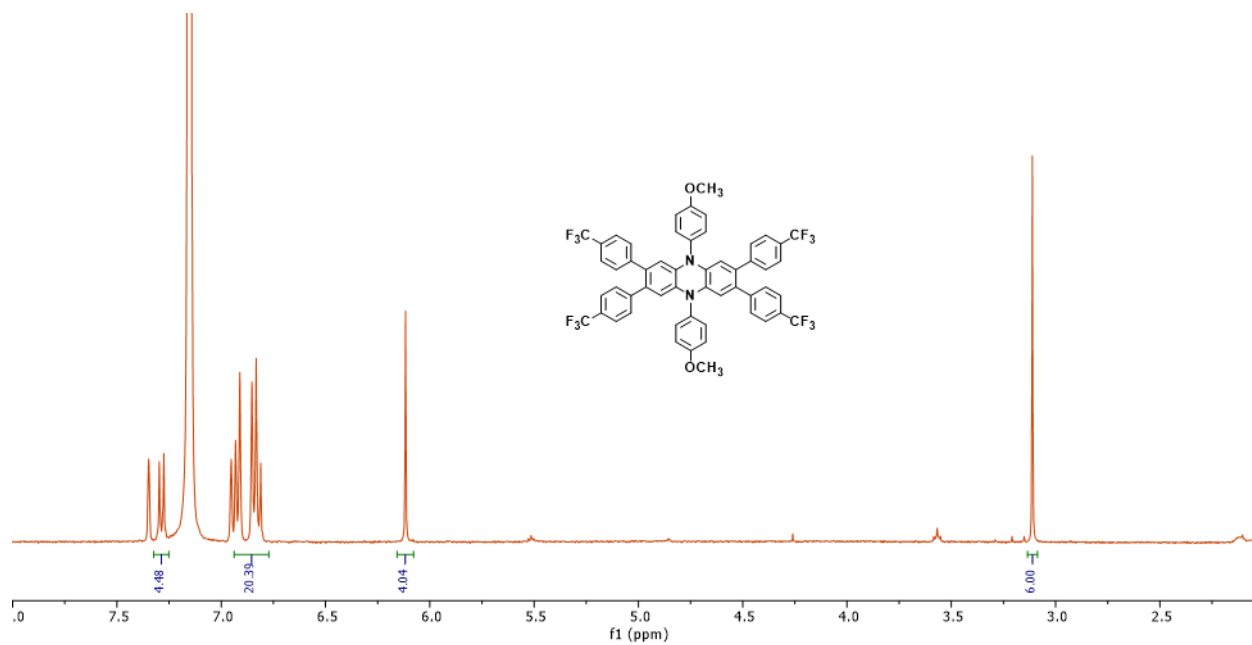
Figure S116. 1 H-NMR spectrum of 4a in C 6 D 6 after recrystallization.
