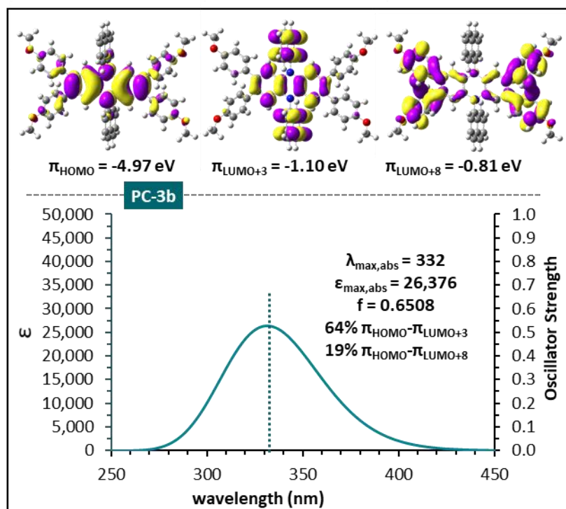
Figure S67: Computationally modeled molecular orbitals predicted to be involved in absorption transitions for PC 3b detailed below (top). Computationally predicted UV-vis spectrum of PCs 3b along with theoretically assigned percentage contributions (>15%) of various orbitals to the predicted absorption peaks. \lambda_{\text{max,abs}} is the predicted absorption maximum wavelength and is reported in units of nm, \epsilon_{\text{max,abs}} is the predicted molar extinction coefficient at the predicted \lambda_{\text{max,abs}} and is reported in units of \text{M}^{-1} \text{ cm}^{-1} , and f is the predicted oscillator strength; all of these values were predicted at the TD-DFT CAM-B3LYP/6-31+G(d,p)/CPCM-DMA level of theory (bottom).
