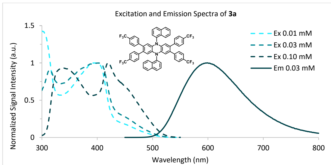
Figure S9. Fluorescence spectra of PC 3a . Dashed lines are the excitation spectra at varying concentrations in DMAc and the solid line is the emission spectrum at 0.03 mM in DMAc. Emission spectra was collected using an excitation wavelength of 385 nm and is representative of emission profiles at all concentrations between 0.01 mM and 0.10 mM. Excitation spectra were collected for emission at 586 nm.
