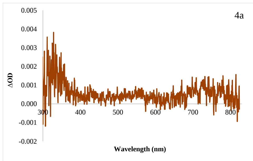
Figure S23. Spectral absorption of PC 4a in DMAc at a 200 ns time delay, with no emission subtraction. There are no distinguishable features that can be followed by kinetic absorption. The spectral absorption data was offset corrected using kinetic data acquired at \lambda = 450 nm.
