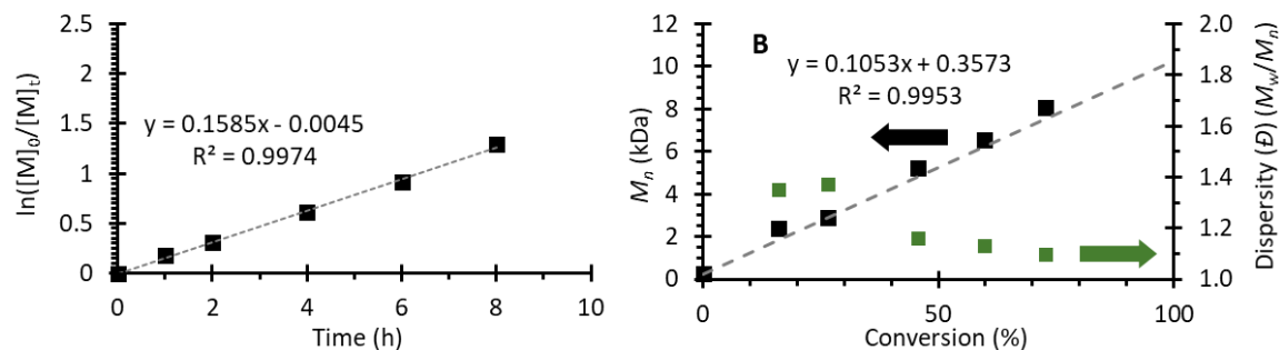
Figure S92. Polymerization data from Run 18 (Table S3). [MMA]:[DMAc]:[DBMM]:[5a] = [1000]:[1000]:[10]:[0.1]. (A) First order kinetic plot of the natural log of monomer consumption as a function of time. (B) Plot of molecular weight ( M_n ) growth as a function of monomer conversion (black squares), theoretical M_n growth as a function of monomer conversion (dashed grey line), and dispersity as a function of monomer conversion (green squares). Equation on chart (B) represents the trendline for the measured M_n growth as a function of conversion.
