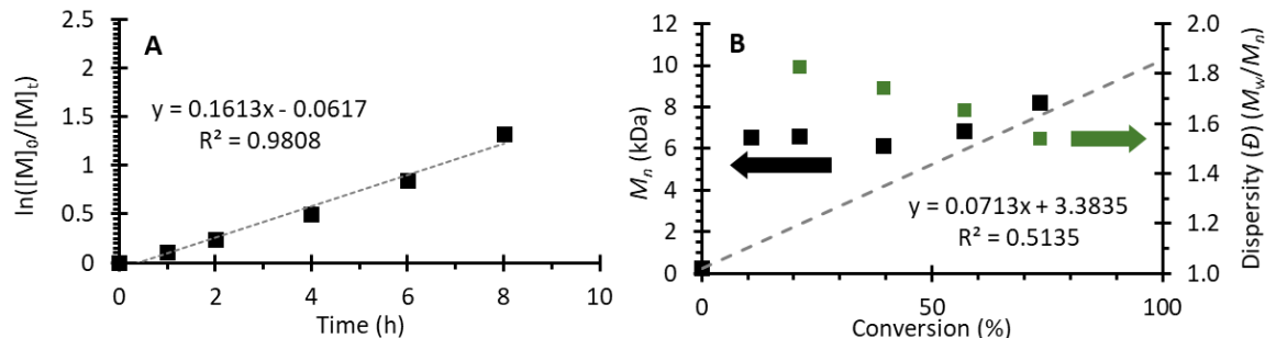
Figure S96. Polymerization data from Run 22 (Table S3). [MMA]:[DMAc]:[DBMM]:[ 5b ] = [1000]:[1000]:[10]:[0.1]. (A) First order kinetic plot of the natural log of monomer consumption as a function of time. (B) Plot of molecular weight ( M_n ) growth as a function of monomer conversion (black squares), theoretical M_n growth as a function of monomer conversion (dashed grey line), and dispersity as a function of monomer conversion (green squares). Equation on chart (B) represents the trendline for the measured M_n growth as a function of conversion.
