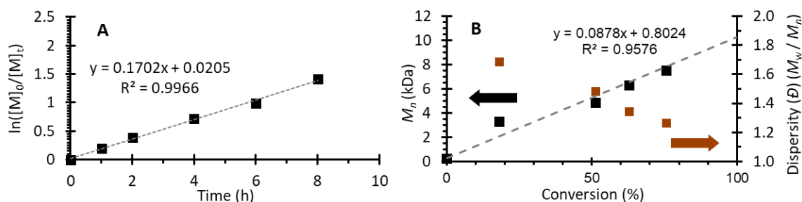
Figure S85. Polymerization data from Run 11 (Table S3). [MMA]:[DMAc]:[DBMM]:[4a] = [1000]:[1000]:[10]:[0.05]. (A) First order kinetic plot of the natural log of monomer consumption as a function of time. (B) Plot of molecular weight ( M_n ) growth as a function of monomer conversion (black squares), theoretical M_n growth as a function of monomer conversion (dashed grey line), and dispersity as a function of monomer conversion (orange squares). Equation on chart (B) represents the trendline for the measured M_n growth as a function of conversion.
