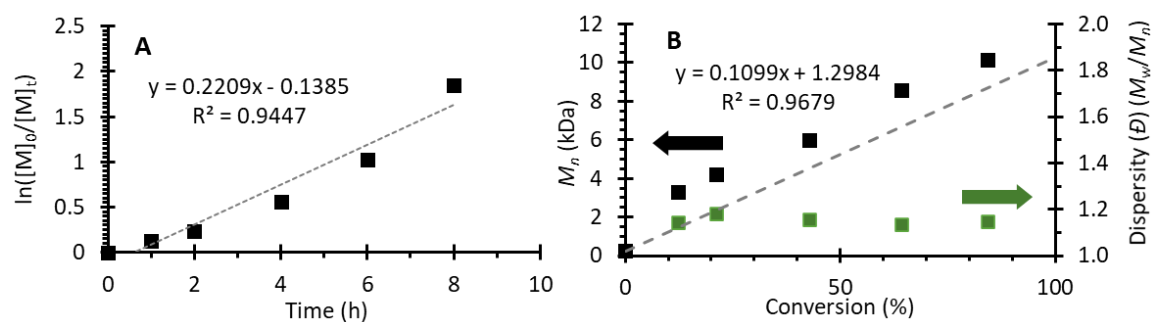
Figure S87. Polymerization data from Run 13 (Table S3). [MMA]:[DMAc]:[DBMM]:[5] = [1000]:[1000]:[10]:[0.5]. (A) First order kinetic plot of the natural log of monomer consumption as a function of time. (B) Plot of molecular weight ( M_n ) growth as a function of monomer conversion (black squares), theoretical M_n growth as a function of monomer conversion (dashed grey line), and dispersity as a function of monomer conversion (green squares). Equation on chart (B) represents the trendline for the measured M_n growth as a function of conversion.
