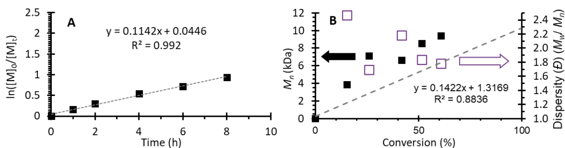
Figure S106. Polymerization data from Run 35 (Table S4). [MMA]:[DMAc]:[DBMM]:[PhenO*] = [1000]:[1000]:[10]:[0.1]. (A) First order kinetic plot of the natural log of monomer consumption as a function of time. (B) Plot of molecular weight ( M_n ) growth as a function of monomer conversion (black squares), theoretical M_n growth as a function of monomer conversion (dashed grey line), and dispersity as a function of monomer conversion (orange squares). Equation on chart (B) represents the trendline for the measured M_n growth as a function of conversion. *(PhenO: 3,7-Di([1,1'-biphenyl]-4-yl)-10-(naphthalen-1-yl)-10H-phenoxazine).
