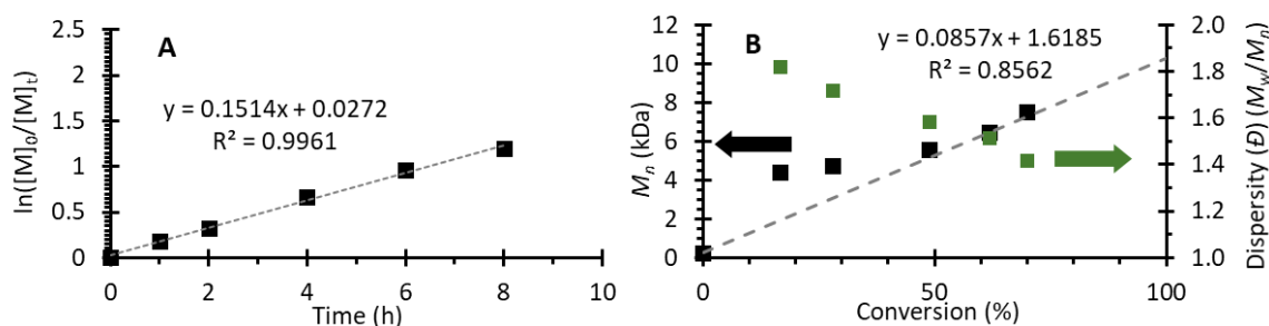
Figure S94. Polymerization data from Run 20 (Table S3). [MMA]:[DMAc]:[DBMM]:[ 5a ] = [1000]:[1000]:[10]:[0.01]. (A) First order kinetic plot of the natural log of monomer consumption as a function of time. (B) Plot of molecular weight ( M_n ) growth as a function of monomer conversion (black squares), theoretical M_n growth as a function of monomer conversion (dashed grey line), and dispersity as a function of monomer conversion (green squares). Equation on chart (B) represents the trendline for the measured M_n growth as a function of conversion.
