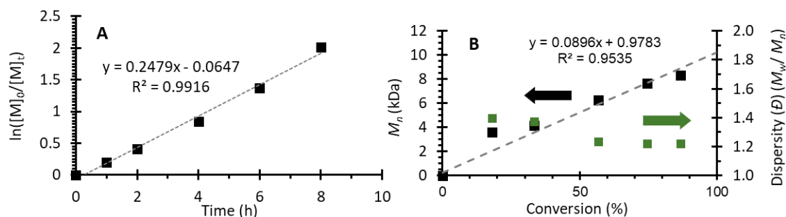
Figure S89. Polymerization data from Run 15 (Table S3). [MMA]:[DMAc]:[DBMM]:[5] = [1000]:[1000]:[10]:[0.05]. (A) First order kinetic plot of the natural log of monomer consumption as a function of time. (B) Plot of molecular weight ( M_n ) growth as a function of monomer conversion (black squares), theoretical M_n growth as a function of monomer conversion (dashed grey line), and dispersity as a function of monomer conversion (green squares). Equation on chart (B) represents the trendline for the measured M_n growth as a function of conversion.
