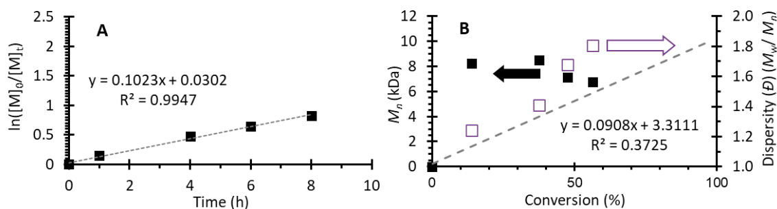
Figure S105. Polymerization data from Run 34 (Table S4). [MMA]:[DMAc]:[DBMM]:[PhenO*] = [1000]:[1000]:[10]:[0.05]. (A) First order kinetic plot of the natural log of monomer consumption as a function of time. (B) Plot of molecular weight ( M_n ) growth as a function of monomer conversion (black squares), theoretical M_n growth as a function of monomer conversion (dashed grey line), and dispersity as a function of monomer conversion (orange squares). Equation on chart (B) represents the trendline for the measured M_n growth as a function of conversion. *(PhenO: 3,7-Di([1,1'-biphenyl]-4-yl)-10-(naphthalen-1-yl)-10H-phenoxazine).
