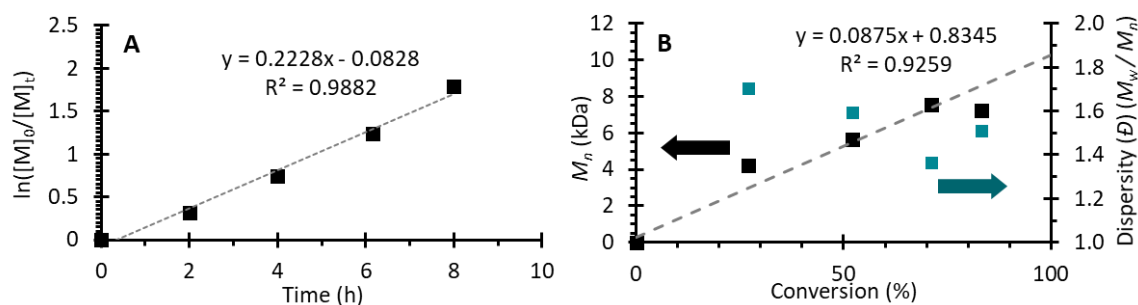
Figure S101. Polymerization data from Run 27 (Table S4). [MMA]:[Benz]:[DBMM]:[ 3a ] = [1000]:[1000]:[10]:[0.01]. (A) First order kinetic plot of the natural log of monomer consumption as a function of time. (B) Plot of molecular weight ( M_n ) growth as a function of monomer conversion (black squares), theoretical M_n growth as a function of monomer conversion (dashed grey line), and dispersity as a function of monomer conversion (blue squares). Equation on chart (B) represents the trendline for the measured M_n growth as a function of conversion.
