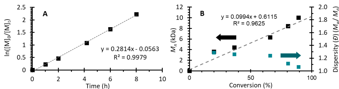
Figure S99. Polymerization data from Run 25 (Table S4). [MMA]:[Benz]:[DBMM]:[ 3a ] = [1000]:[1000]:[10]:[0.05]. (A) First order kinetic plot of the natural log of monomer consumption as a function of time. (B) Plot of molecular weight ( M_n ) growth as a function of monomer conversion (black squares), theoretical M_n growth as a function of monomer conversion (dashed grey line), and dispersity as a function of monomer conversion (blue squares). Equation on chart (B) represents the trendline for the measured M_n growth as a function of conversion.
