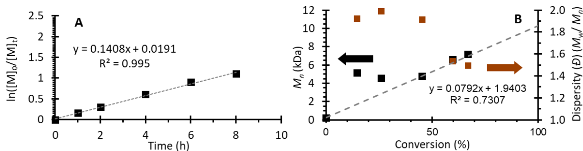
Figure S86. Polymerization data from Run 12 (Table S3). [MMA]:[DMAc]:[DBMM]:[4a] = [1000]:[1000]:[10]:[0.01]. (A) First order kinetic plot of the natural log of monomer consumption as a function of time. (B) Plot of molecular weight ( M_n ) growth as a function of monomer conversion (black squares), theoretical M_n growth as a function of monomer conversion (dashed grey line), and dispersity as a function of monomer conversion (orange squares). Equation on chart (B) represents the trendline for the measured M_n growth as a function of conversion.
