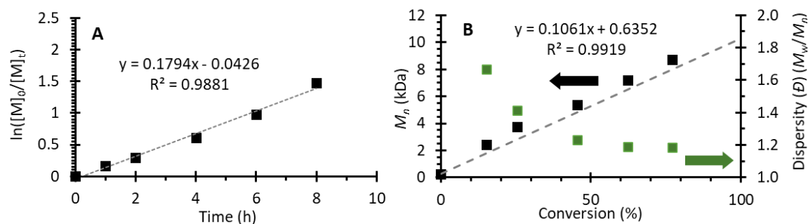
Figure S88. Polymerization data from Run 14 (Table S3). [MMA]:[DMAc]:[DBMM]:[5] = [1000]:[1000]:[10]:[0.1]. (A) First order kinetic plot of the natural log of monomer consumption as a function of time. (B) Plot of molecular weight ( M_n ) growth as a function of monomer conversion (black squares), theoretical M_n growth as a function of monomer conversion (dashed grey line), and dispersity as a function of monomer conversion (green squares). Equation on chart (B) represents the trendline for the measured M_n growth as a function of conversion.
