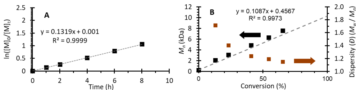
Figure S84. Polymerization data from Run 10 (Table S3). [MMA]:[DMAc]:[DBMM]:[ 4a ] = [1000]:[1000]:[10]:[0.1]. (A) First order kinetic plot of the natural log of monomer consumption as a function of time. (B) Plot of molecular weight ( M_n ) growth as a function of monomer conversion (black squares), theoretical M_n growth as a function of monomer conversion (dashed grey line), and dispersity as a function of monomer conversion (orange squares). Equation on chart (B) represents the trendline for the measured M_n growth as a function of conversion.
