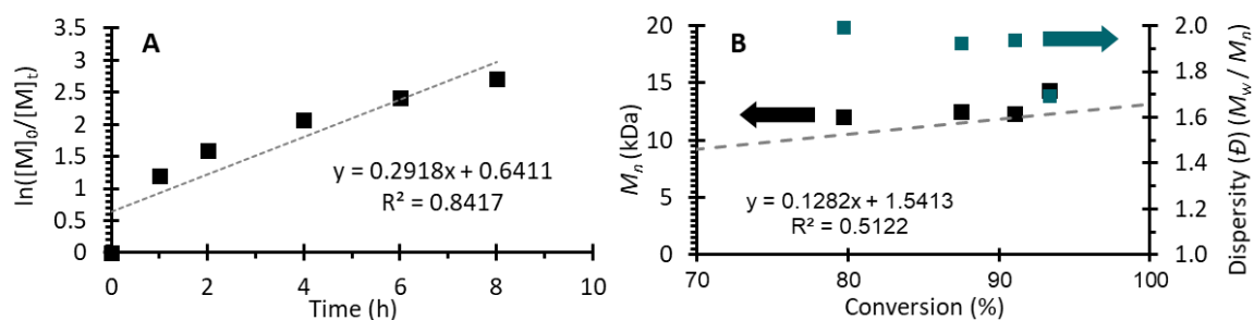
Figure S102. Polymerization data from Run 28 (Table S4). [nBA]:[Benz]:[DBMM]:[ 3a ] = [1000]:[1000]:[10]:[0.05]. (A) First order kinetic plot of the natural log of monomer consumption as a function of time. (B) Plot of molecular weight ( M_n ) growth as a function of monomer conversion (black squares), theoretical M_n growth as a function of monomer conversion (dashed grey line), and dispersity as a function of monomer conversion (blue squares). Equation on chart (B) represents the trendline for the measured M_n growth as a function of conversion.
