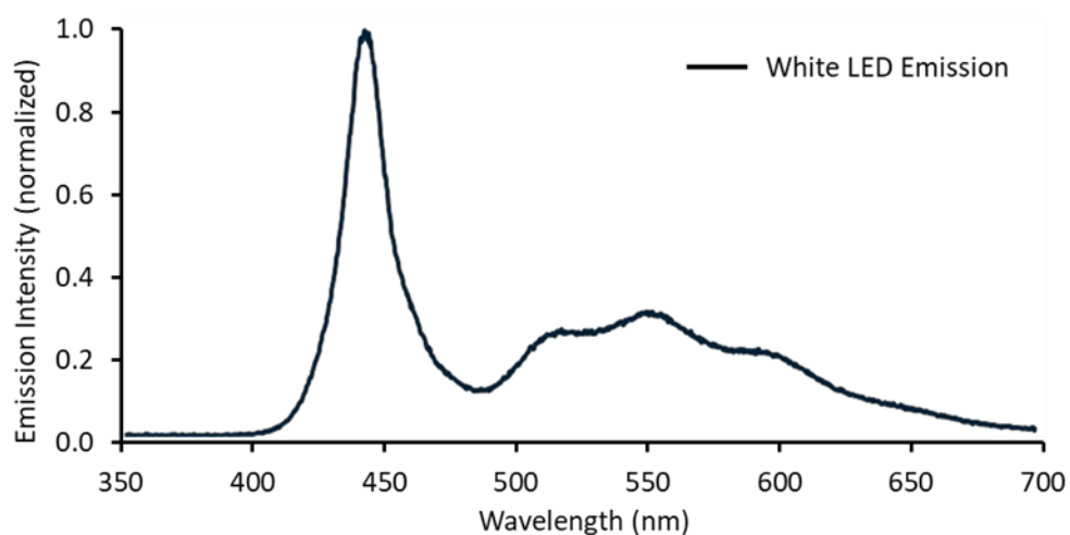
Figure S2. Normalized emission spectra of white light LEDs from creative lighting solutions.
