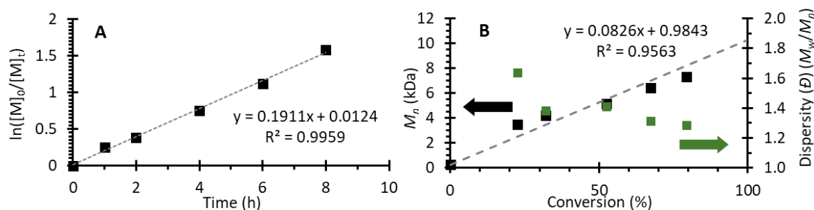
Figure S93. Polymerization data from Run 19 (Table S3). [MMA]:[DMAc]:[DBMM]:[ 5a ] = [1000]:[1000]:[10]:[0.05]. (A) First order kinetic plot of the natural log of monomer consumption as a function of time. (B) Plot of molecular weight ( M_n ) growth as a function of monomer conversion (black squares), theoretical M_n growth as a function of monomer conversion (dashed grey line), and dispersity as a function of monomer conversion (green squares). Equation on chart (B) represents the trendline for the measured M_n growth as a function of conversion.
