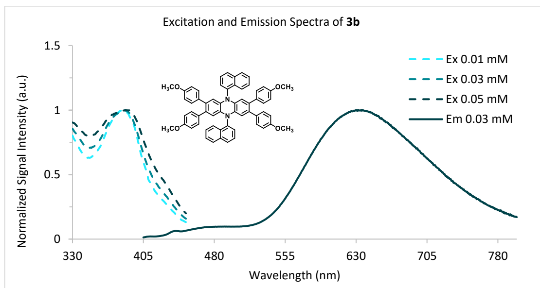
Figure S11. Fluorescence spectra of PC 3b . Dashed lines are the excitation spectra at varying concentrations in DMAc and the solid line is the emission spectrum at 0.03 mM in DMAc. Emission spectra was collected using an excitation wavelength of 385 nm and is representative of emission profiles at all concentrations between 0.01 mM and 0.10 mM. Excitation spectra were collected for emission at 636 nm.
