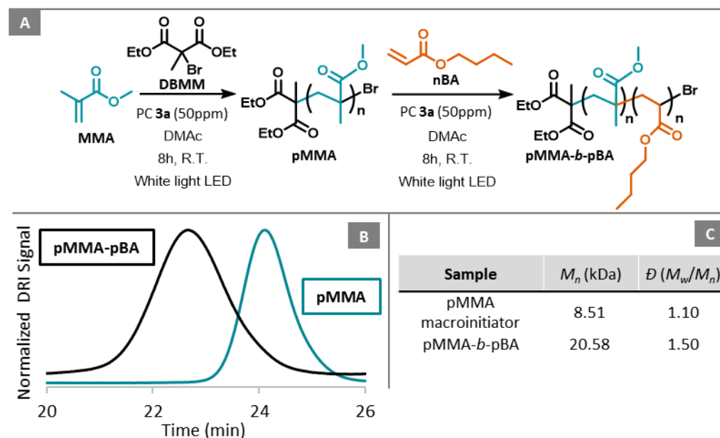
Figure S108. (A) Reaction scheme for chain extension of pMMA macroinitiator with nBA to form pMMA- b -pBA. The polymerization of the macromonomer was run in DMAc using DBMM as the initiator and MMA as the monomer in a ratio of [MMA]:[DBMM]:[3a] = [1000]:[10]:[0.05]. (B) Overlaid GPC traces of the isolated pMMA macroinitiator and the isolated pMMA- b -pBA block copolymer. (C) Molecular weight data (obtained using GPC) for the isolated pMMA macroinitiator and the isolated pMMA- b -nBA block copolymer.
