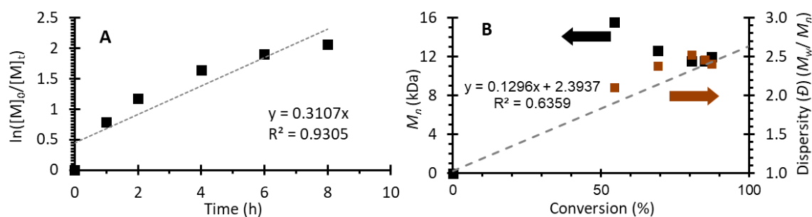
Figure S103. Polymerization data from Run 32 (Table S4). [nBA]:[Benz]:[DBMM]:[4a] = [1000]:[1000]:[10]:[0.05]. (A) First order kinetic plot of the natural log of monomer consumption as a function of time. (B) Plot of molecular weight ( M_n ) growth as a function of monomer conversion (black squares), theoretical M_n growth as a function of monomer conversion (dashed grey line), and dispersity as a function of monomer conversion (orange squares). Equation on chart (B) represents the trendline for the measured M_n growth as a function of conversion.
