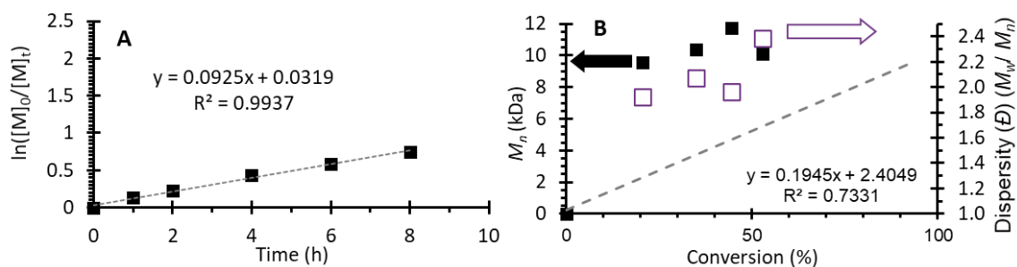
Figure S107. Polymerization data from Run 36 (Table S4). [MMA]:[DMAc]:[DBMM]:[PhenO*] = [1000]:[1000]:[10]:[0.5]. (A) First order kinetic plot of the natural log of monomer consumption as a function of time. (B) Plot of molecular weight ( M_n ) growth as a function of monomer conversion (black squares), theoretical M_n growth as a function of monomer conversion (dashed grey line), and dispersity as a function of monomer conversion (orange squares). Equation on chart (B) represents the trendline for the measured M_n growth as a function of conversion. *(PhenO: 3,7-Di([1,1'-biphenyl]-4-yl)-10-(naphthalen-1-yl)-10H-phenoxazine).
