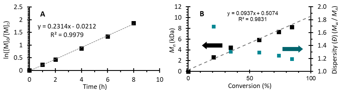
Figure S78. Polymerization data from Run 3 (Table S3). [MMA]:[DMAc]:[DBMM]:[ 3 ] = [1000]:[1000]:[10]:[0.05]. (A) First order kinetic plot of the natural log of monomer consumption as a function of time. (B) Plot of molecular weight ( M_n ) growth as a function of monomer conversion (black squares), theoretical M_n growth as a function of monomer conversion (dashed grey line), and dispersity as a function of monomer conversion (blue squares). Equation on chart (B) represents the trendline for the measured M_n growth as a function of conversion.
