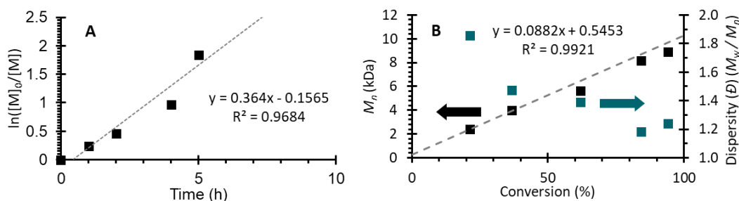
Figure S100. Polymerization data from Run 26 (Table S4). [MMA]:[DCM]:[DBMM]:[ 3a ] = [1000]:[1000]:[10]:[0.05]. (A) First order kinetic plot of the natural log of monomer consumption as a function of time. (B) Plot of molecular weight ( M_n ) growth as a function of monomer conversion (black squares), theoretical M_n growth as a function of monomer conversion (dashed grey line), and dispersity as a function of monomer conversion (blue squares). Equation on chart (B) represents the trendline for the measured M_n growth as a function of conversion.
