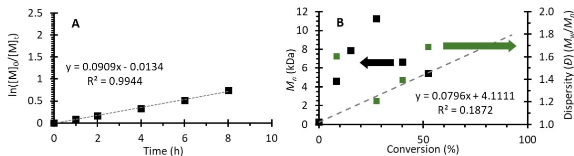
Figure S95. Polymerization data from Run 21 (Table S3). [MMA]:[DMAc]:[DBMM]:[ 5b ] = [1000]:[1000]:[10]:[0.5]. (A) First order kinetic plot of the natural log of monomer consumption as a function of time. (B) Plot of molecular weight ( M_n ) growth as a function of monomer conversion (black squares), theoretical M_n growth as a function of monomer conversion (dashed grey line), and dispersity as a function of monomer conversion (green squares). Equation on chart (B) represents the trendline for the measured M_n growth as a function of conversion.
