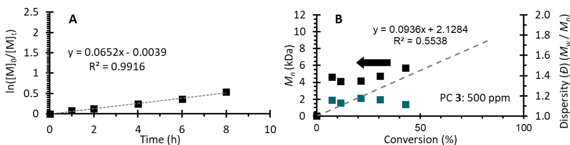
Figure S76. Polymerization data from Run 1 (Table S3). [MMA]:[DMAc]:[DBMM]:[ 3 ] = [1000]:[1000]:[10]:[0.5]. (A) First order kinetic plot of the natural log of monomer consumption as a function of time. (B) Plot of molecular weight ( M_n ) growth as a function of monomer conversion (black squares), theoretical M_n growth as a function of monomer conversion (dashed grey line), and dispersity as a function of monomer conversion (blue squares). Equation on chart (B) represents the trendline for the measured M_n growth as a function of conversion.
