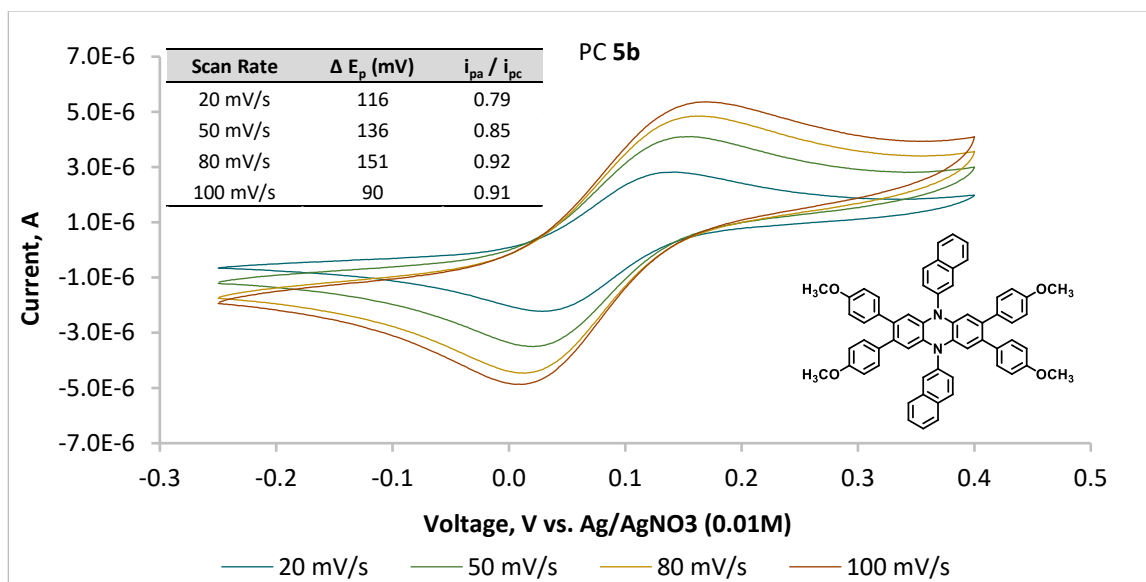
Figure S60. Cyclic voltammogram of PC 5b in DMAc at 20 mV/s, 50 mV/s, 80 mV/s, and 100 mV/s scan rates. Inserted into the graph is a chart showing the ratios of peak anodic current to peak cathodic current ( i_{pa}/i_{pc} ) and the difference between peak anodic and peak cathodic current ( \Delta E_p ) at each scan rate.
