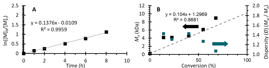
Figure S77. Polymerization data from Run 2 (Table S3). [MMA]:[DMAc]:[DBMM]:[ 3 ] = [1000]:[1000]:[10]:[0.1]. (A) First order kinetic plot of the natural log of monomer consumption as a function of time. (B) Plot of molecular weight ( M_n ) growth as a function of monomer conversion (black squares), theoretical M_n growth as a function of monomer conversion (dashed grey line), and dispersity as a function of monomer conversion (blue squares). Equation on chart (B) represents the trendline for the measured M_n growth as a function of conversion.
