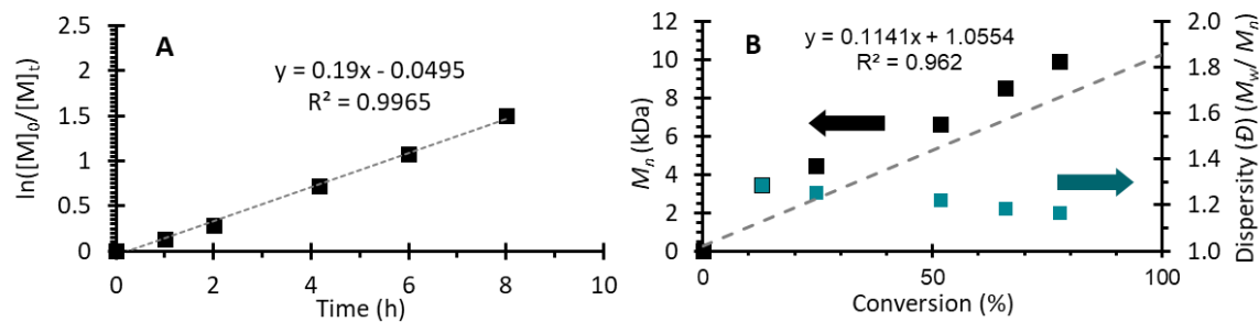
Figure S97. Polymerization data from Run 23 (Table S4). [MMA]:[THF]:[DBMM]:[ 3a ] = [1000]:[1000]:[10]:[0.05]. (A) First order kinetic plot of the natural log of monomer consumption as a function of time. (B) Plot of molecular weight ( M_n ) growth as a function of monomer conversion (black squares), theoretical M_n growth as a function of monomer conversion (dashed grey line), and dispersity as a function of monomer conversion (blue squares). Equation on chart (B) represents the trendline for the measured M_n growth as a function of conversion.
