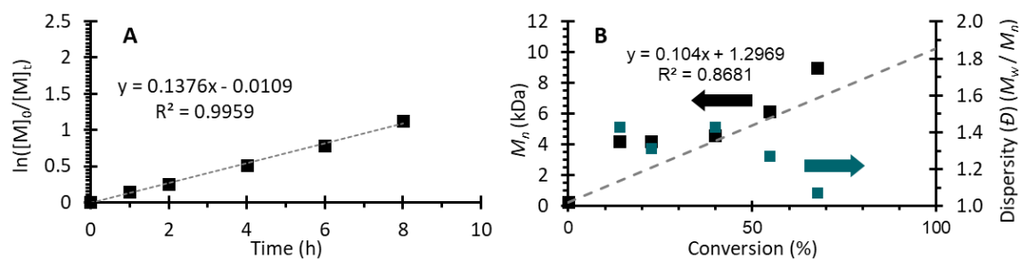
Figure S80. Polymerization data from Run 5 (Table S3). [MMA]:[DMAc]:[DBMM]:[ 3a ] = [1000]:[1000]:[10]:[0.1]. (A) First order kinetic plot of the natural log of monomer consumption as a function of time. (B) Plot of molecular weight ( M_n ) growth as a function of monomer conversion (black squares), theoretical M_n growth as a function of monomer conversion (dashed grey line), and dispersity as a function of monomer conversion (blue squares). Equation on chart (B) represents the trendline for the measured M_n growth as a function of conversion.
