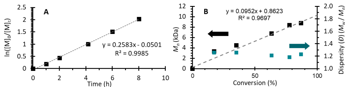
Figure S98. Polymerization data from Run 24 (Table S4). [MMA]:[EtOAc]:[DBMM]:[ 3a ] = [1000]:[1000]:[10]:[0.05]. (A) First order kinetic plot of the natural log of monomer consumption as a function of time. (B) Plot of molecular weight ( M_n ) growth as a function of monomer conversion (black squares), theoretical M_n growth as a function of monomer conversion (dashed grey line), and dispersity as a function of monomer conversion (blue squares). Equation on chart (B) represents the trendline for the measured M_n growth as a function of conversion.
