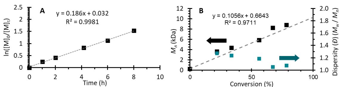
Figure S81. Polymerization data from Run 6 (Table S3). [MMA]:[DMAc]:[DBMM]:[ 3a ] = [1000]:[1000]:[10]:[0.05]. (A) First order kinetic plot of the natural log of monomer consumption as a function of time. (B) Plot of molecular weight ( M_n ) growth as a function of monomer conversion (black squares), theoretical M_n growth as a function of monomer conversion (dashed grey line), and dispersity as a function of monomer conversion (blue squares). Equation on chart (B) represents the trendline for the measured M_n growth as a function of conversion.
