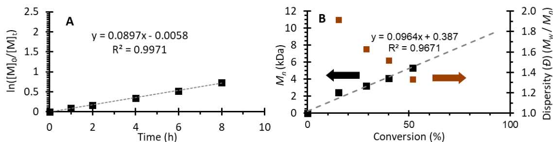
Figure S104. Polymerization data from Run 33 (Table S4). [MMA]:[Benz]:[DBMM]:[4a] = [1000]:[1000]:[10]:[0.01]. (A) First order kinetic plot of the natural log of monomer consumption as a function of time. (B) Plot of molecular weight ( M_n ) growth as a function of monomer conversion (black squares), theoretical M_n growth as a function of monomer conversion (dashed grey line), and dispersity as a function of monomer conversion (orange squares). Equation on chart (B) represents the trendline for the measured M_n growth as a function of conversion.
