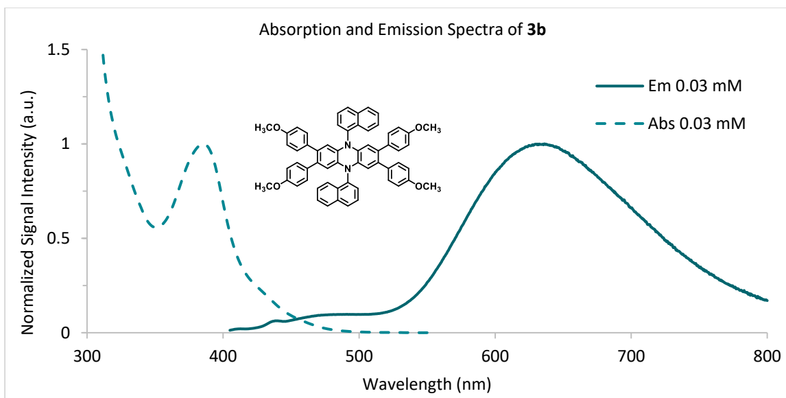
Figure S12. Emission spectra of PC 3b (solid) and absorption spectra of 3b (dashed) at 0.03 mM in DMAc. Absorption spectra was measured using UV-Vis and emission spectra was measured using fluorimetry. Emission spectra was collected using an excitation wavelength of 385 nm.
