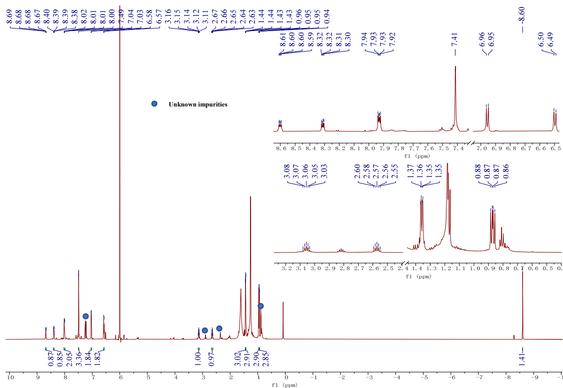
Figure S25 ^1\text{H} NMR spectrum of 5a (in \text{C}_2\text{D}_2\text{Cl}_4 )
