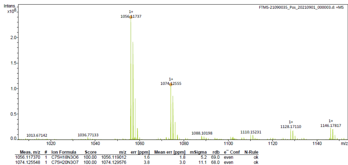
Figure S3 Mass spectrum of 2a
