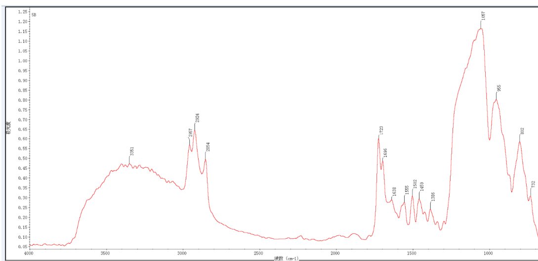
Figure S32 FTIR spectrum of 5b
