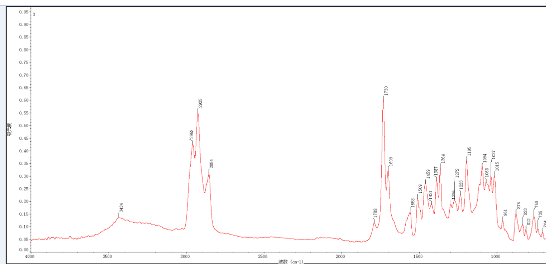
Figure S16 FTIR spectrum of 3b
