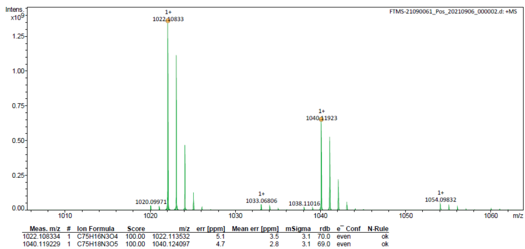
Figure S23 Mass spectrum of 4b
