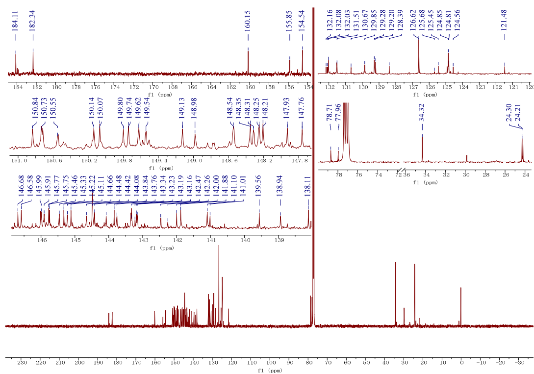
Figure S6 ^{13}\text{C} NMR spectrum of 2b (in \text{CDCl}_3 )
