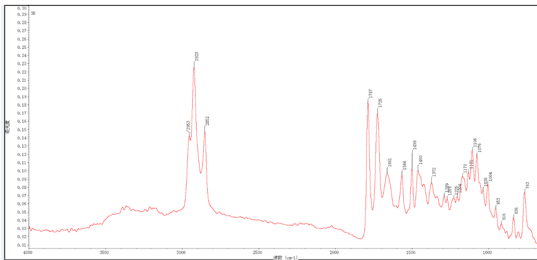
Figure S24 FTIR spectrum of 4b
