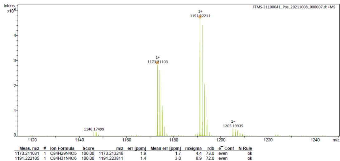
Figure S15 Mass spectrum of 3b
