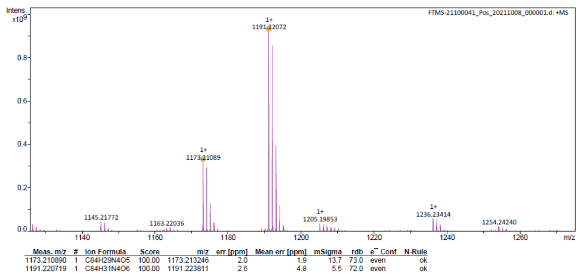
Figure S11 Mass spectrum of 3a
