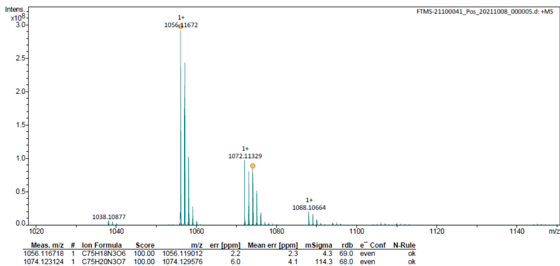
Figure S7 Mass spectrum of 2b
