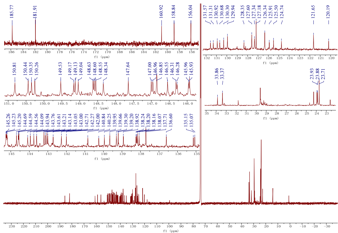
Figure S26 ^{13}\text{C} NMR spectrum of 5a (in \text{C}_2\text{D}_2\text{Cl}_4 )
