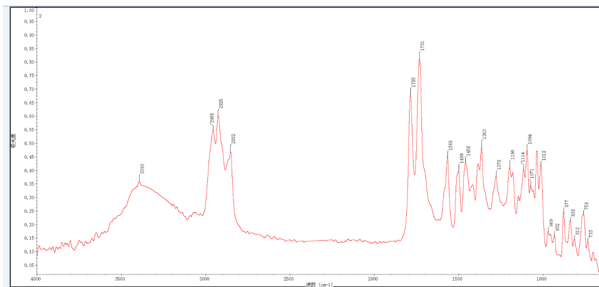
Figure S4 FTIR spectrum of 2a
