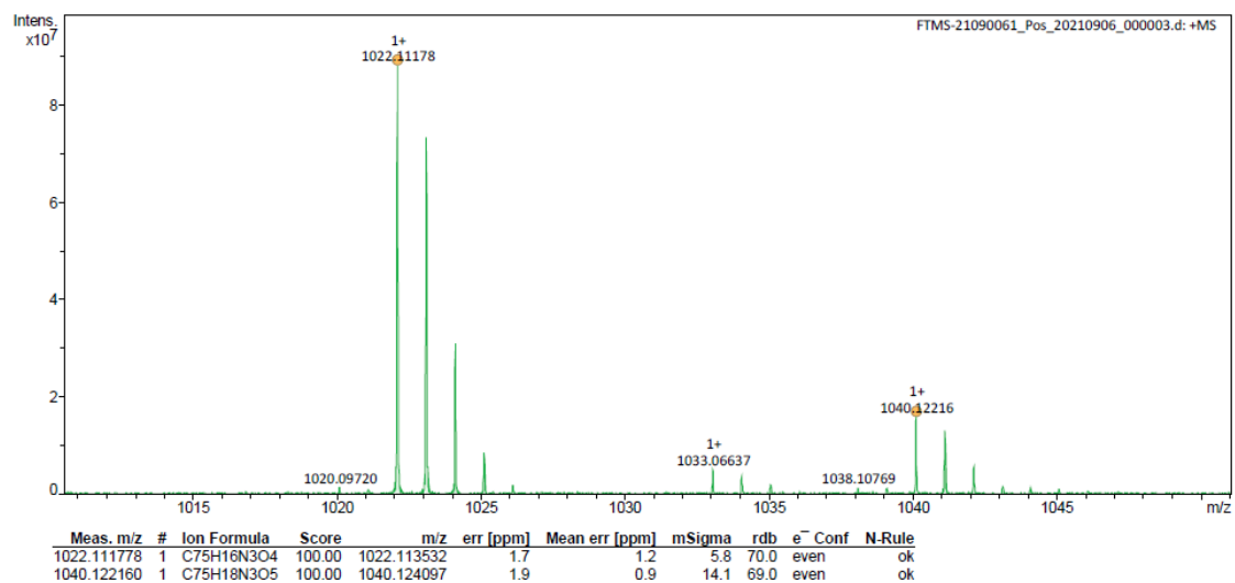
Figure S19 Mass spectrum of 4a
