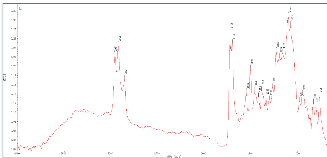
Figure S28 FTIR spectrum of 5a
