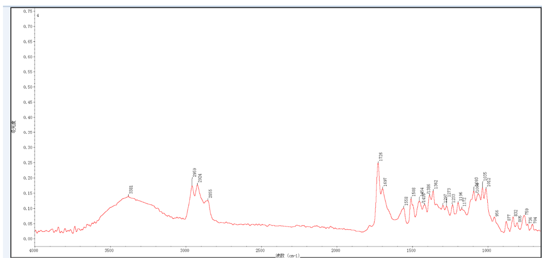
Figure S12 FTIR spectrum of 3a
