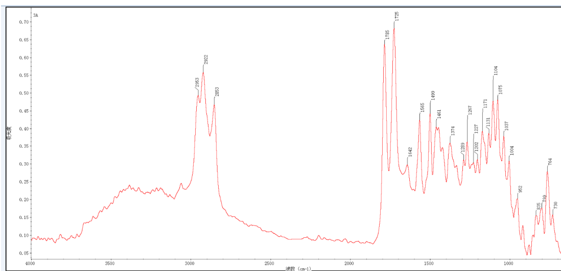
Figure S20 FTIR spectrum of 4a
