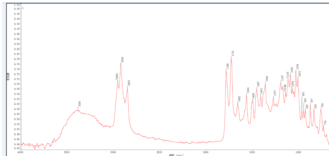
Figure S8 FTIR spectrum of 2b
