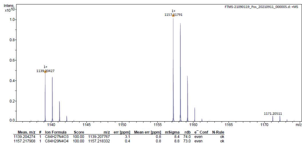
Figure S31 Mass spectrum of 5b
