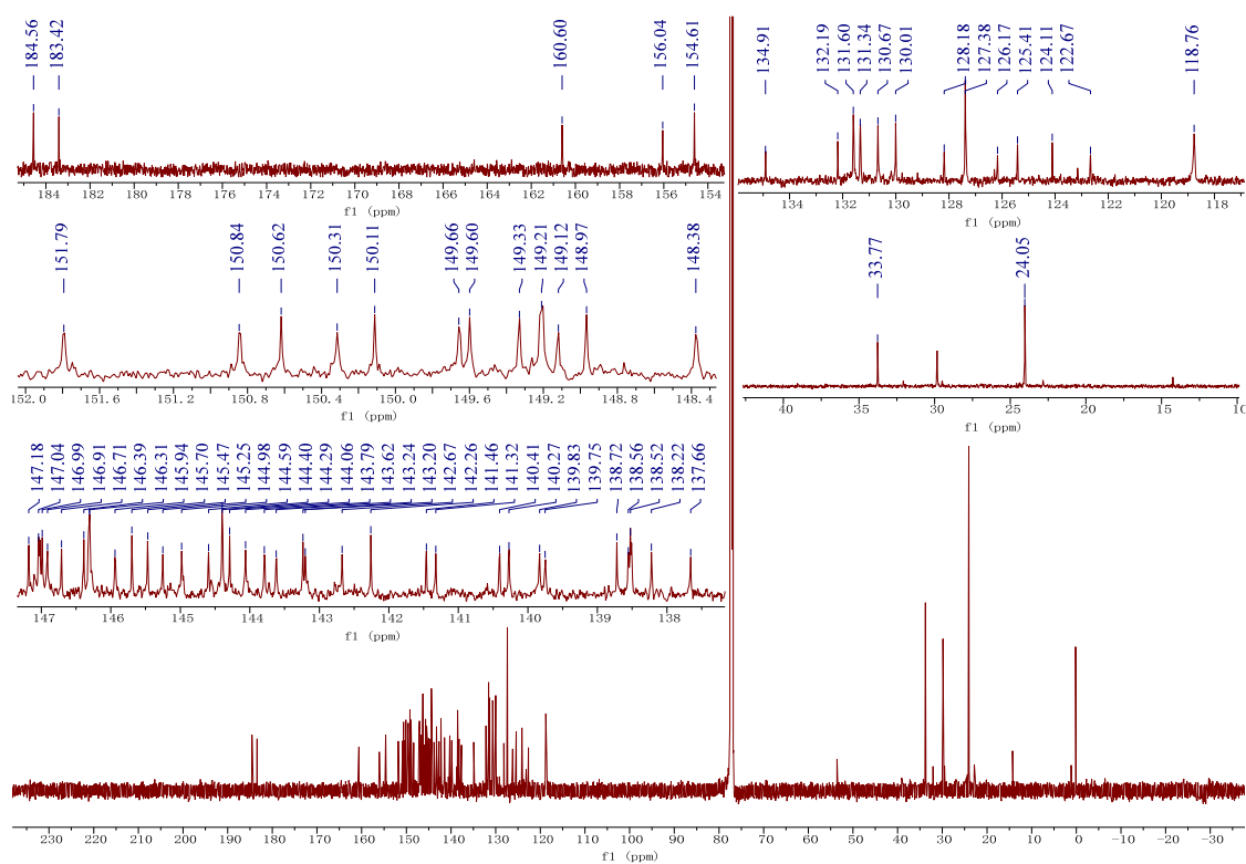
Figure S22 13 C NMR spectrum of 4b (in CDCl 3 )
