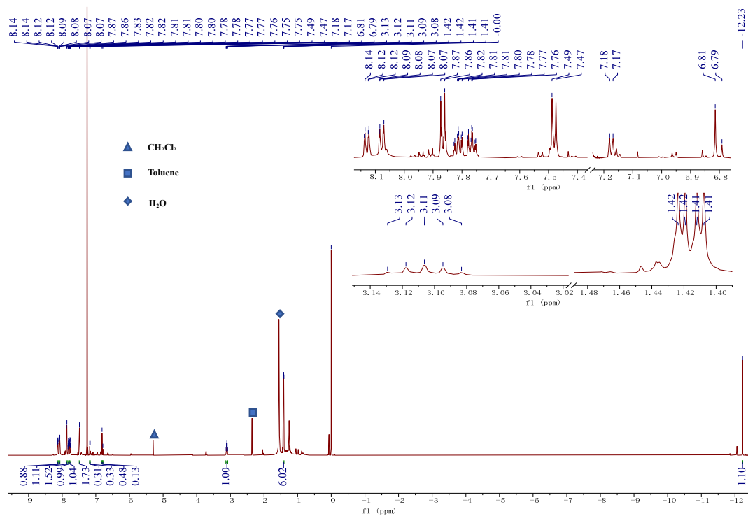
Figure S5 ^1\text{H} NMR spectrum of 2b (in \text{CDCl}_3 )
