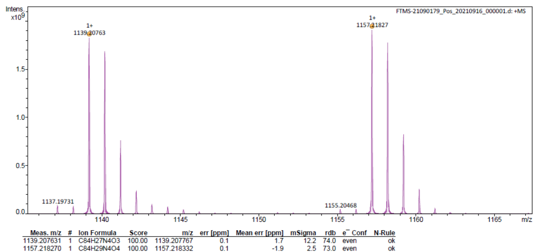
Figure S27 Mass spectrum of 5a
