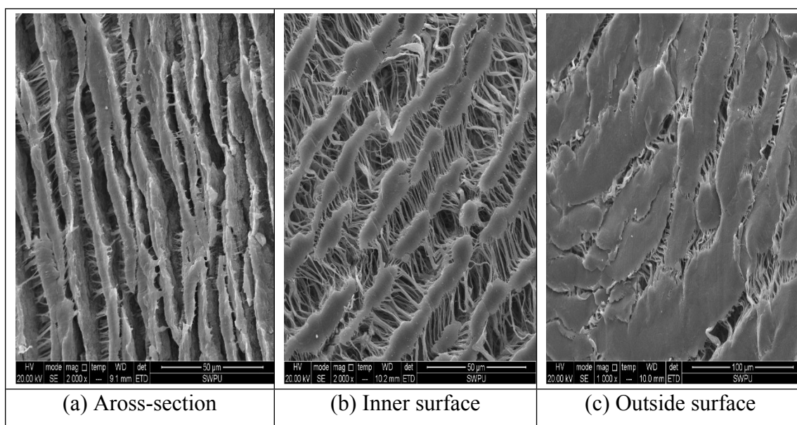
Fig. S1. SEM images of PTFE hollow fiber membrane
