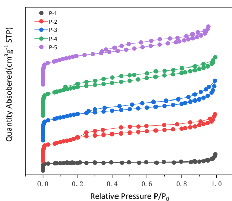
Fig. S2 N 2 adsorption isotherms of samples P-1 to P-5.
