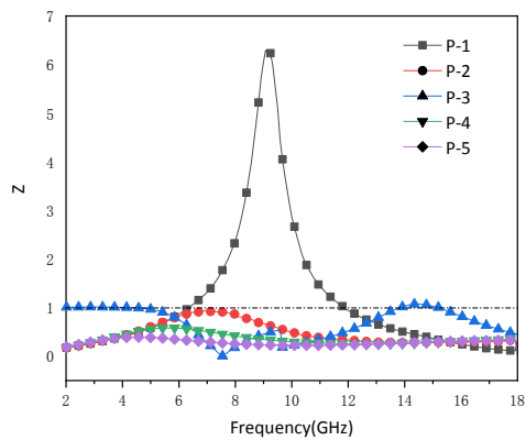
Fig. S3 Modulus of Z of samples P-1 to P-5.
