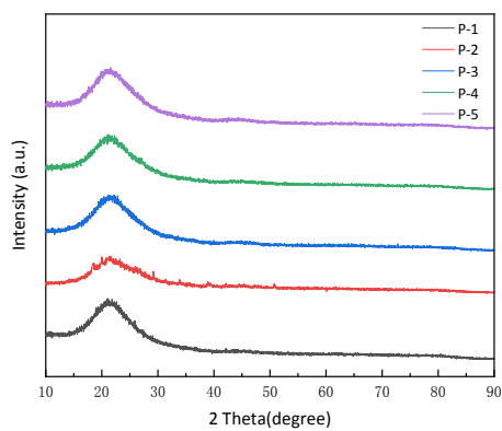
Fig. S1 XRD patterns of samples P1-P5.
