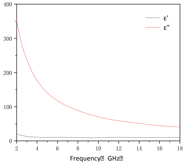
Fig. S4 Complex permittivity values of P3-20wt%.
