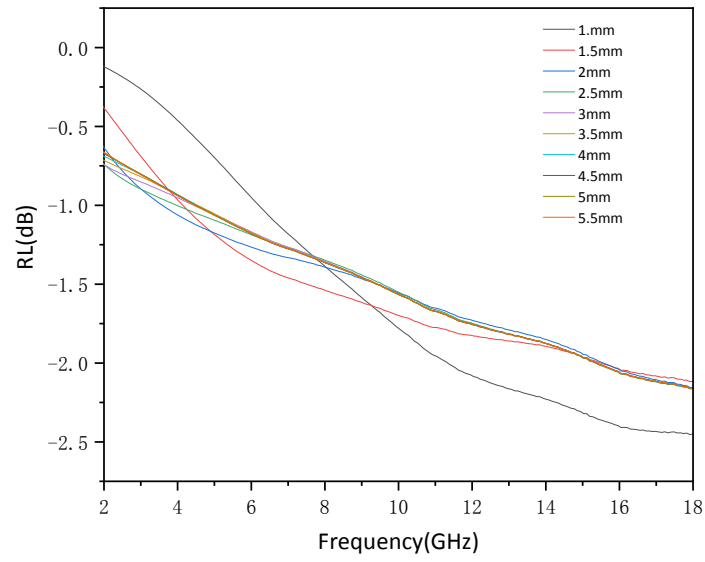
Fig. S5 Microwave reflection loss values at different thickness of different frequency of P3-25wt%.
