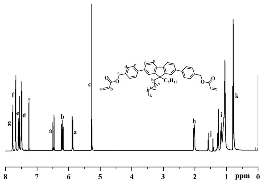
Fig.S3. 1 H NMR spectra for monomer M3 in CDCl 3 .
