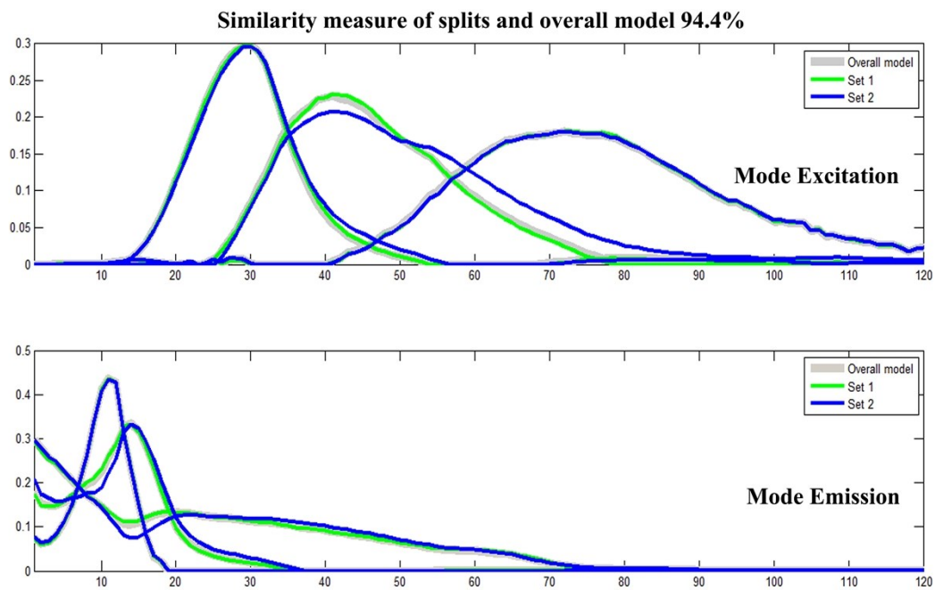
Fig.S4 split half validation of the three fluorescent components via PARAFAC analysis
