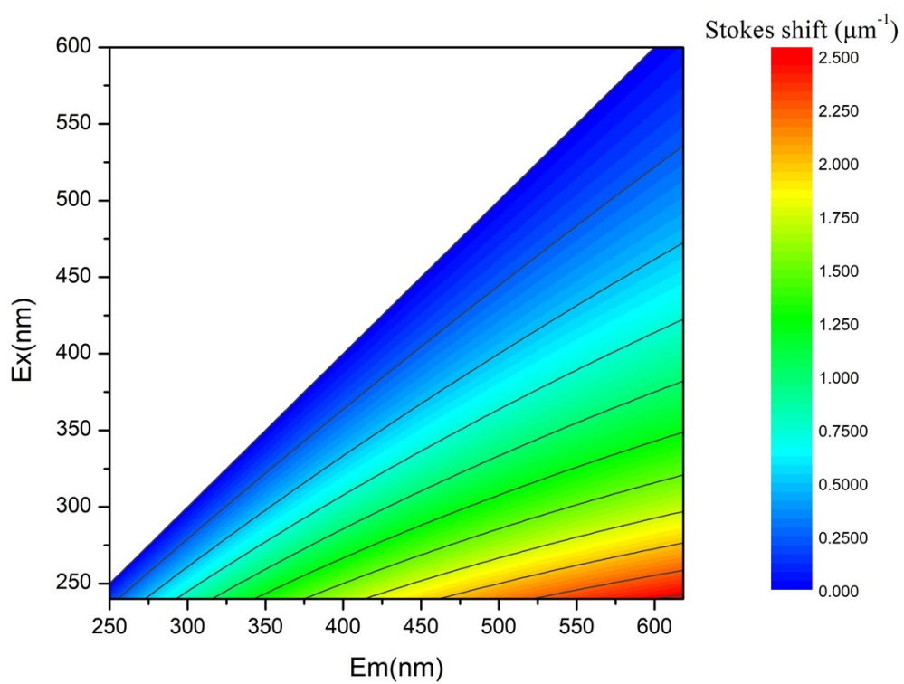
Fig. S2. Contour map of Stokes shift.
