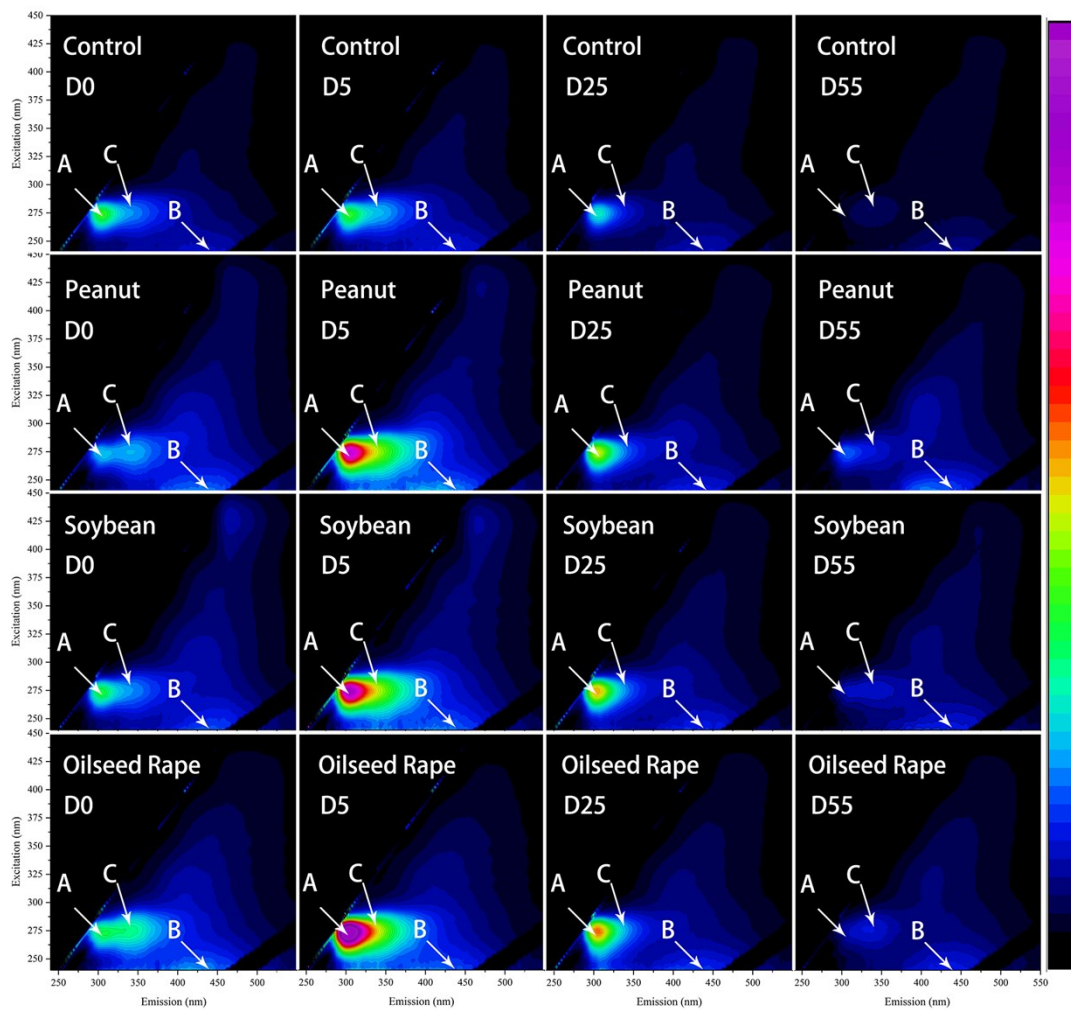
Fig. S3. Fluorescence EEMs of DOM in D 0 , D 5 , D 25 , and D 55 samples during anaerobic digestion of oil crop straw.
