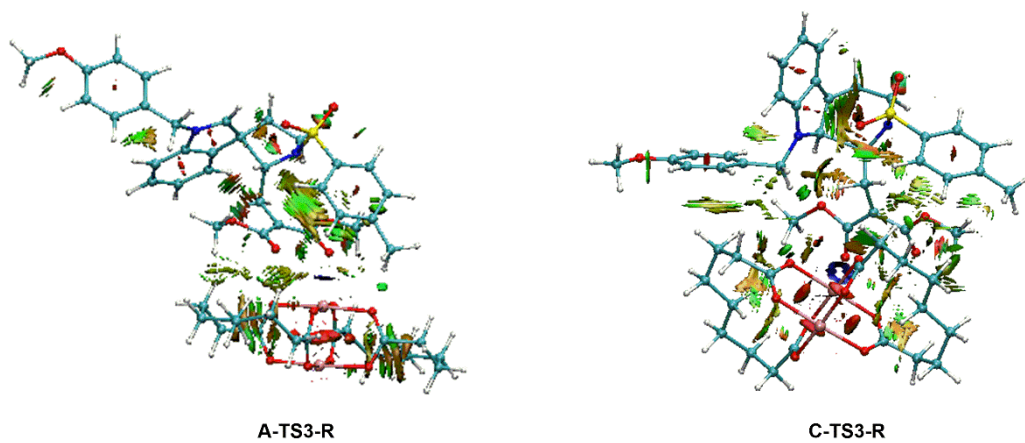
Figure S2. NCI plots for the transition states A-TS3-R and C-TS3-R .
