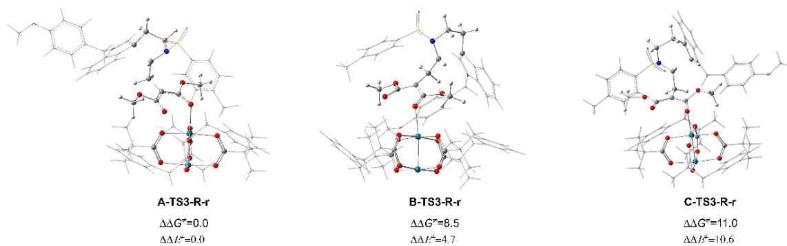
Figure S1. Geometric structures of transition states as well as the free energy barriers \Delta\Delta G^\ddagger and energy barriers \Delta\Delta E^\ddagger relative to the most favored path A from 1-Rh to int3 with real \text{Rh}_2(\text{esp})_2 catalyst (energies are given in kcal/mol).
