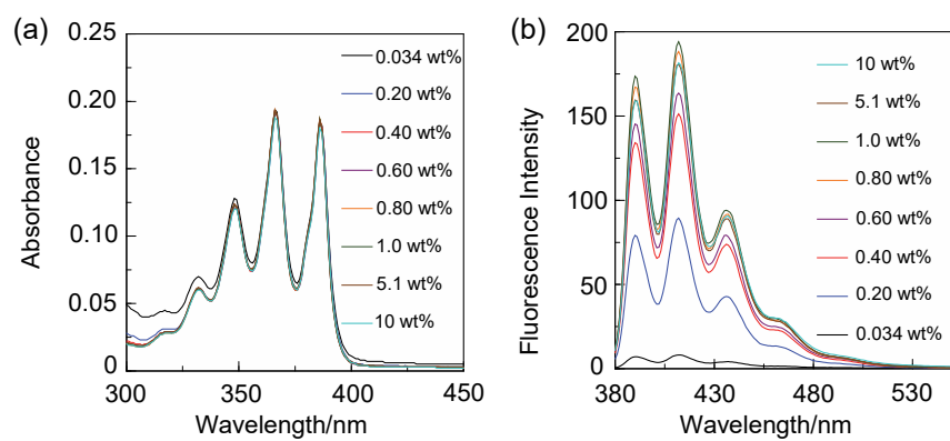
Fig. S1 (a) Absorption and (b) fluorescence spectra ( \lambda^{\text{ex}} = 366 \text{ nm} ) of OF-2 ( 2.0 \times 10^{-5} \text{ M} ) in acetonitrile containing water (0.034–10 wt%).
