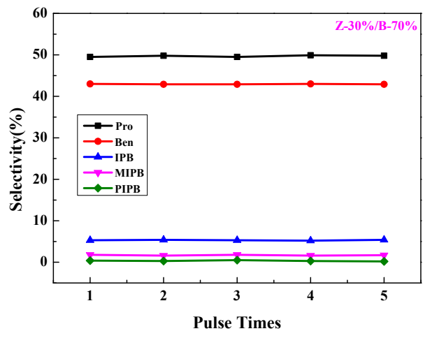
Fig.S1 Selectivities of each product over the Z-x/B-y samples at different pulse times.
