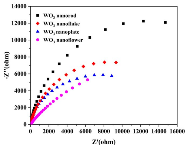
Fig. S1 EIS Nyquist plots of the WO 3 arrays.
