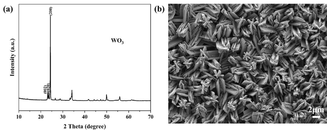
Fig. S2 (a) XRD patterns and (b) FESEM image of the WO 3 nanoflower arrays after the photocatalytic and photoelectrocatalytic reaction.
