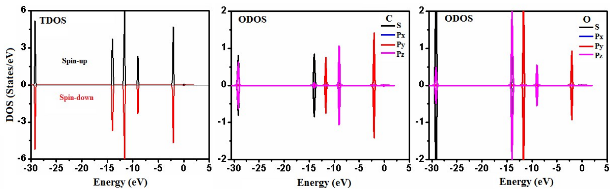
Figure S4: Spin-polarized total and orbital resolved density of states for isolated CO molecule
