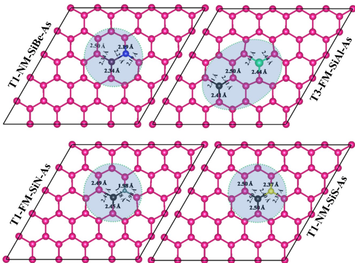
Figure S3: Bond lengths around the doped sites
