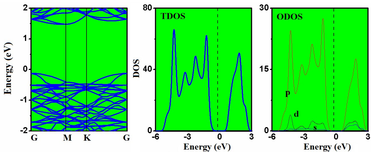
Figure S1: Computed GGA/PBE based electronic band structure and density of states for 5x5 supercell pristine arsenene
