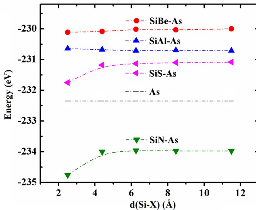
Figure S2: Total energy comparison in various doping systems
