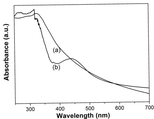
Fig. S1. UV-Vis absorption spectra of (a) N-TiO 2 and (b) P25-TiO 2 /Ag samples.
