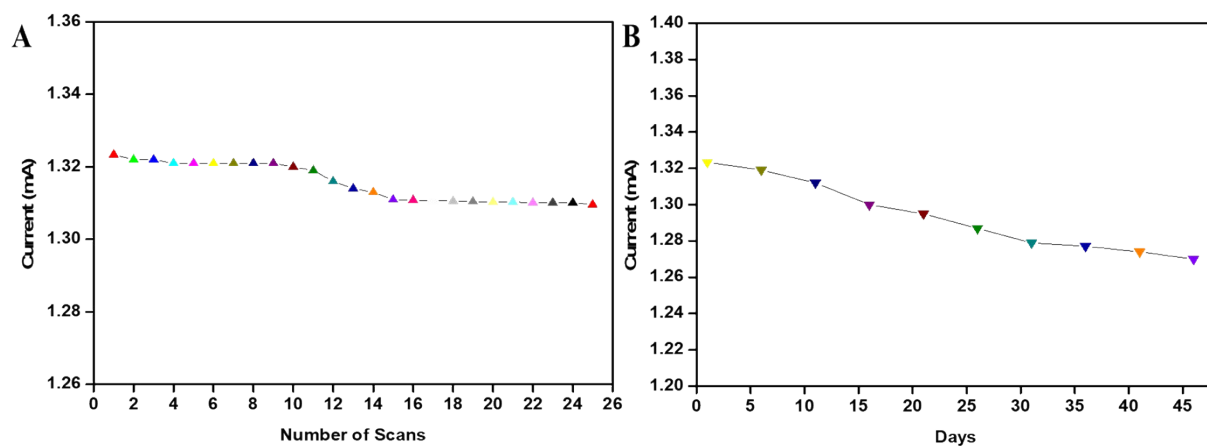
Supp. Figure 1 bT-ZnO/ITO electrodes: A) Reproducibility/reusability study and B) Stability/durability study up to 46 days at interval of 5 days.
