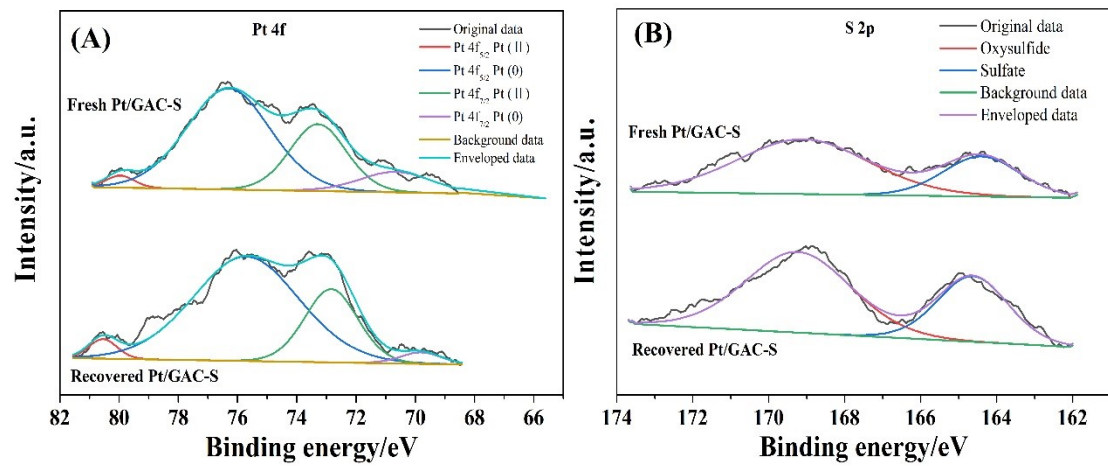
Fig. S1. (A) Pt 4f XPS spectra of the fresh Pt/GAC-S catalyst and the recovered Pt/GAC-S catalyst;
