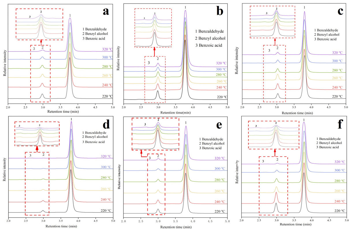
Figure S1: Liquid chromatogram of products from selective oxidation of benzyl alcohol at different temperatures over MoVO x catalysts with different doping ratio of Ce. Ce-0 (a), Ce-0.02 (b), Ce-0.05 (c), Ce-0.10 (d), Ce-0.20 (e) and Ce-0.33 (f)
