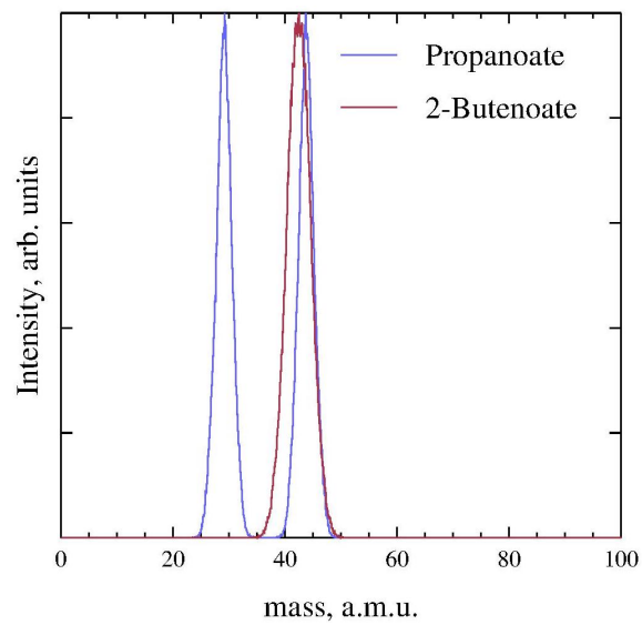
Figure S1: The fragment mass spectrum of propanoate and 2-butenate.
