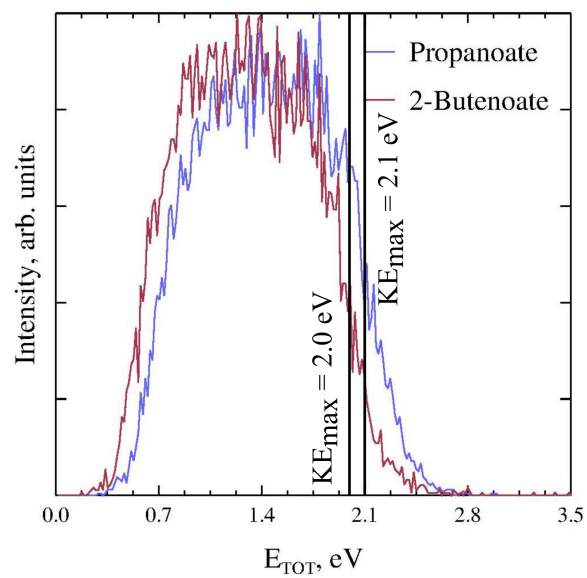
Figure S2: The total energy ( E_{\text{TOT}} ) spectrum of propanoate and 2-butenate.
