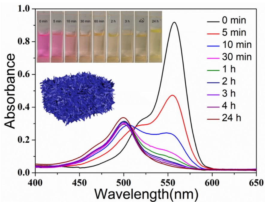
Fig. S1. UV-Vis spectra of RhB degradation by pure MnO 2 particles at pH = 3.5
