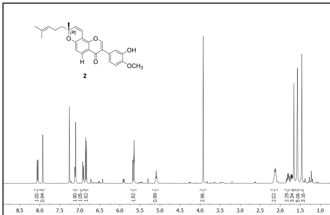
Figure S8. 1 H NMR spectrum of dalpulapan B ( 2 )
