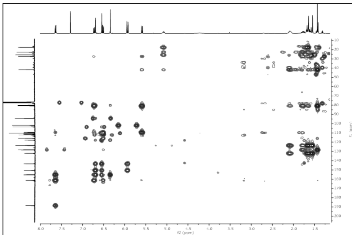
Figure S33. HMBC spectrum of dalpulapan E (5)
