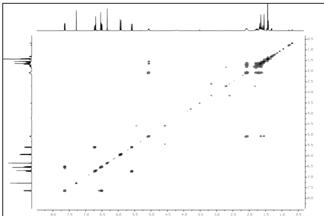
Figure S31. ^1\text{H} - ^1\text{H} COSY spectrum of dalpulapan E (5)
