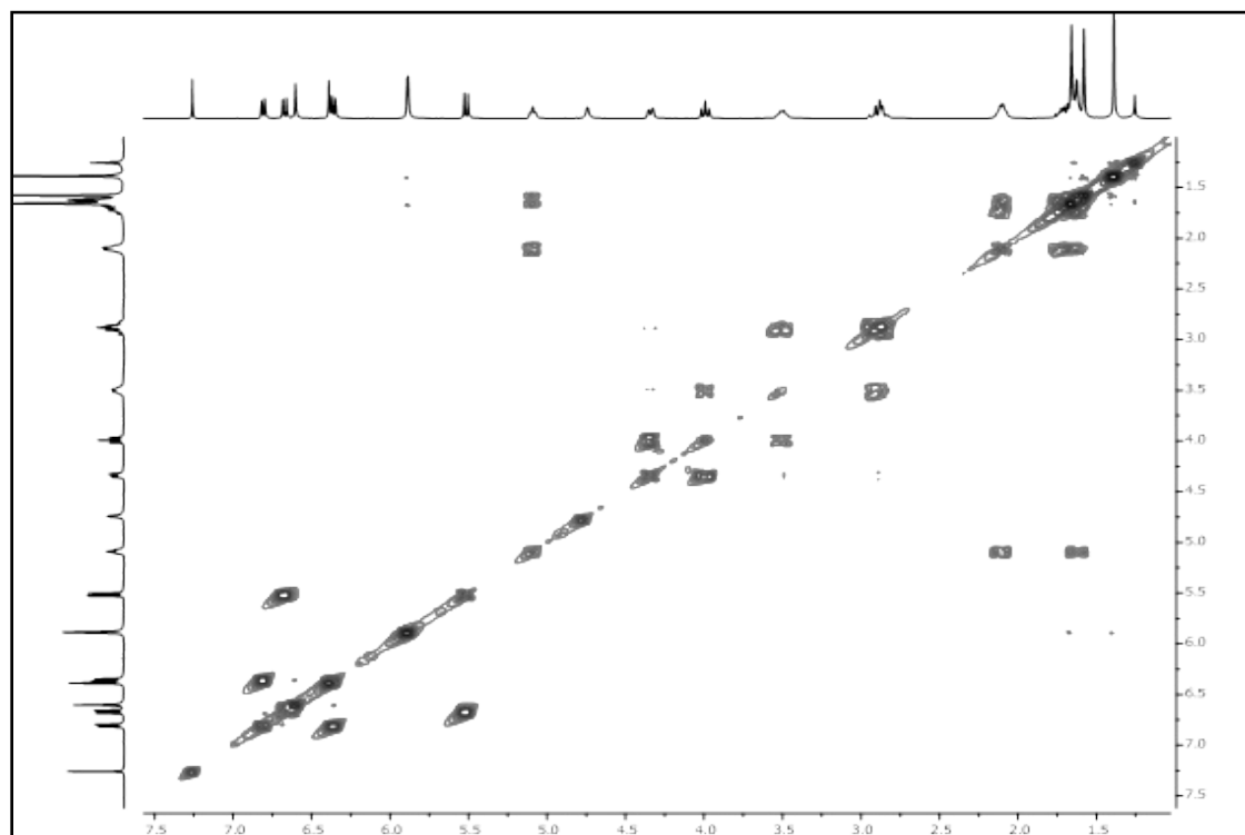
Figure S24. ^1\text{H} - ^1\text{H} COSY spectrum of dalpulan D (4)
