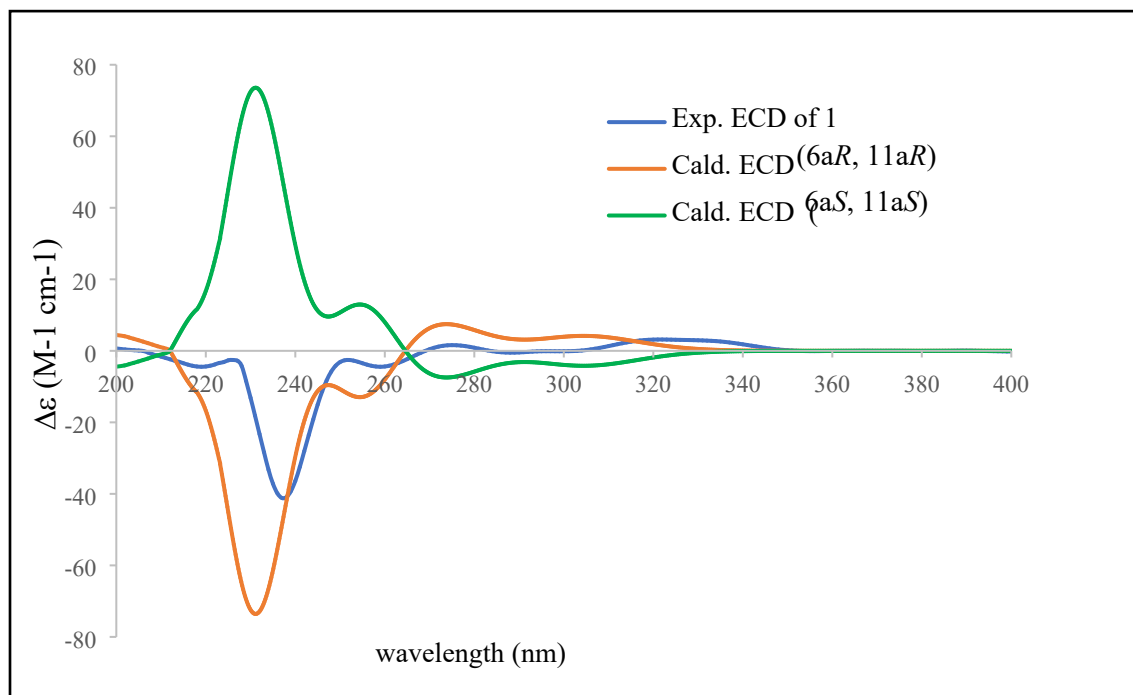
Figure S7. ECD spectrum of dalpulapan A ( 1 )
