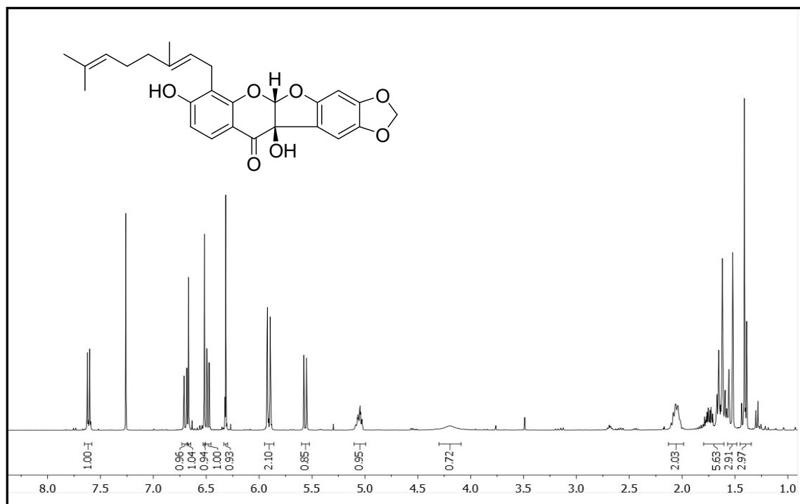
Figure S29. 1 H NMR spectrum of dalpulapan E (5)
