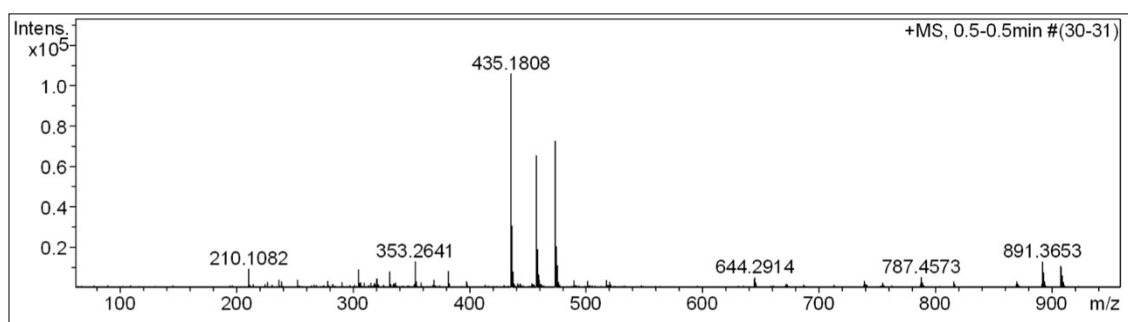
Figure S20. MS spectrum of dalpulapan C ( 3 )
