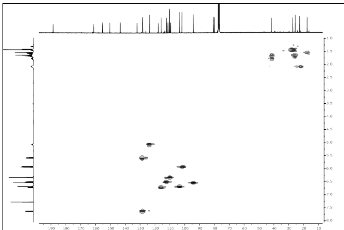
Figure S32. HMQC spectrum of dalpulapan E (5)
