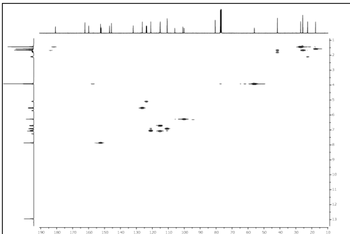
Figure S18. HMQC spectrum of dalpulan C ( 3 )
