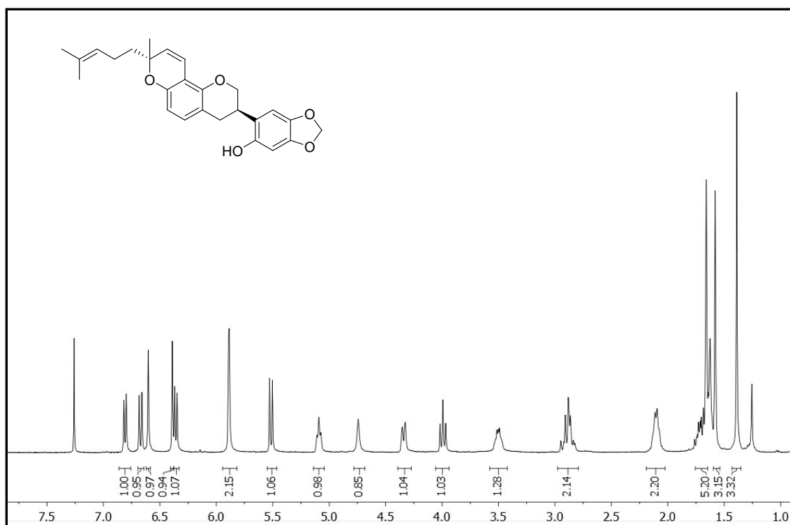
Figure S22. ^1\text{H NMR} spectrum of dalpulan D (4)
