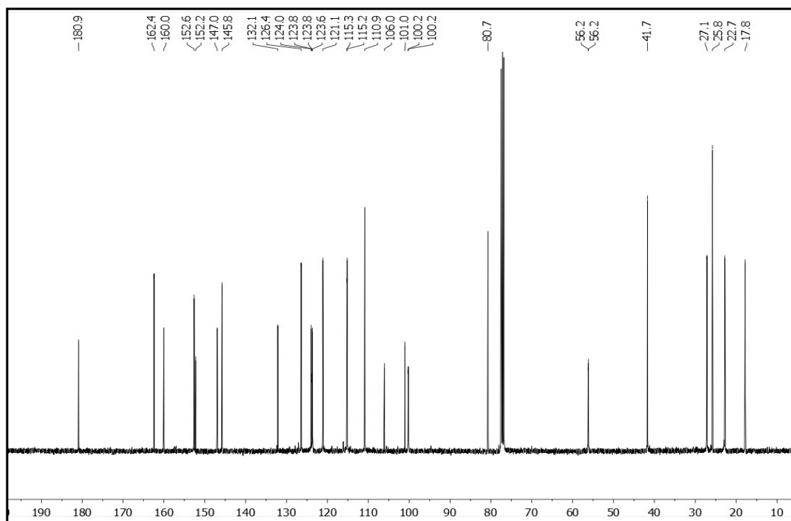
Figure S16. 13 C NMR spectrum of dalpulapan C (3)
