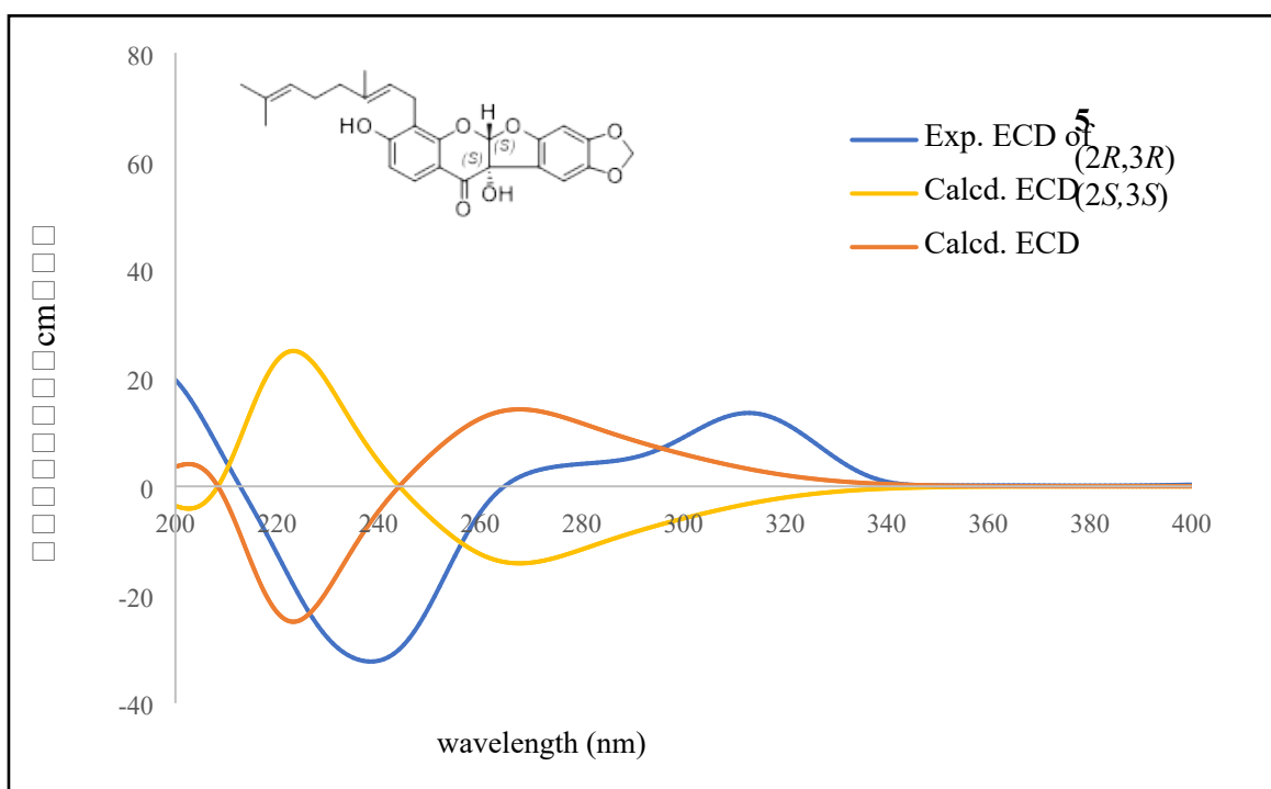
Figure S36. Calculated ECD spectrum of (2 R ,3 R and 2 S ,3 S ) derivatives of 5
