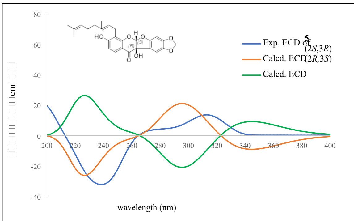
Figure S35. Experimental and calculated ECD spectrum of (2 S ,3 R ) dalpulan E ( 5 )
