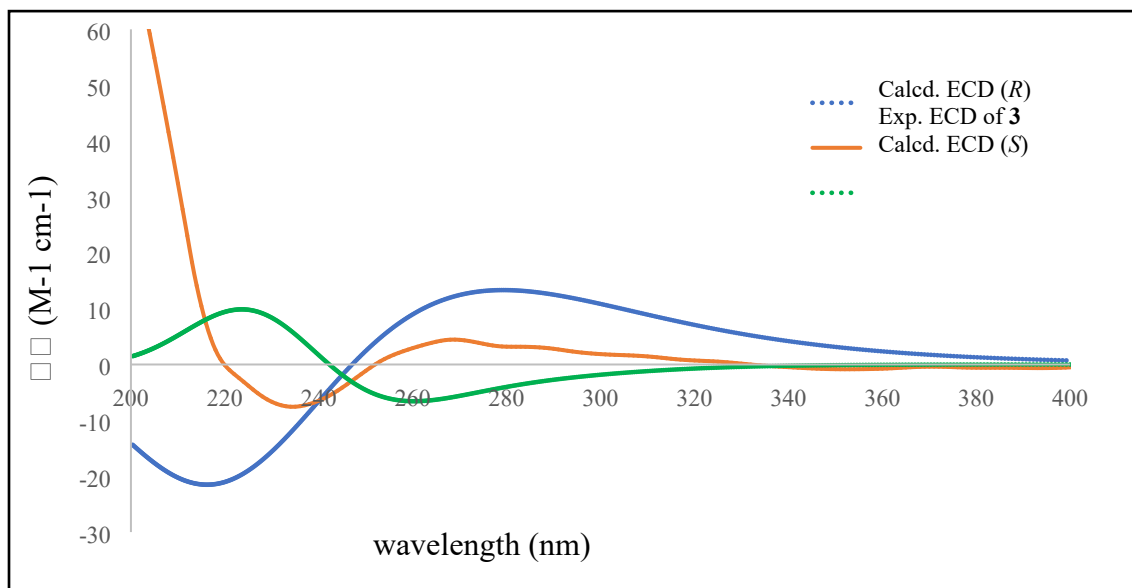
Figure S21. ECD spectrum of dalpulan C (3)
