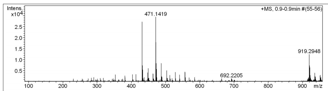
Figure S34. MS spectrum of dalpulapan E (5)
