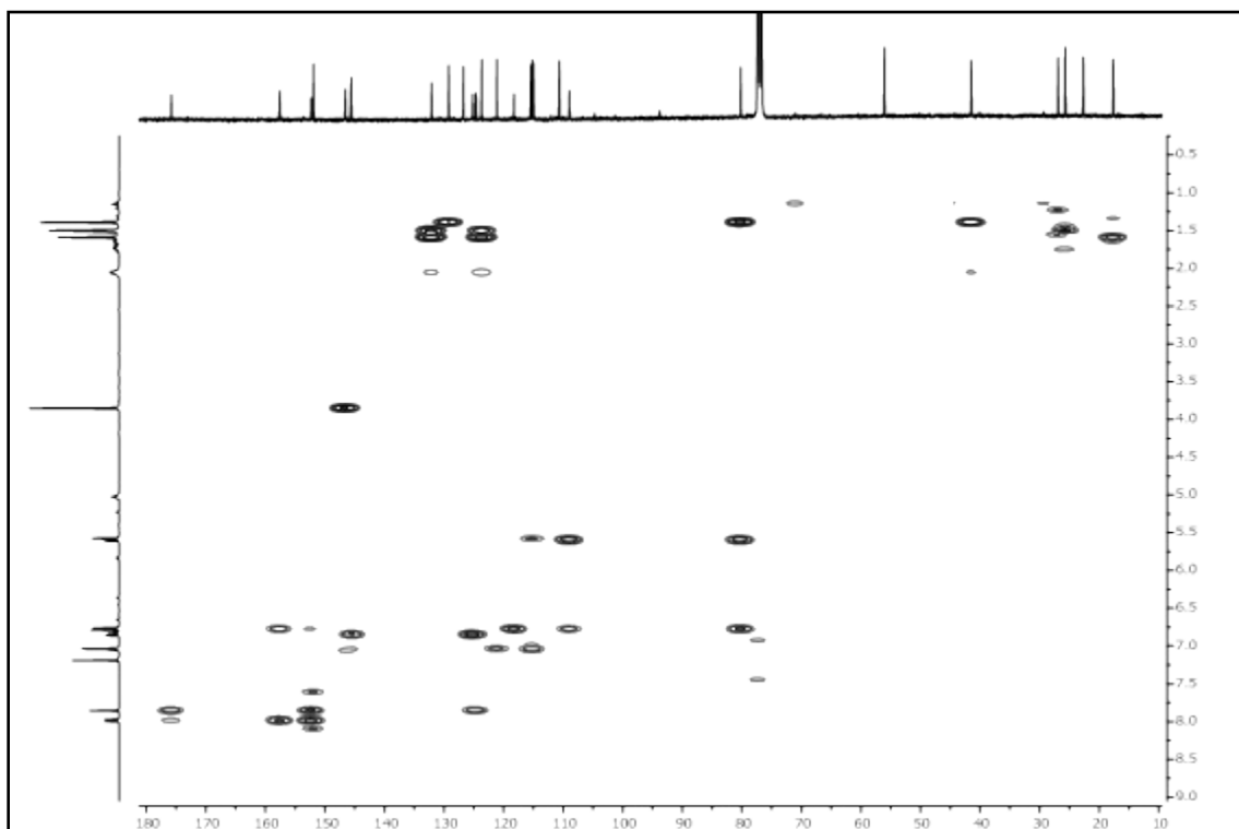
Figure S12. HMBC spectrum of dalpulapan B (2)
