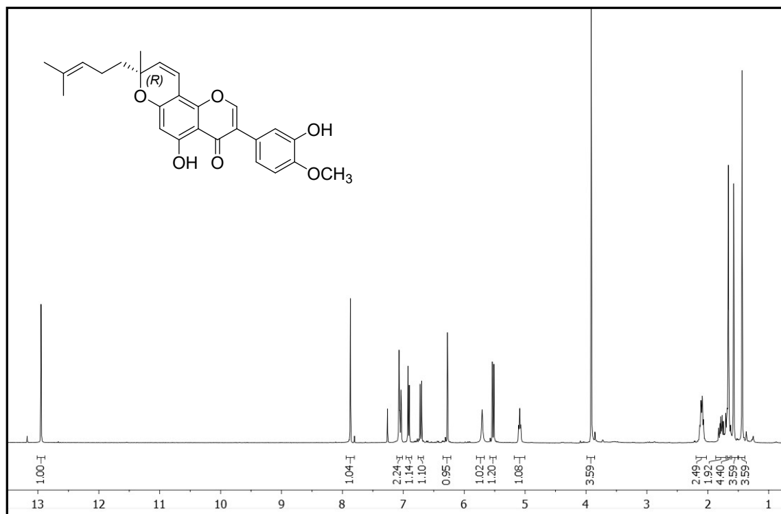
Figure S15. 1 H NMR spectrum of dalpulapan C (3)
