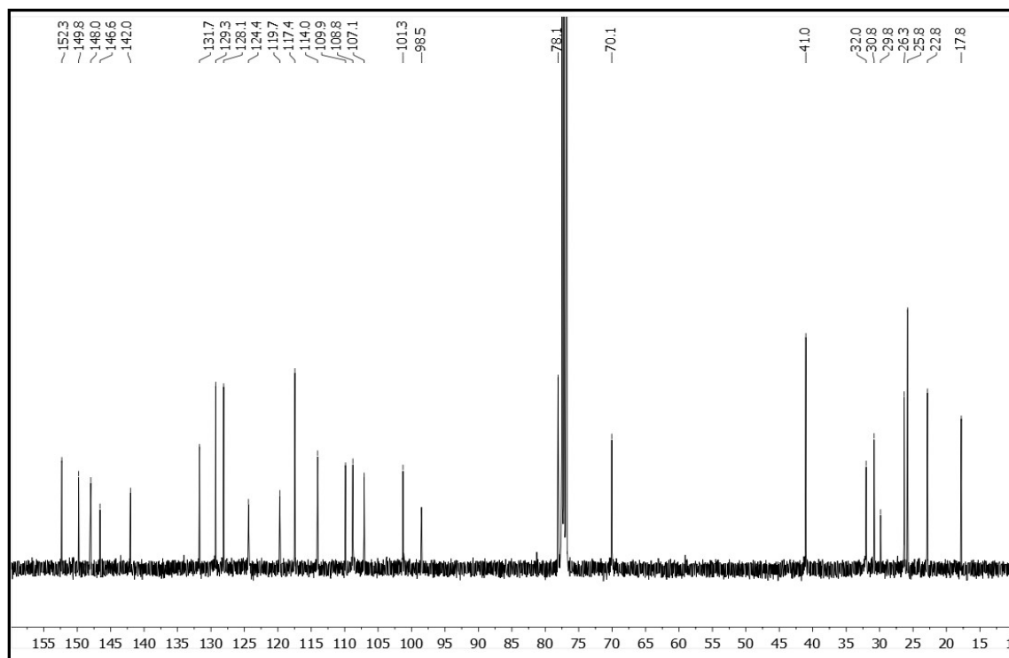
Figure S23. ^{13}\text{C} NMR spectrum of dalpulan D (4)
