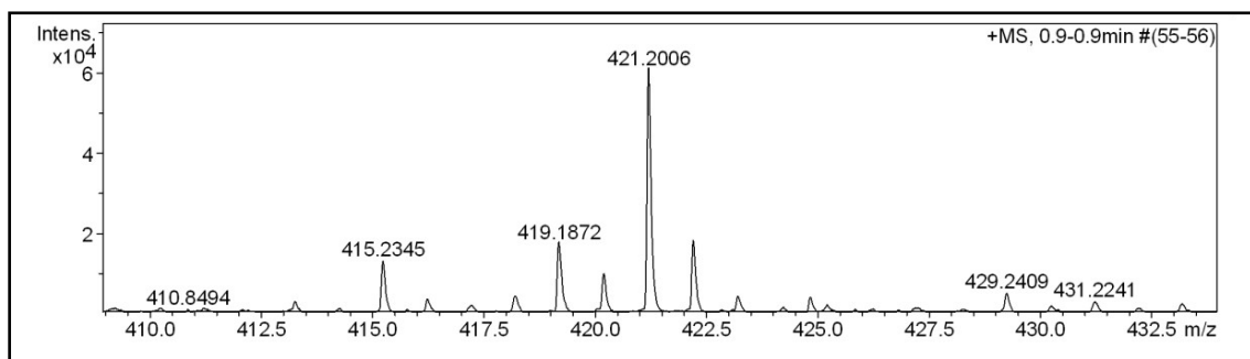
Figure S27. MS spectrum of dalpulapan D (4)
