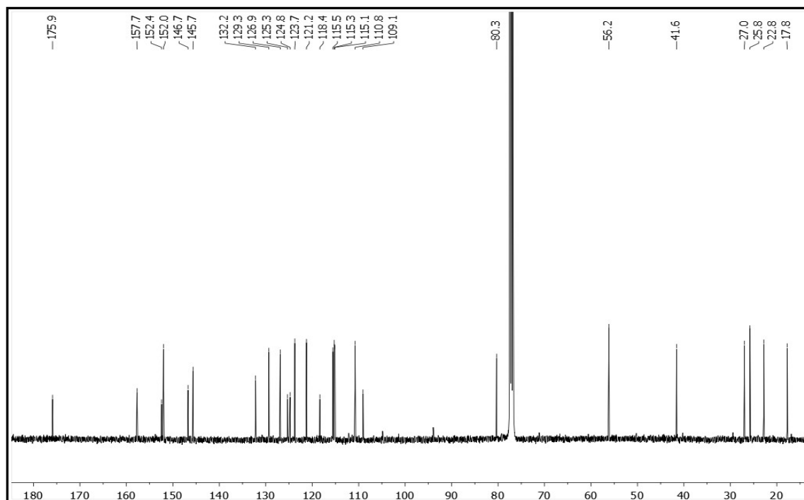
Figure S9. ^{13}\text{C} NMR spectrum of dalpulan B (2)
