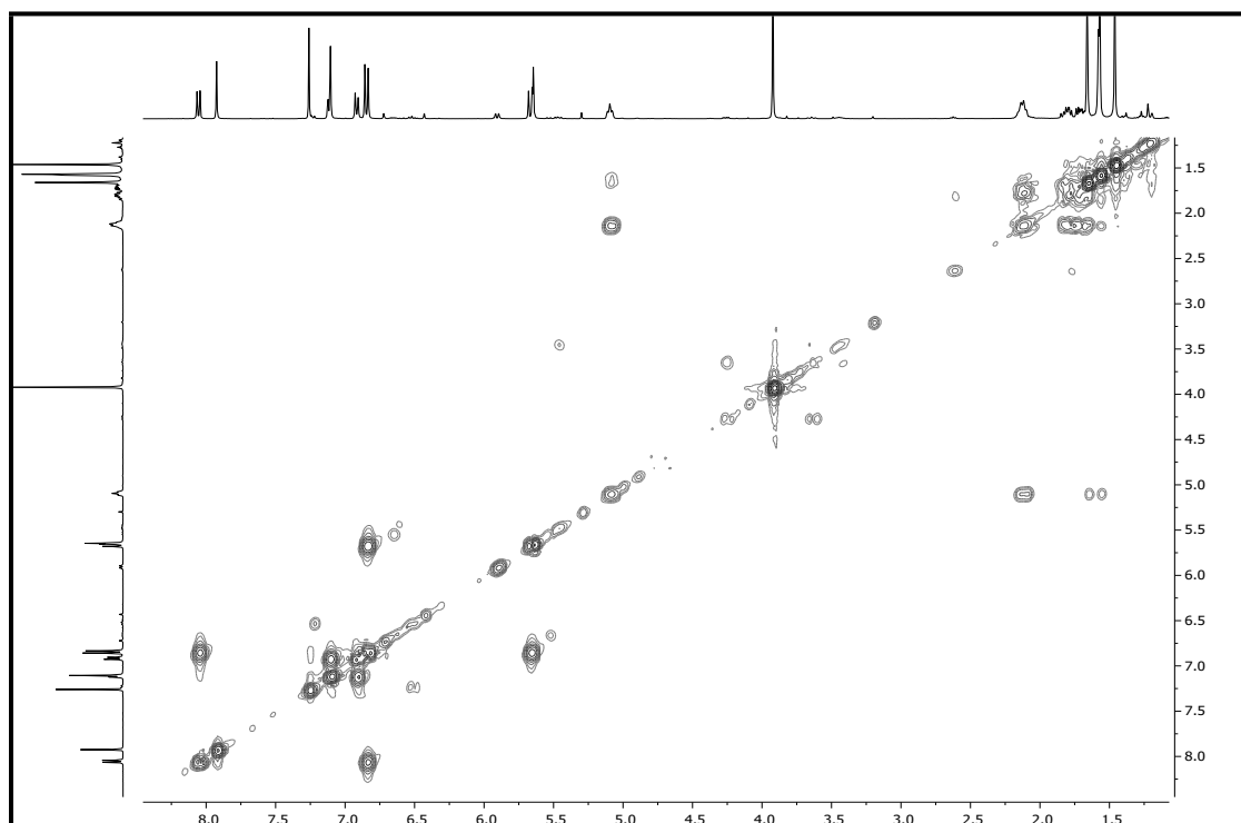
Figure S10. ^1\text{H} - ^1\text{H} COSY spectrum of dalpulan B (2)
