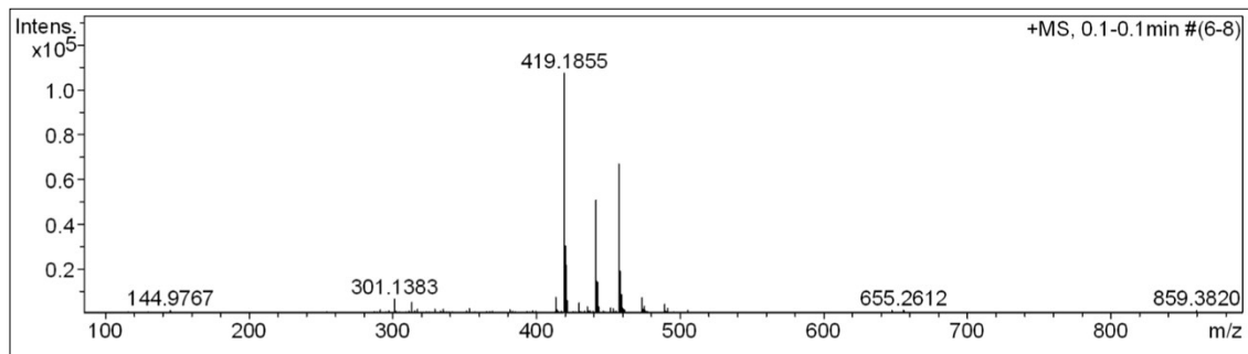
Figure S13. MS spectrum of dalpulapan B (2)
