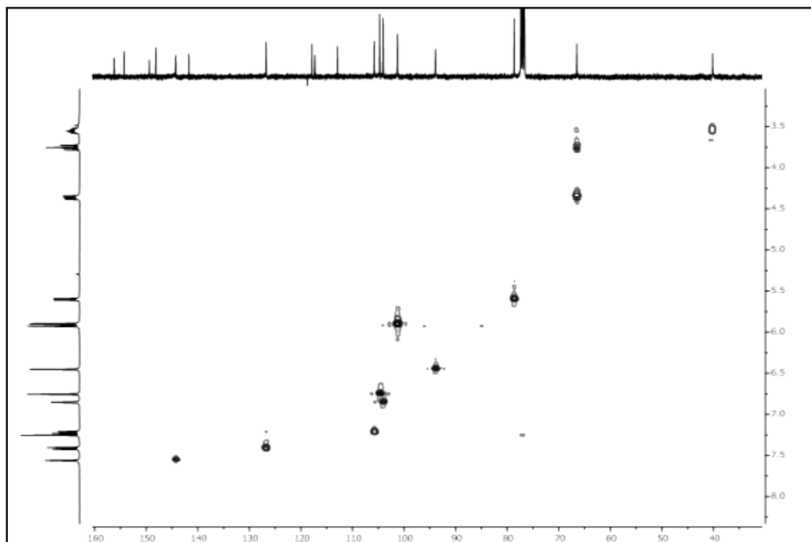
Figure S4. HMBC spectrum of dalpulapan A ( 1 )
