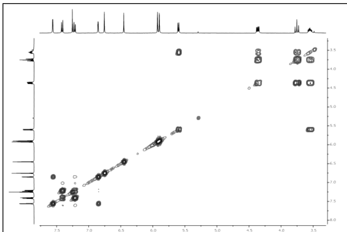
Figure S3. ^1\text{H} - ^1\text{H} COSY spectrum of dalpulapan A ( 1 )
