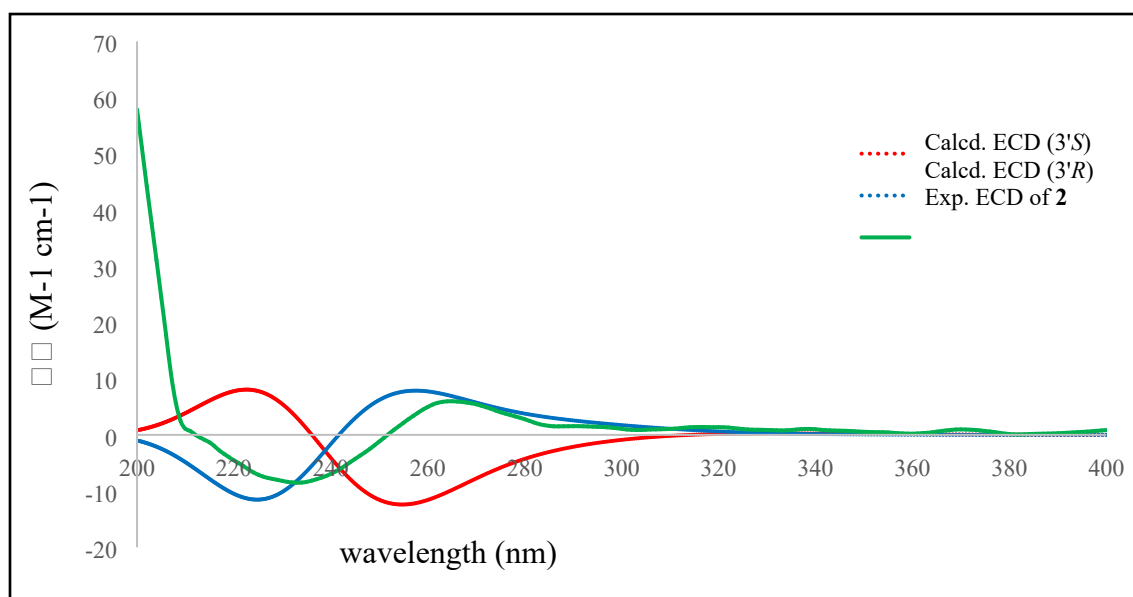
Figure S14. ECD spectrum of dalpulapan B (2)
