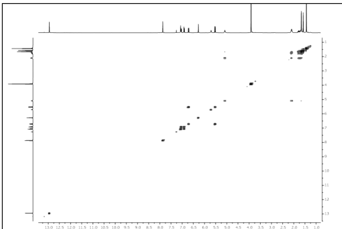
Figure S17. ^1\text{H} - ^1\text{H} COSY spectrum of dalpulan C ( 3 )
