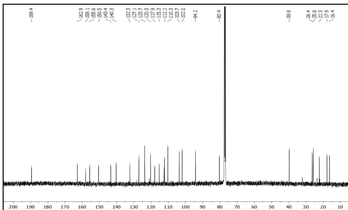
Figure S30. 13 C NMR spectrum of dalpulapan E (5)
