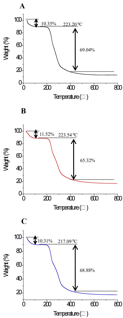
Fig.S4. TGA curves of PKP (A), PCP (B), and PSP (C).
