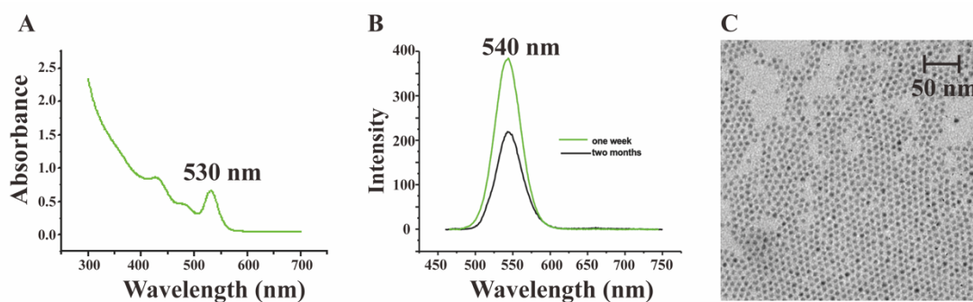
Fig. S1 Characterization of QDs. (A) UV visible spectra. (B) Fluorescence spectra at one week and two months. (C) High-resolution TEM image.
