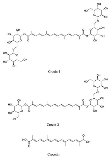
Fig. S1. The chemical structures of crocin and crocetin
