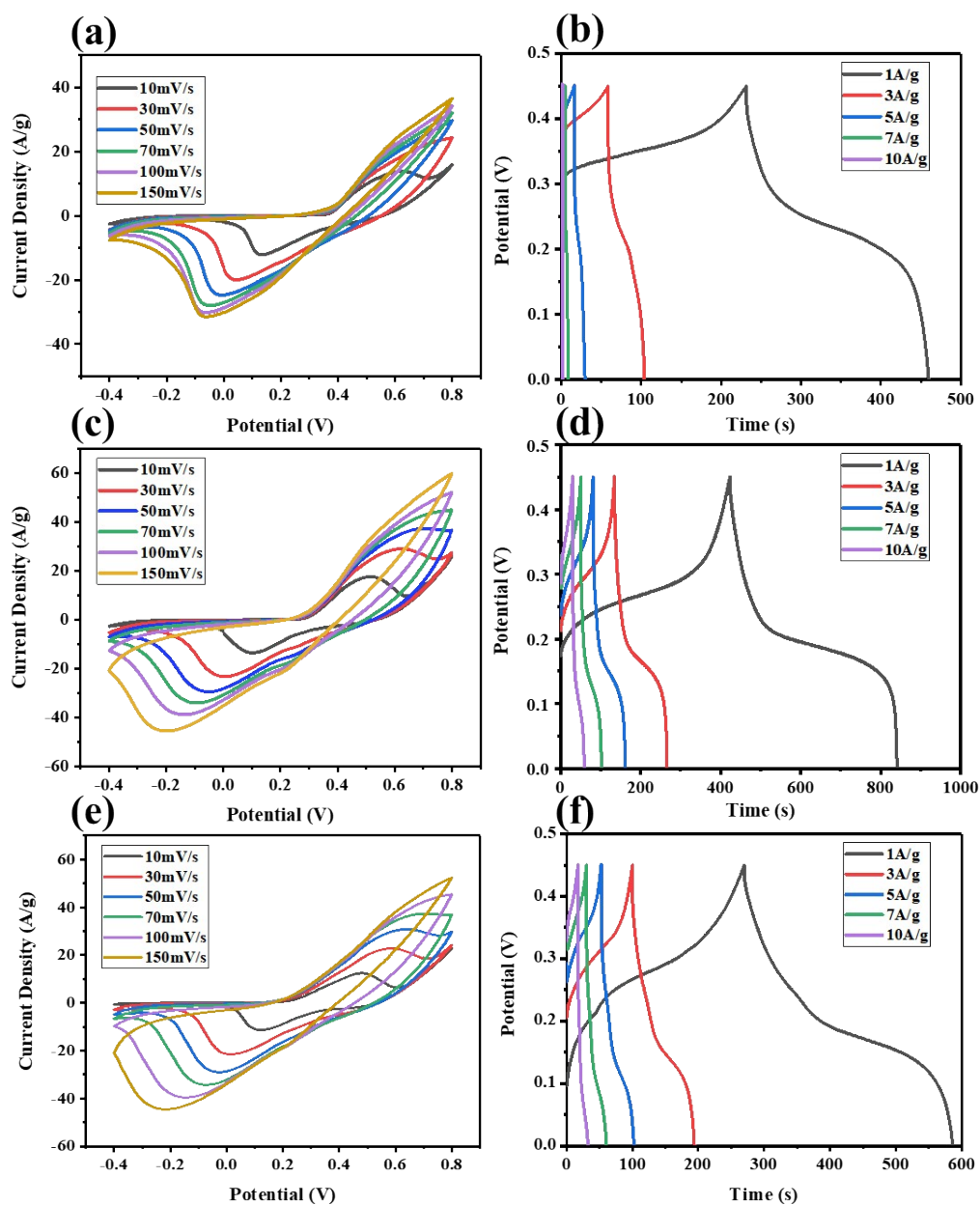
Fig. S2 Electrochemical performances in 1 M KOH solution. CV curves at various scan rate from 10 to 150 mV/s, and GCD curves at different current densities from 1 to 10 A/g of NiCo MOF-0 (a-b), NiCo MOF-2 (c-d) and NiCo MOF-4 (e-f).
