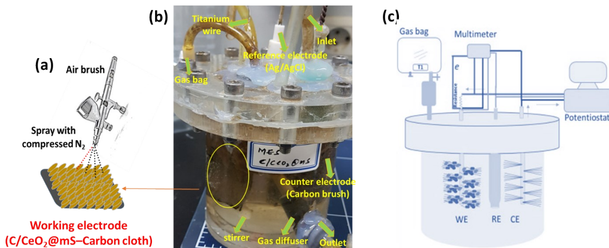
Fig. S1 (a) Coating of catalyst ink over carbon cloth with air brush (b) Image of MES reactor (c) MES control operation diagram
