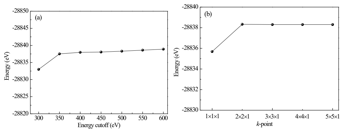
Fig. S1. Variation in energy of CaO (100) surface as a function of energy cutoff (a) and k -point (b).
