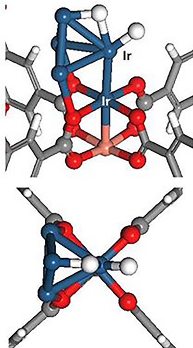
(c) Ir cluster + Ir-Cu-BTC
