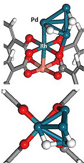
(a) Pd cluster + Rh-Cu-BTC
