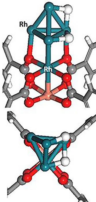
(b) Rh cluster + Rh-Cu-BTC
