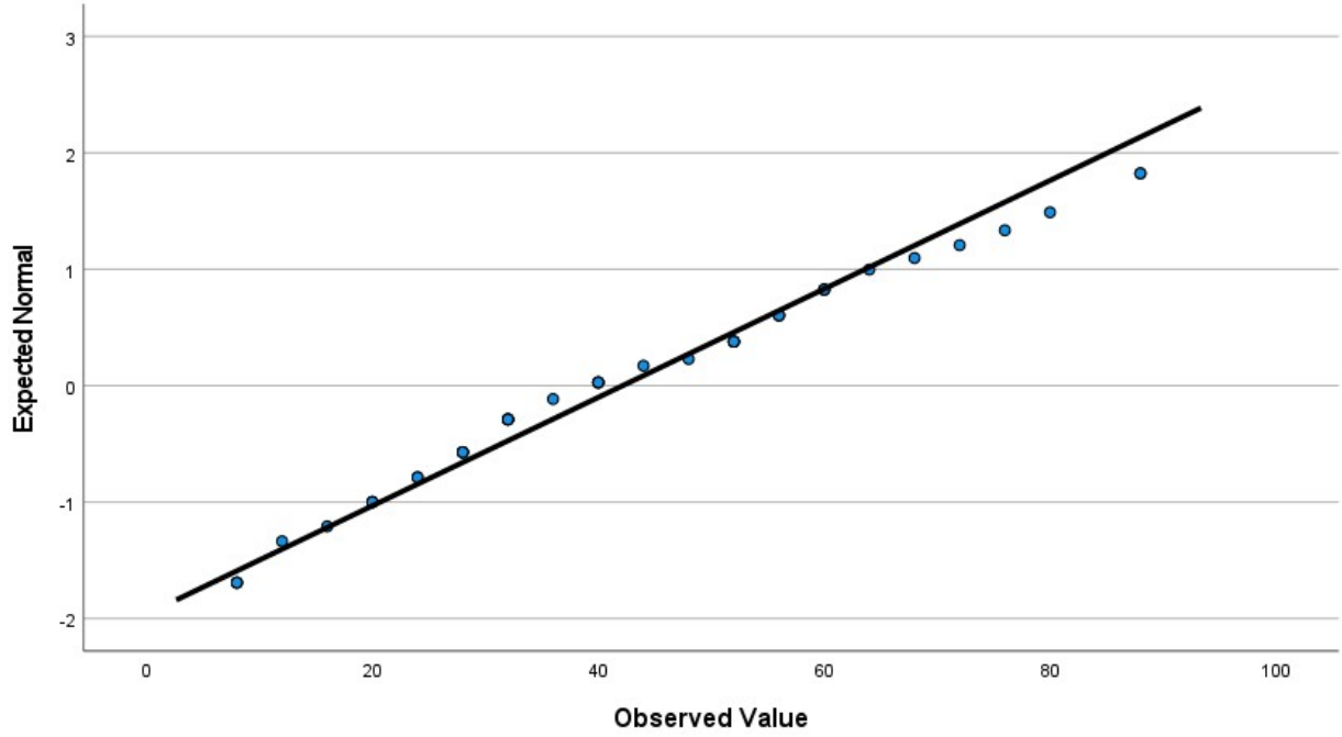
Normal Q-Q Plot of Low_stakes_closed_sort_Match_expert_fig6
