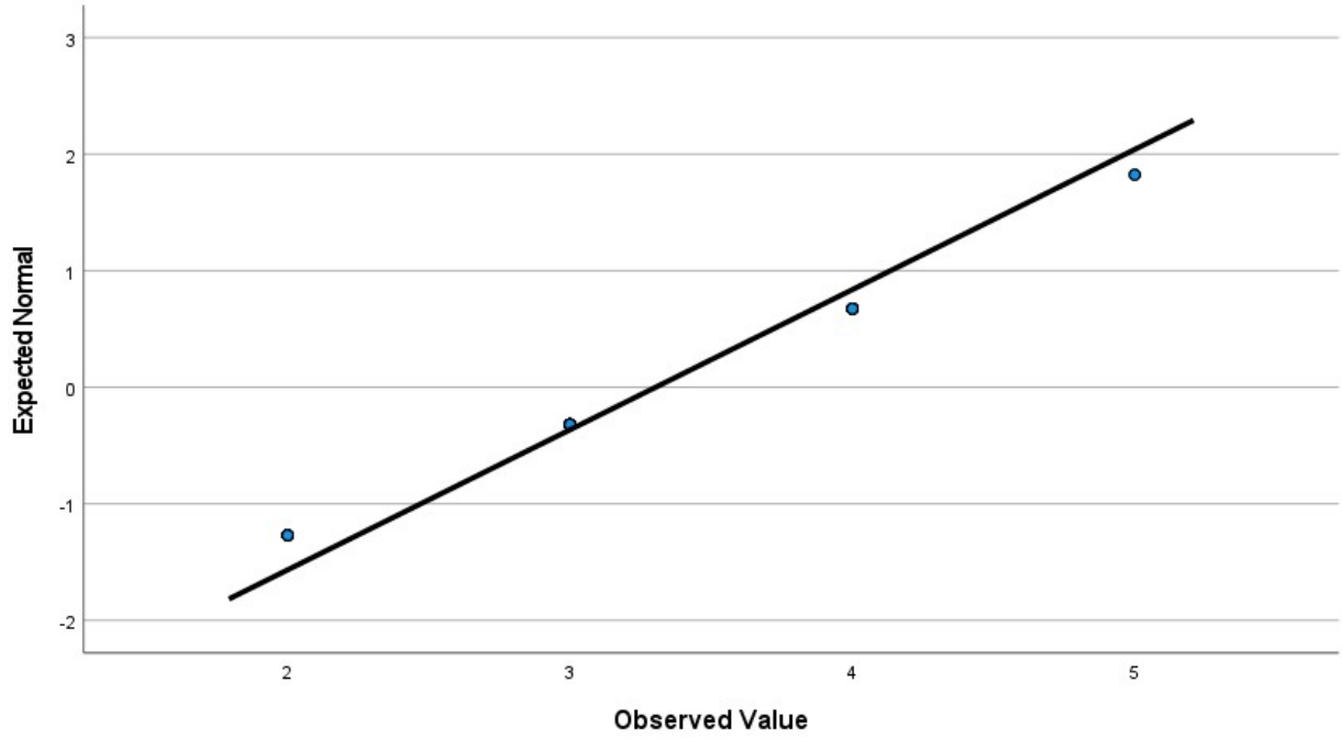
Normal Q-Q Plot of Exam_Match_Expert_fig6
