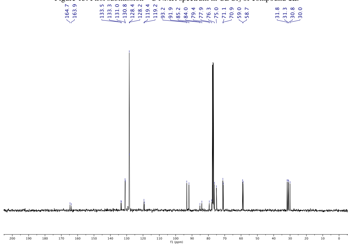
Figure 16. New submission 13 C NMR spectrum in CDCl 3 of compound 1h .
