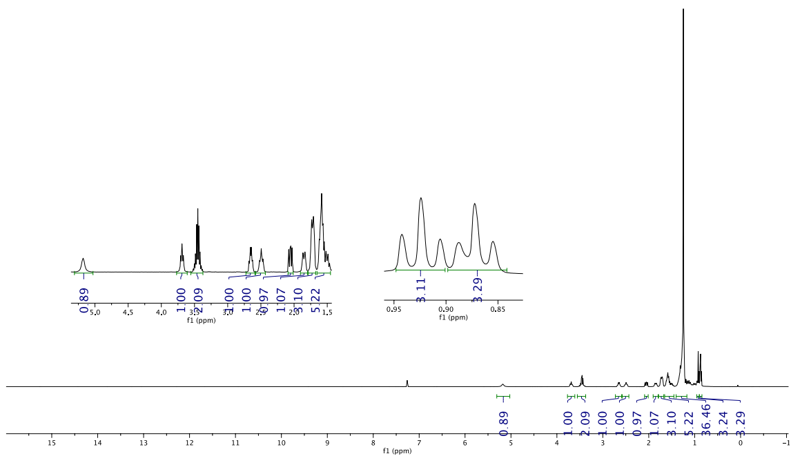
Figure 50. New submission 1 H NMR spectrum in CDCl 3 of compound 2aj .
