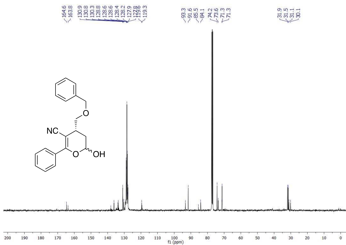
Figure 7. First submission 13 C NMR spectrum in CDCl 3 of compound 1f .
