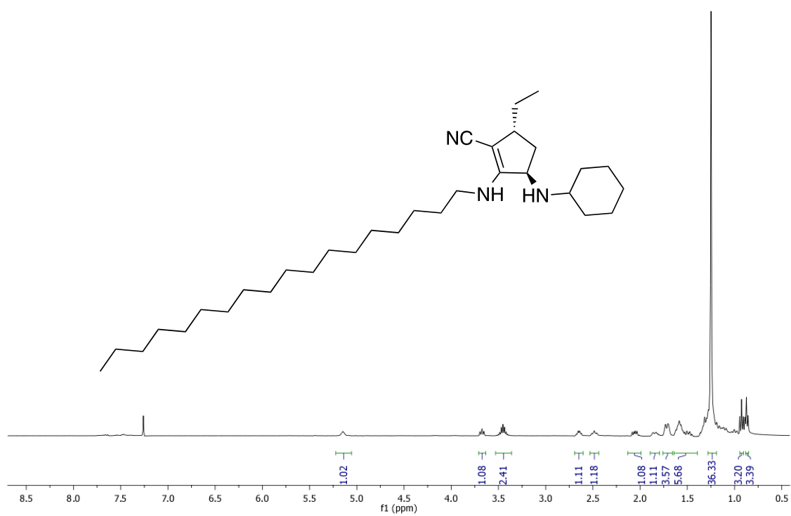
Figure 49. First submission 1 H NMR spectrum in CDCl 3 of compound 2aj .
