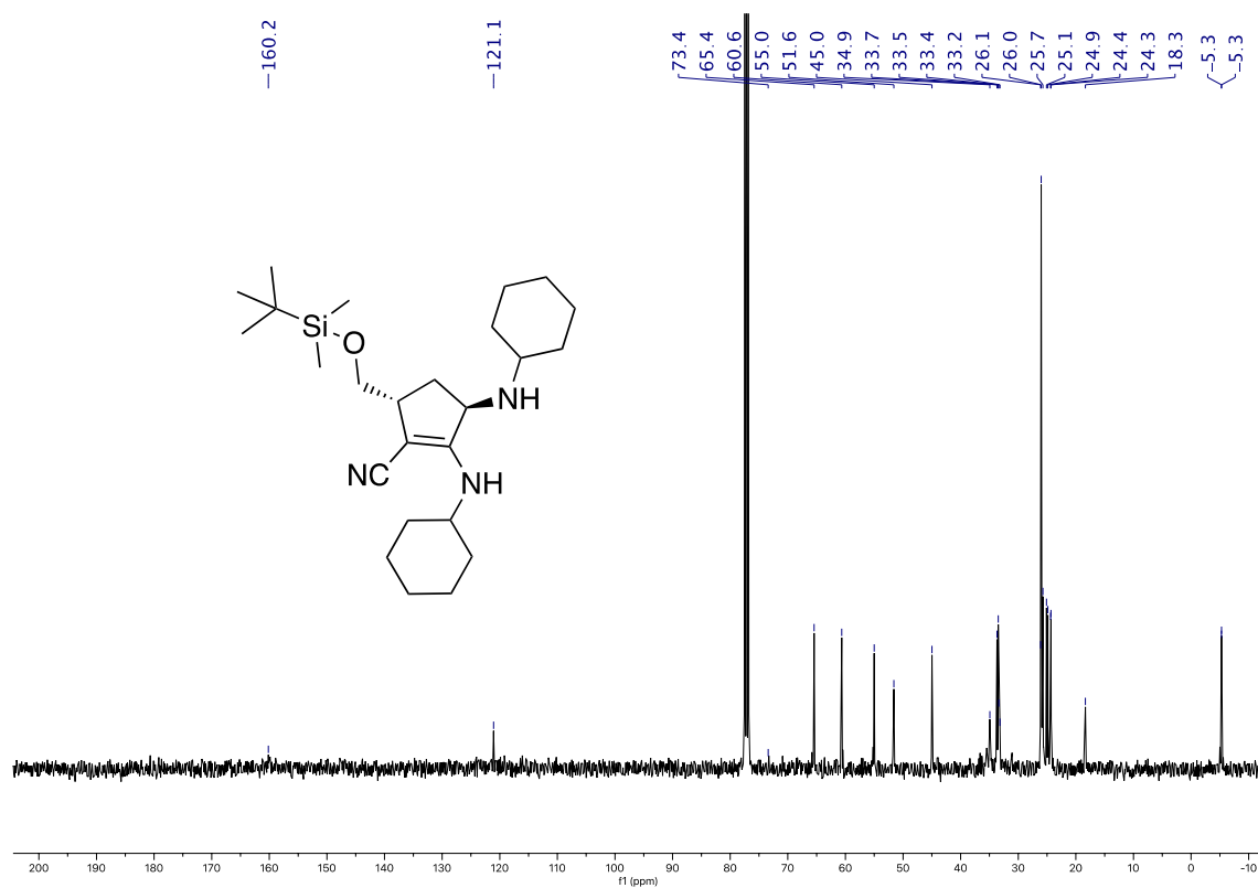
Figure 43. First submission 13 C NMR spectrum in CDCl 3 of compound 2ag .
