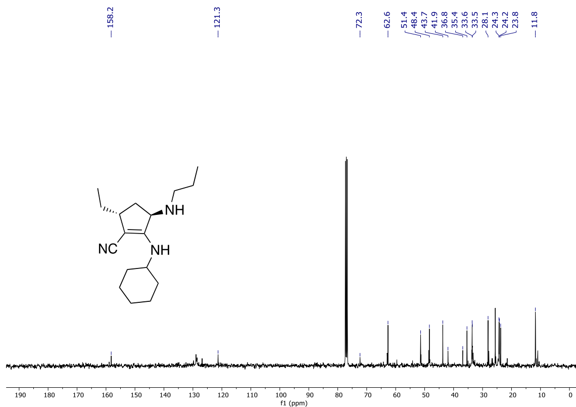
Figure 31. First submission 13 C NMR spectrum in CDCl 3 of compound 2g .
