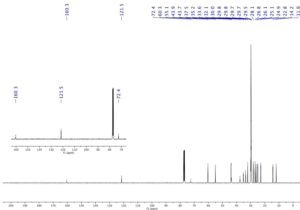
Figure 52. New submission 13 C NMR spectrum in CDCl 3 of compound 2aj .
