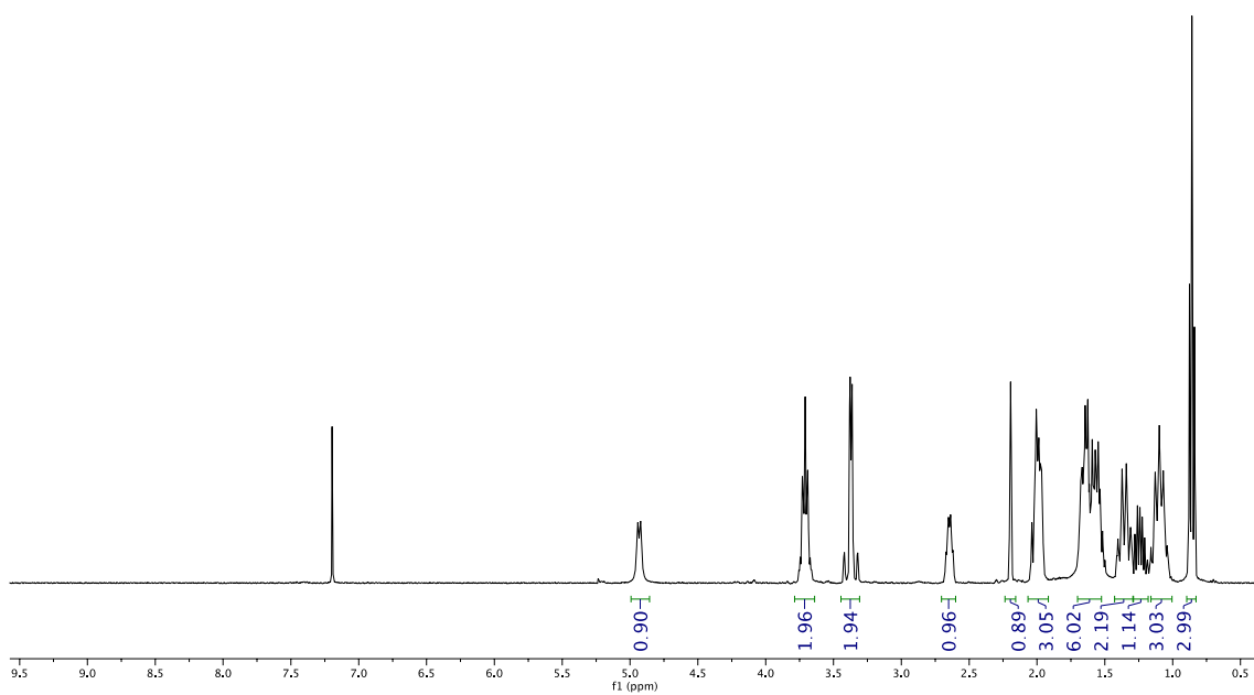
Figure 22. New submission 1 H NMR spectrum in CDCl 3 of compound 2e .
