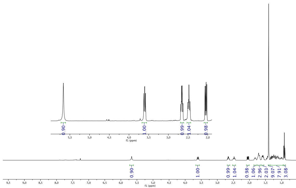
Figure 46. New submission 1 H NMR spectrum in CDCl 3 of compound 2ai .
