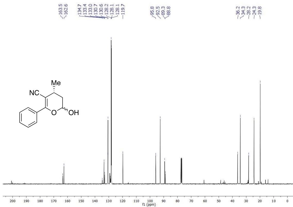
Figure 3. First submission 13 C NMR spectrum in CDCl 3 of compound 1b .
