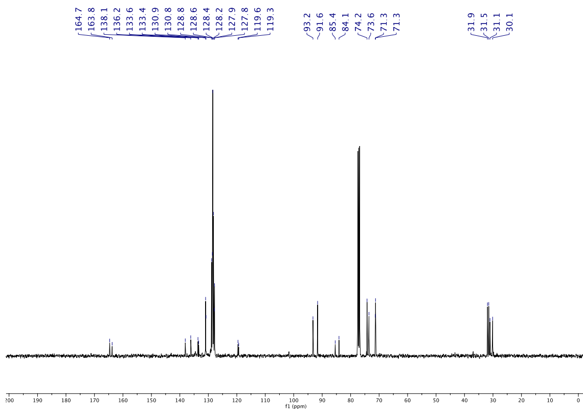
Figure 8. New submission 13 C NMR spectrum in CDCl 3 of compound 1f .
