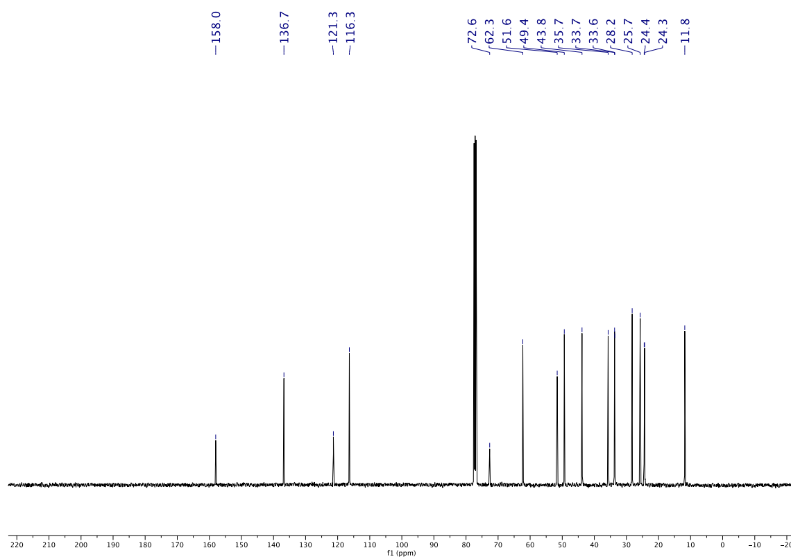
Figure 28. New submission 13 C NMR spectrum in CDCl 3 of compound 2f .
