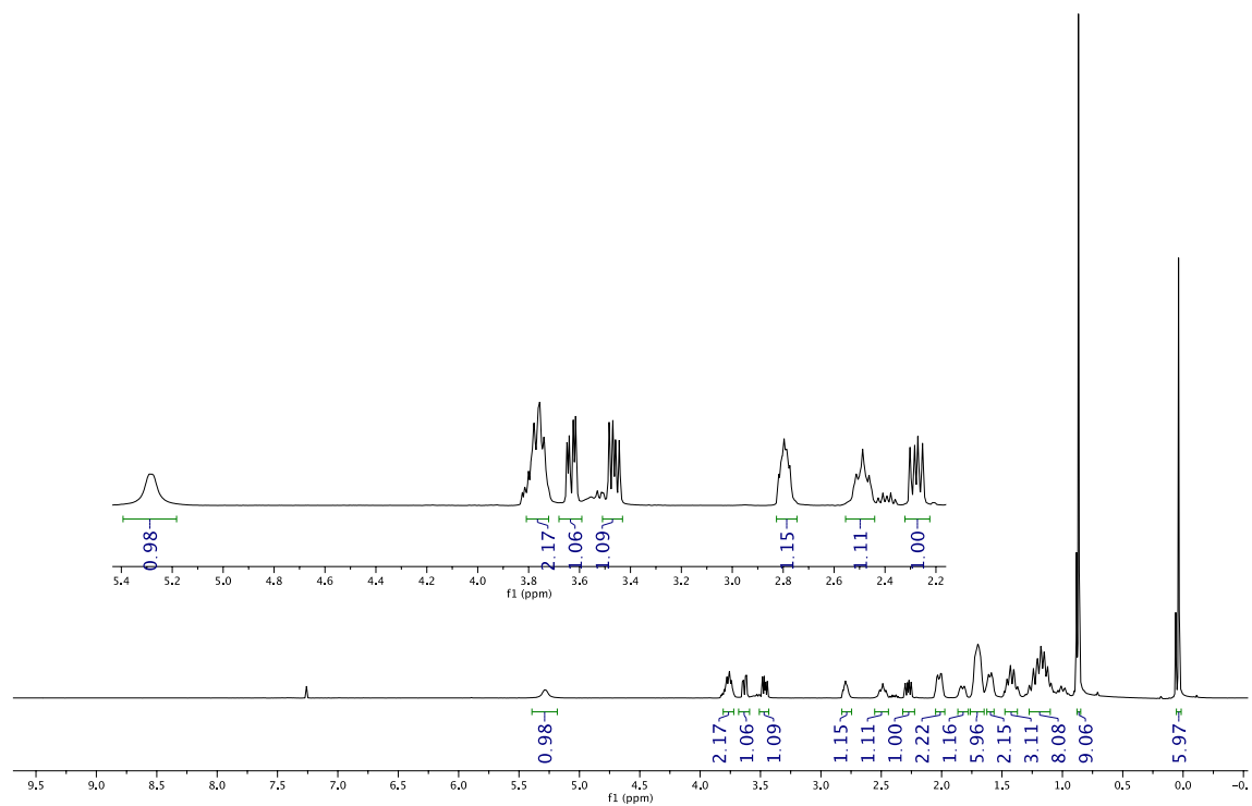
Figure 42. New submission 1 H NMR spectrum in CDCl 3 of compound 2ag .
