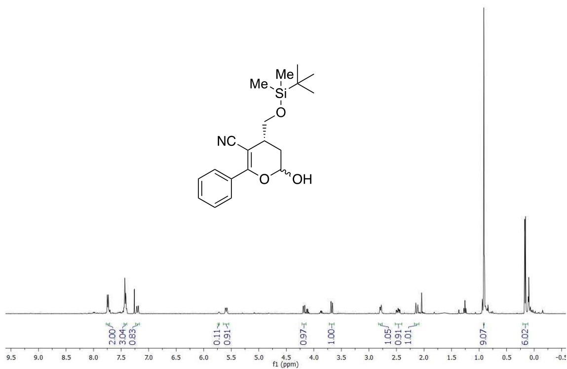
Figure 9. First submission 1 H NMR spectrum in CDCl 3 of compound 1g .
