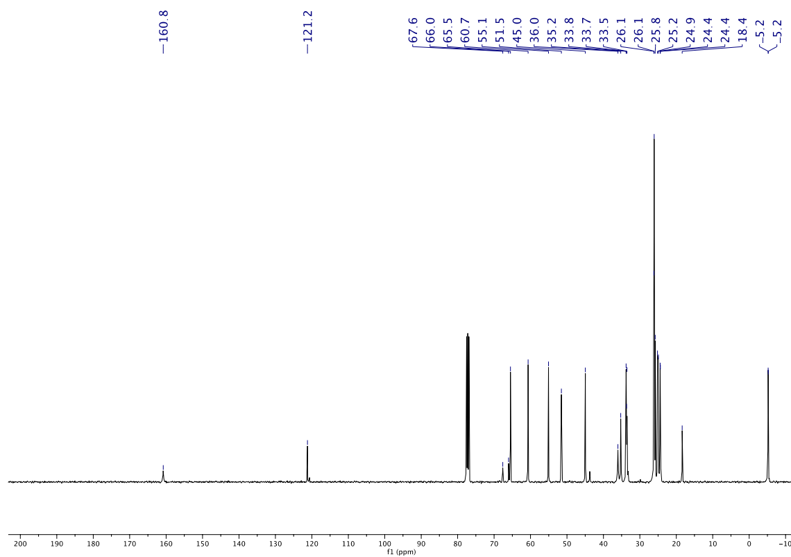
Figure 44. New submission 13 C NMR spectrum in CDCl 3 of compound 2ag .
