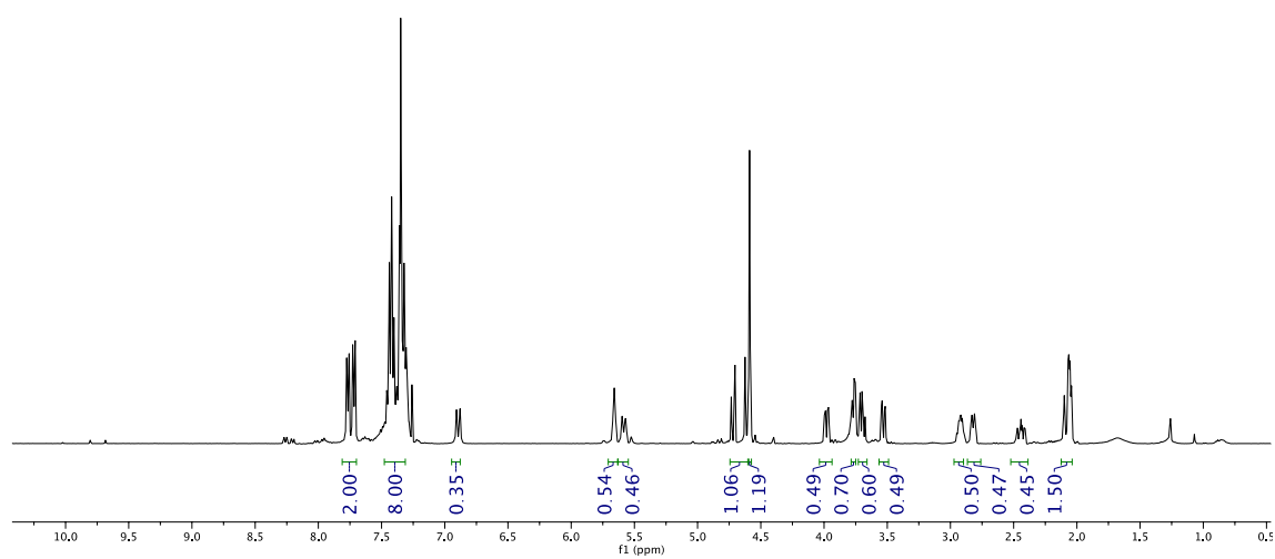
Figure 6. New submission 1 H NMR spectrum in CDCl 3 of compound 1f .
