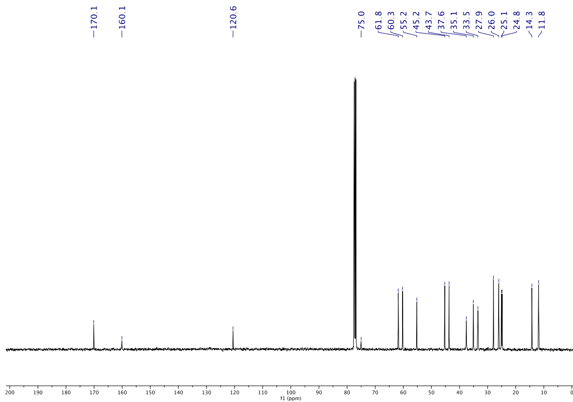
Figure 56. New submission 13 C NMR spectrum in CDCl 3 of compound 2ak .
