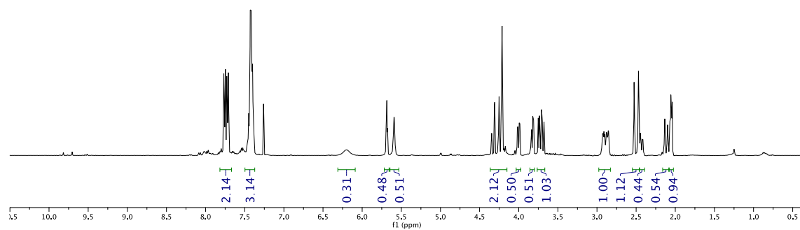
Figure 14. New submission 1 H NMR spectrum in CDCl 3 of compound 1h .
