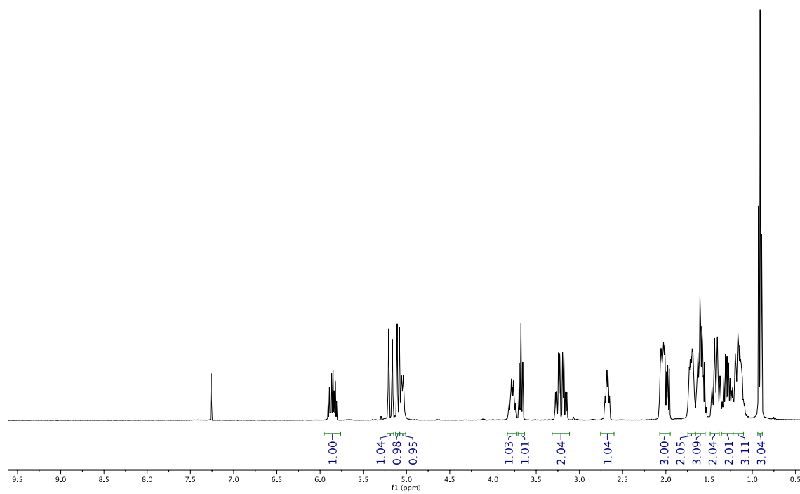
Figure 26. New submission 1 H NMR spectrum in CDCl 3 of compound 2f .
