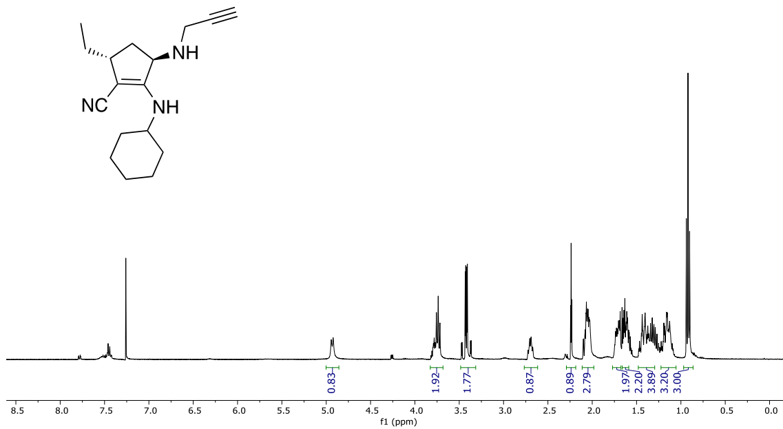
Figure 21. First submission 1 H NMR spectrum in CDCl 3 of compound 2e .
