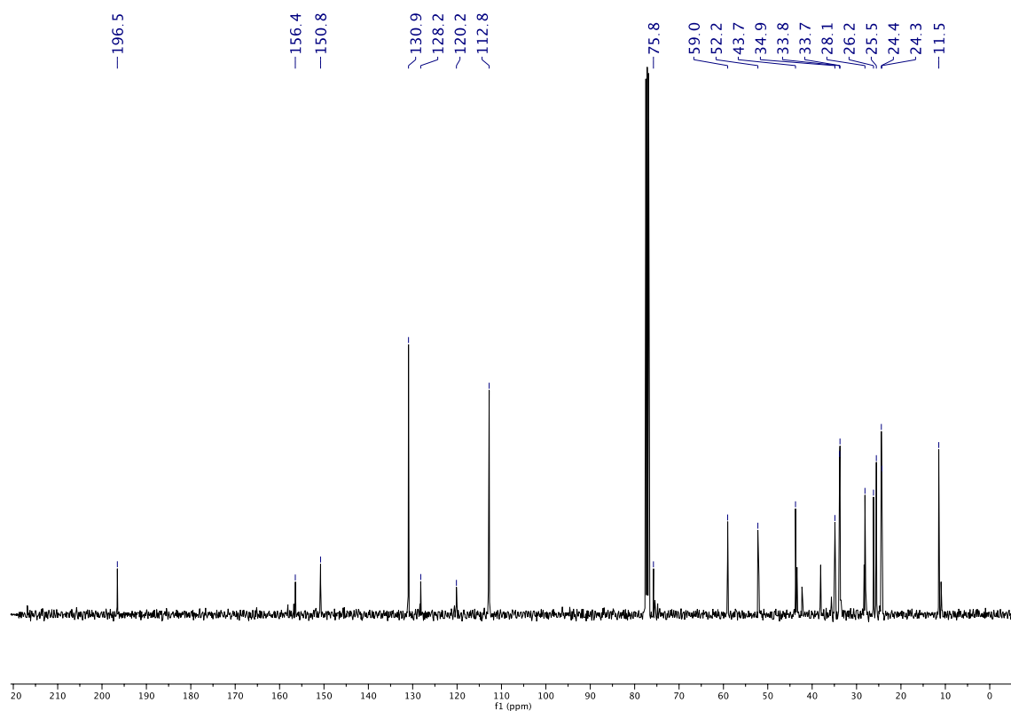
Figure 40. New submission 13 C NMR spectrum in CDCl 3 of compound 2p .
