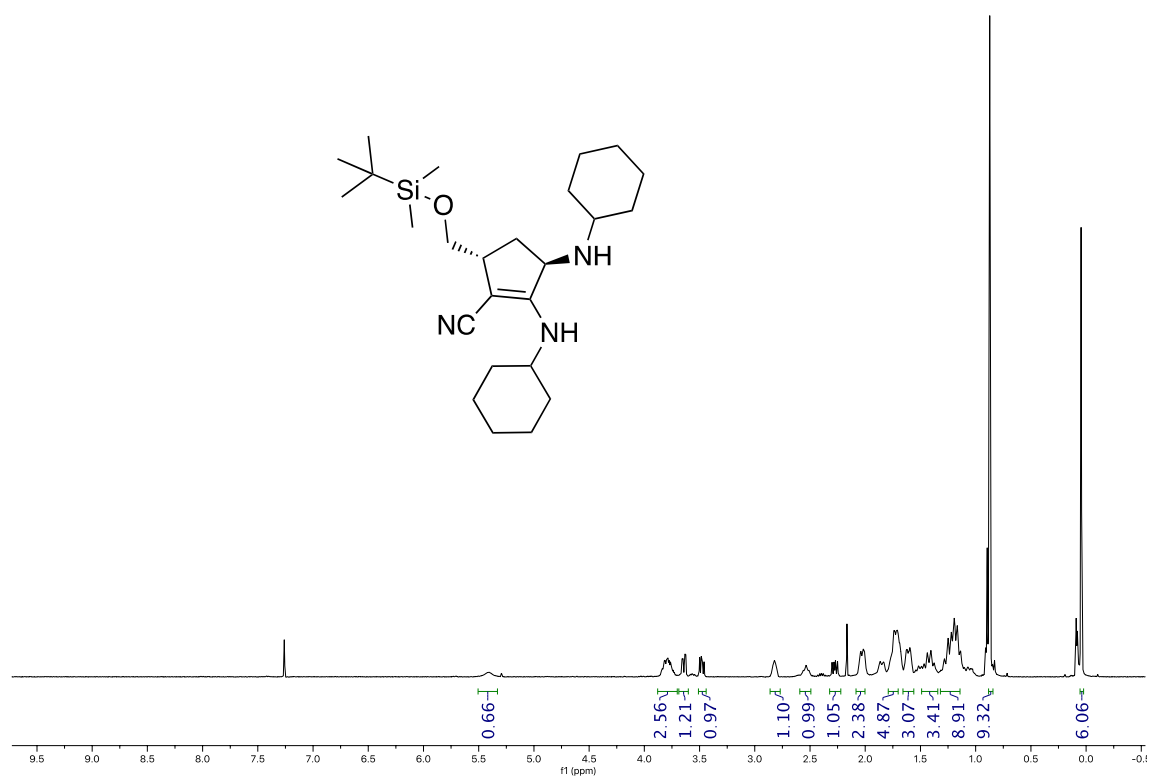
Figure 41. First submission 1 H NMR spectrum in CDCl 3 of compound 2ag .
