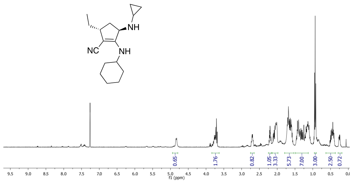
Figure 17. First submission 1 H NMR spectrum in CDCl 3 of compound 2b .
