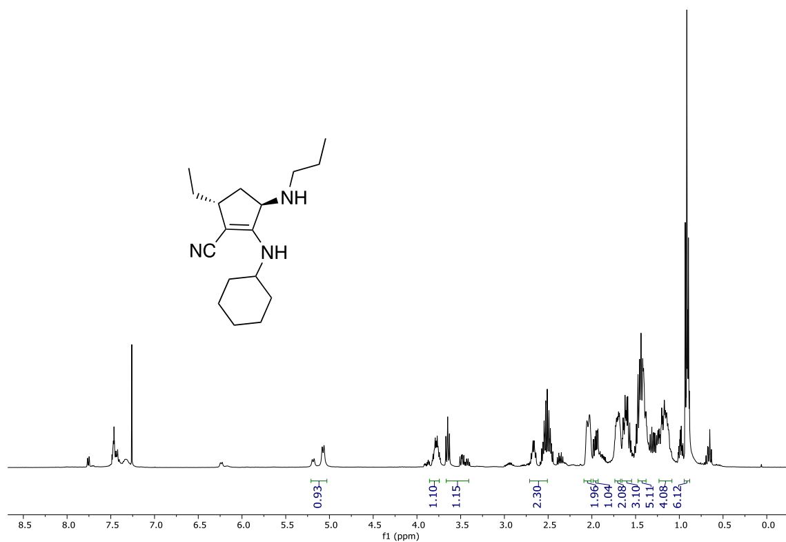
Figure 29. First submission 1 H NMR spectrum in CDCl 3 of compound 2g .
