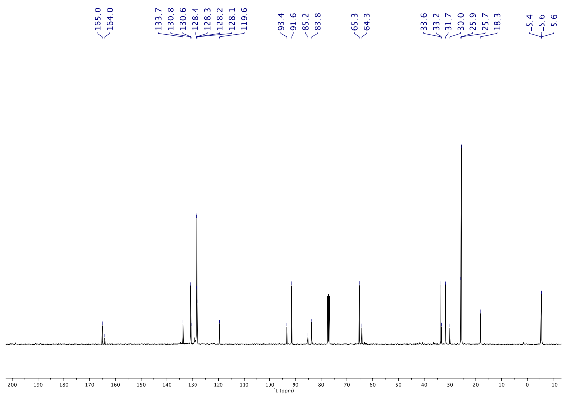
Figure 12. New submission 13 C NMR spectrum in CDCl 3 of compound 1g .
