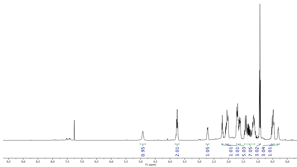
Figure 18. New submission 1 H NMR spectrum in CDCl 3 of compound 2b .
