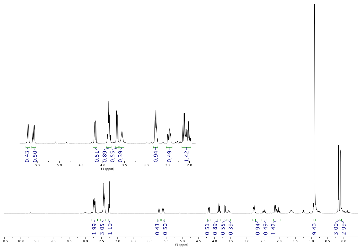
Figure 10. New submission 1 H NMR spectrum in CDCl 3 of compound 1g .
