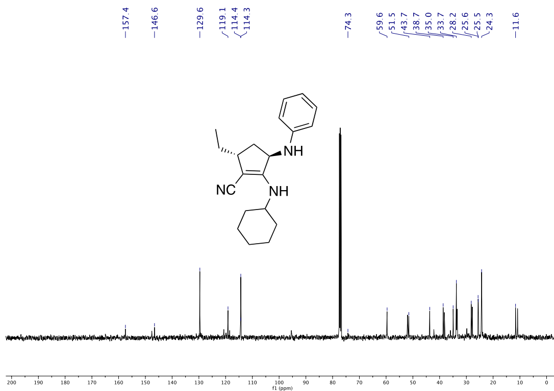
Figure 35. First submission 13 C NMR spectrum in CDCl 3 of compound 2k .
