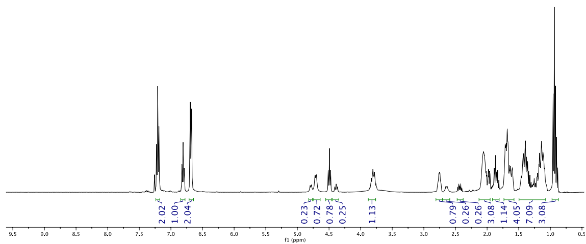
Figure 34. New submission 1 H NMR spectrum in CDCl 3 of compound 2k .
