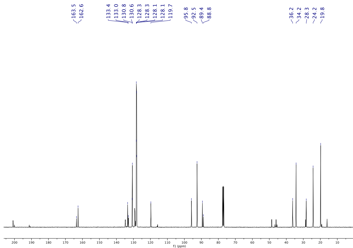
Figure 4. New submission 13 C NMR spectrum in CDCl 3 of compound 1b .
