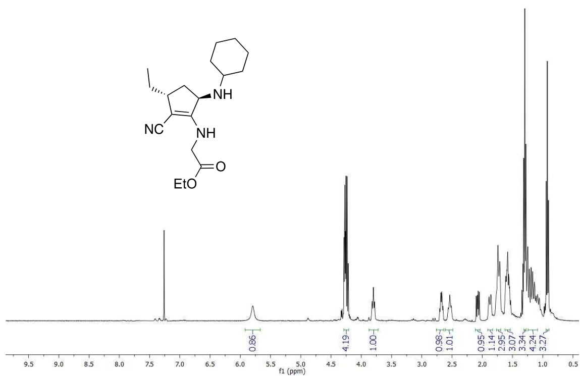
Figure 53. First submission 1 H NMR spectrum in CDCl 3 of compound 2ak .
