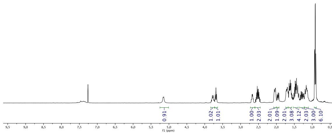
Figure 30. New submission 1 H NMR spectrum in CDCl 3 of compound 2g .
