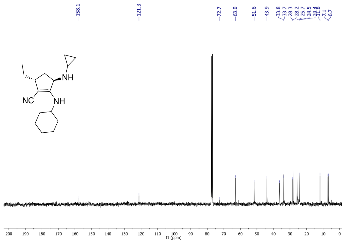
Figure 19. First submission ^{13}\text{C} NMR spectrum in CDCl 3 of compound 2b .
