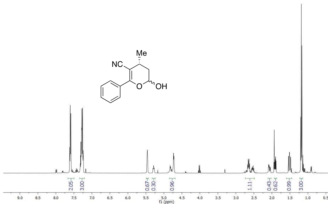
Figure 1. First submission 1 H NMR spectrum in CDCl 3 of compound 1b .
