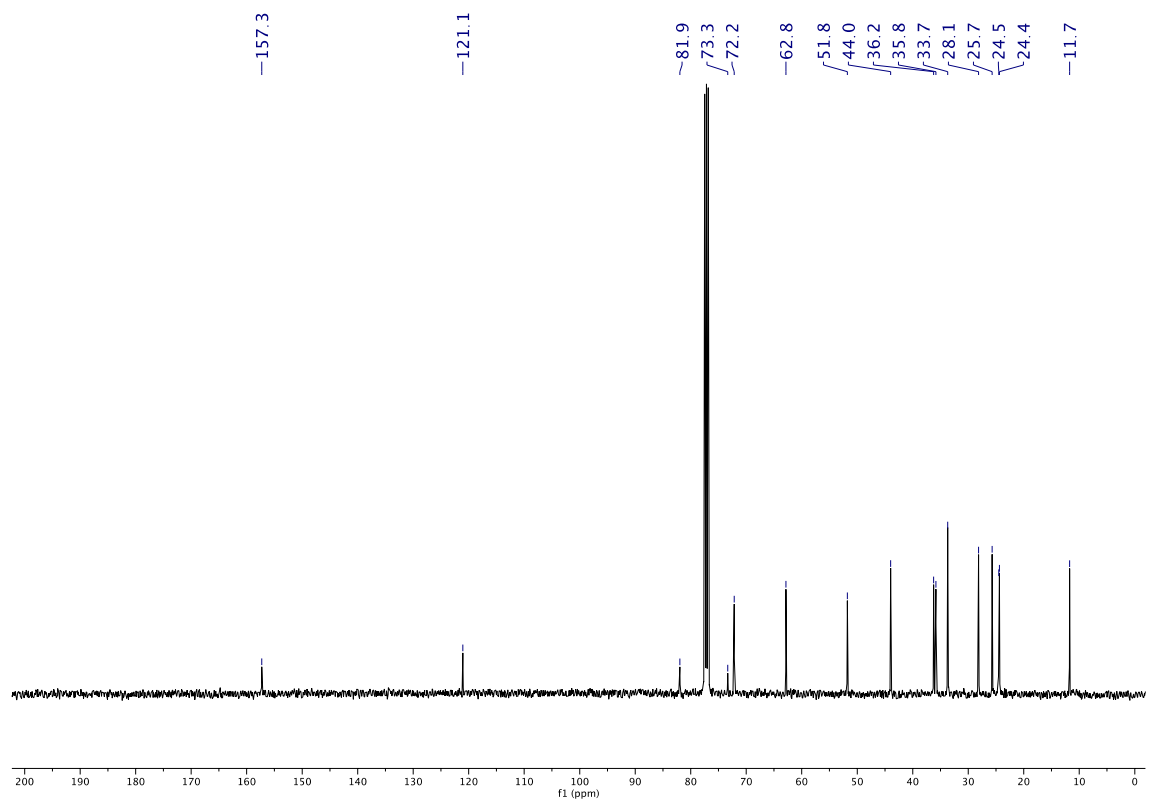
Figure 24. New submission 13 C NMR spectrum in CDCl 3 of compound 2e .
