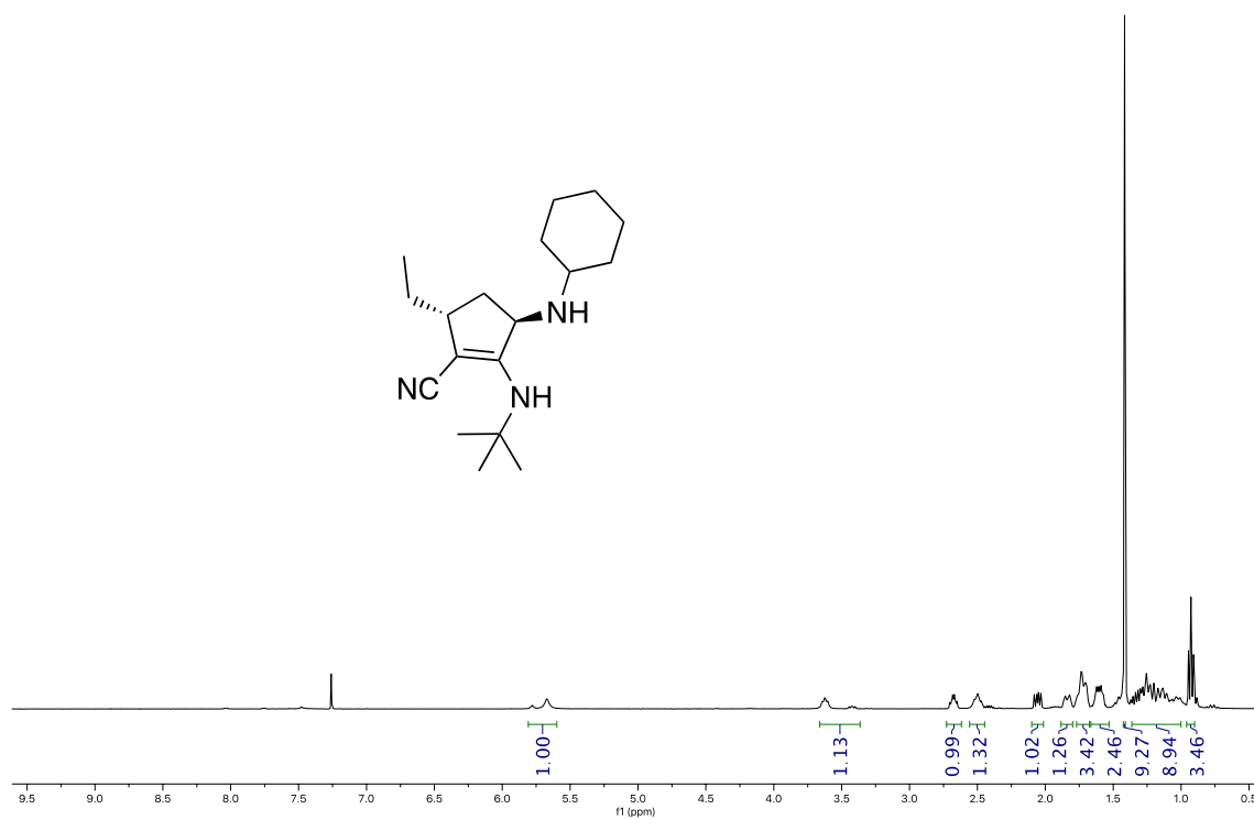
Figure 45. First submission 1 H NMR spectrum in CDCl 3 of compound 2ai .
