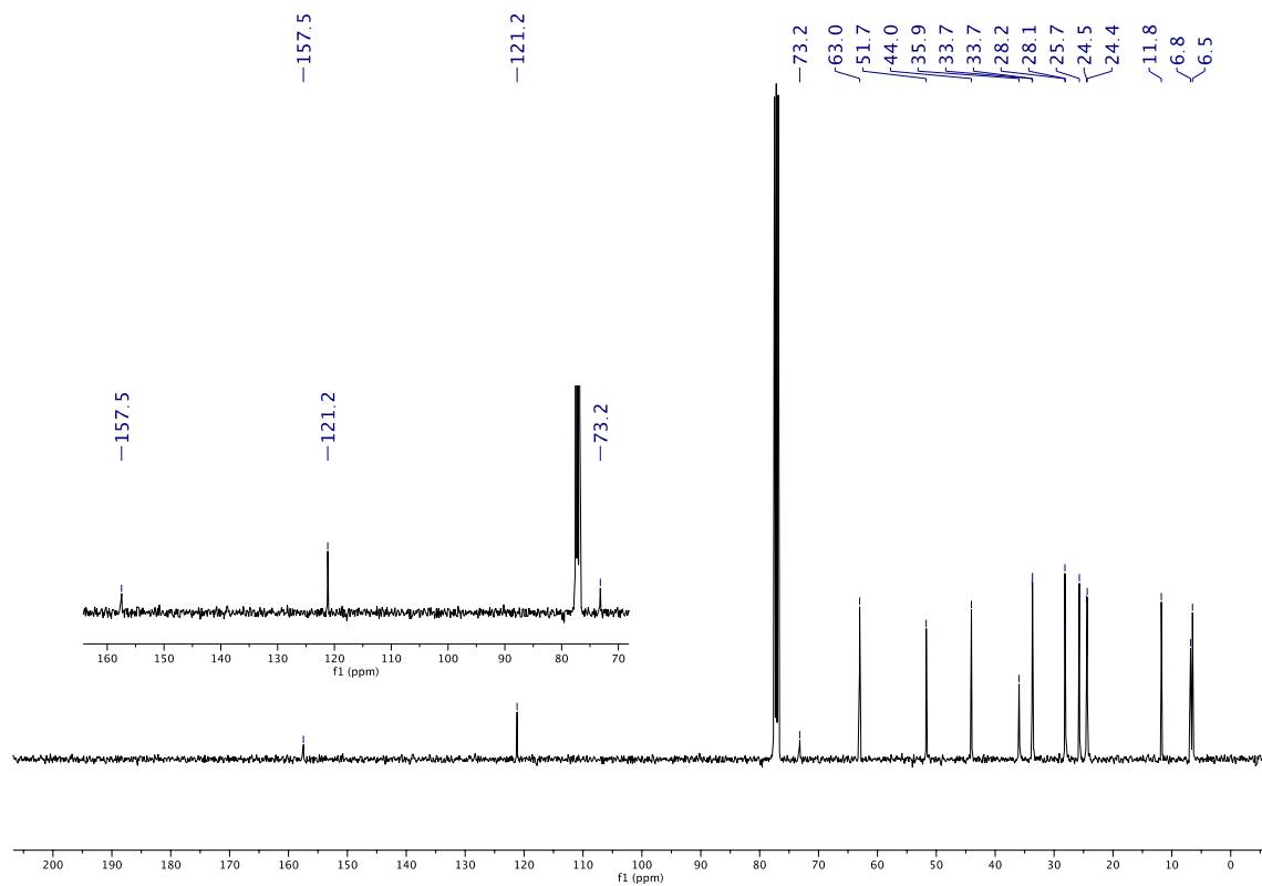
Figure 20. New submission ^{13}\text{C} NMR spectrum in CDCl 3 of compound 2b .
