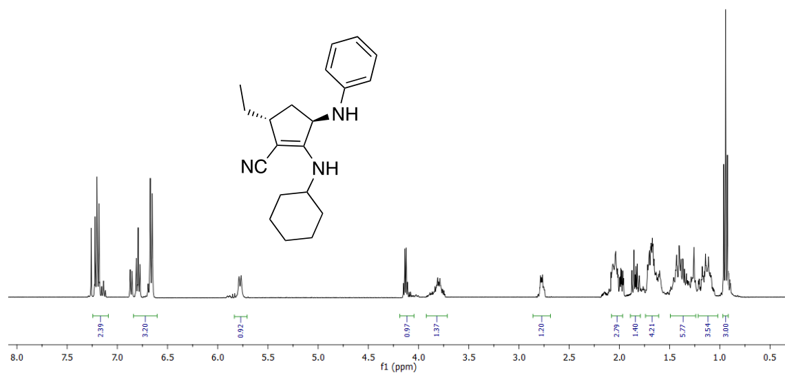
Figure 33. First submission 1 H NMR spectrum in CDCl 3 of compound 2k .
