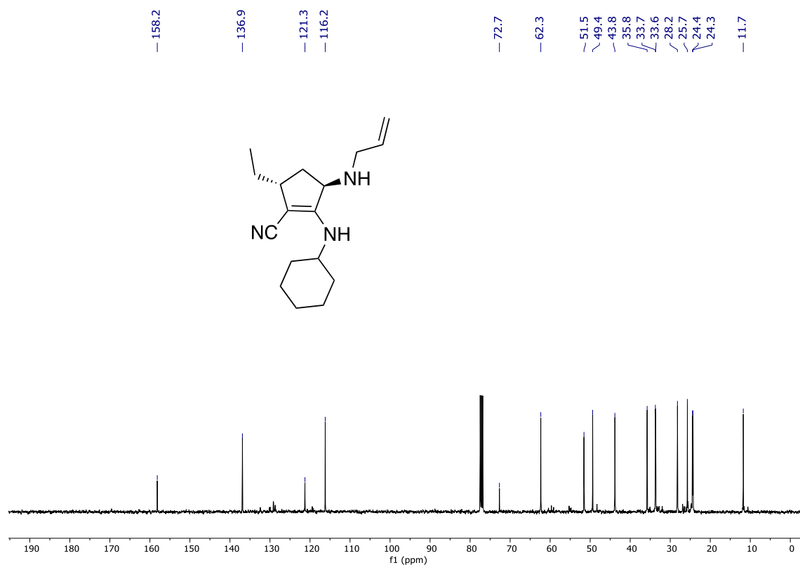
Figure 27. First submission 13 C NMR spectrum in CDCl 3 of compound 2f .
