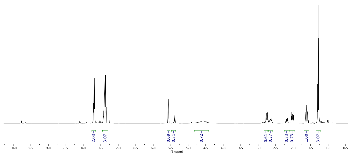
Figure 2. New submission 1 H NMR spectrum in CDCl 3 of compound 1b .
