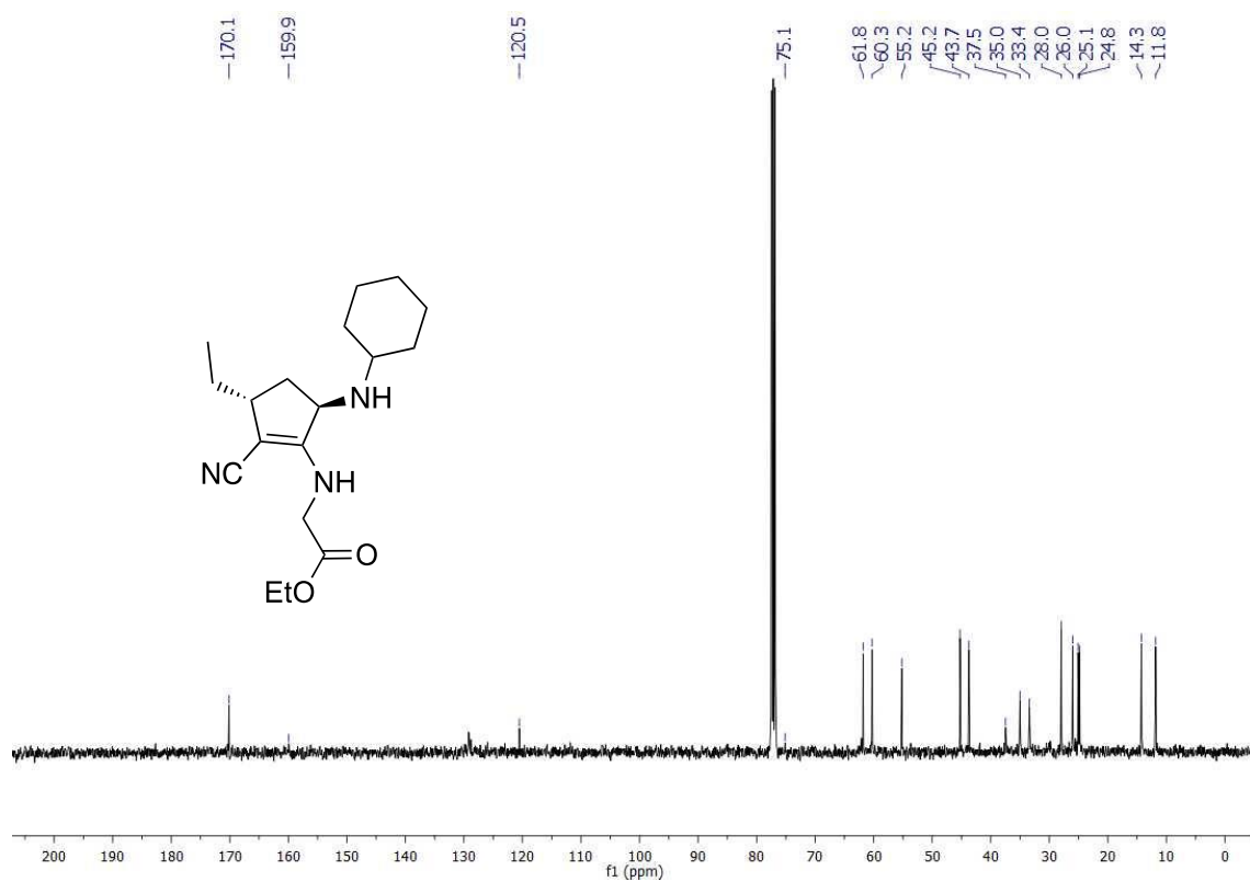
Figure 55. First submission 13 C NMR spectrum in CDCl 3 of compound 2ak .
