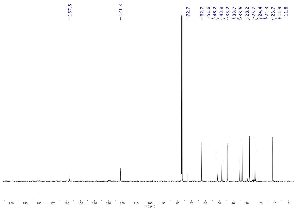
Figure 32. New submission 13 C NMR spectrum in CDCl 3 of compound 2g .
