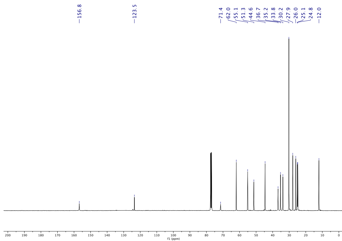
Figure 48. New submission 13 C NMR spectrum in CDCl 3 of compound 2ai .
