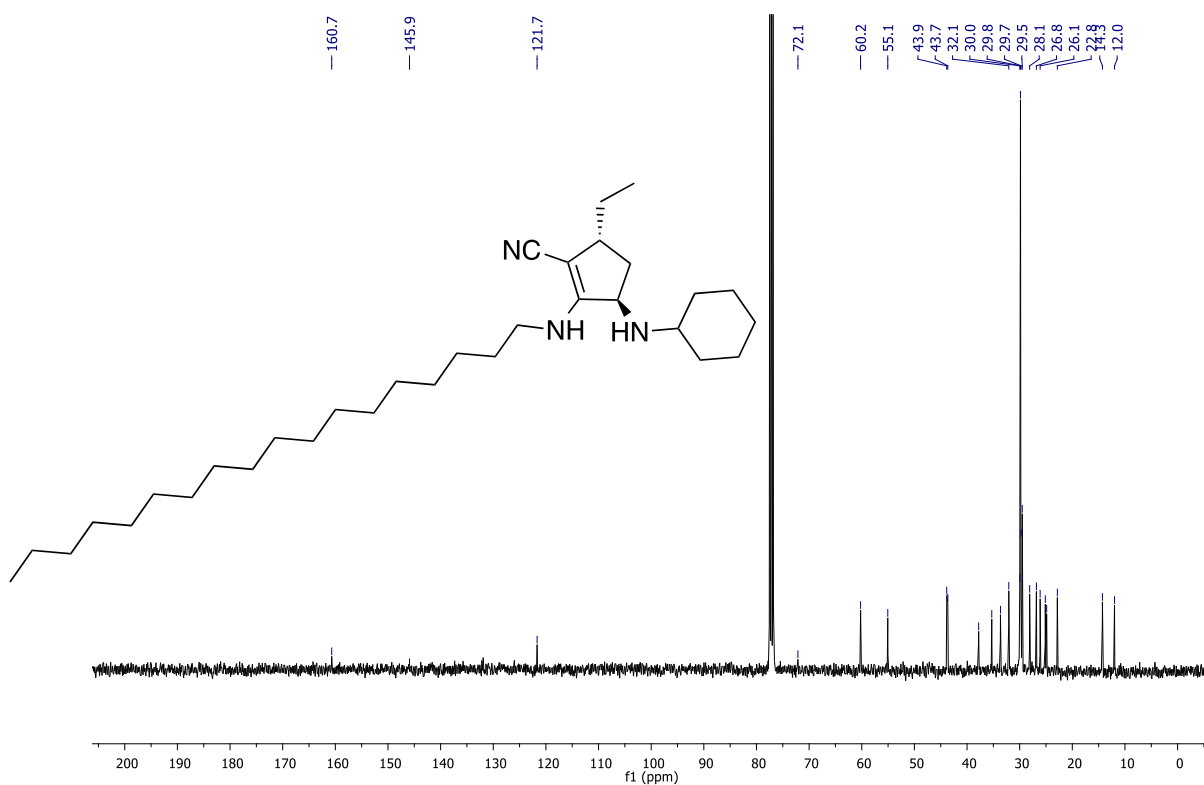
Figure 51. First submission 13 C NMR spectrum in CDCl 3 of compound 2aj .
