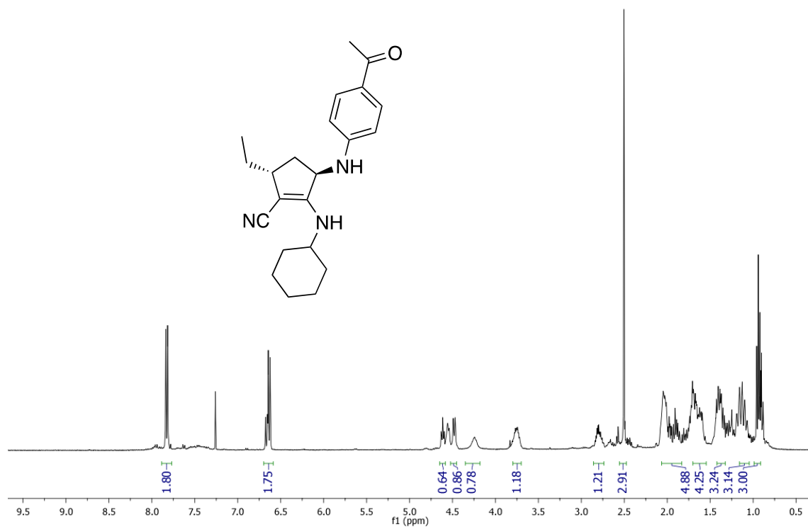
Figure 37. First submission 1 H NMR spectrum in CDCl 3 of compound 2p .
