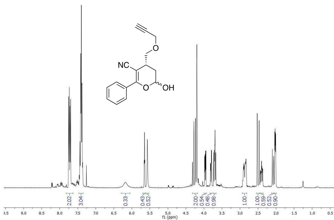
Figure 13. First submission 1 H NMR spectrum in CDCl 3 of compound 1h .
