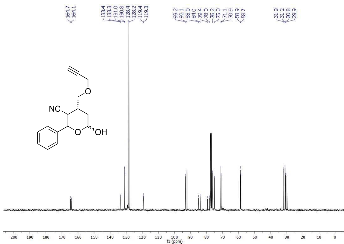
Figure 15. First submission 13 C NMR spectrum in CDCl 3 of compound 1h .
