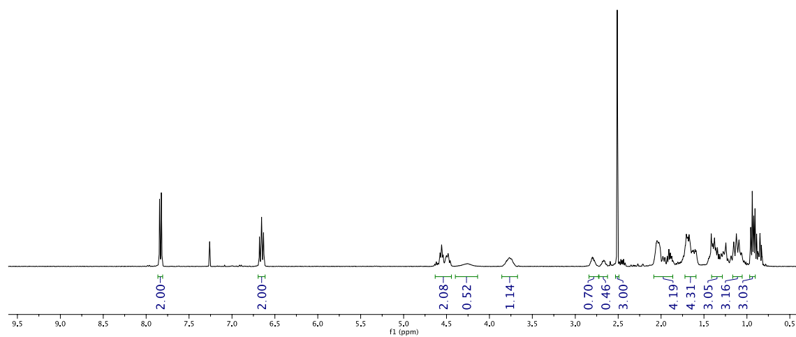
Figure 38. New submission 1 H NMR spectrum in CDCl 3 of compound 2p .
