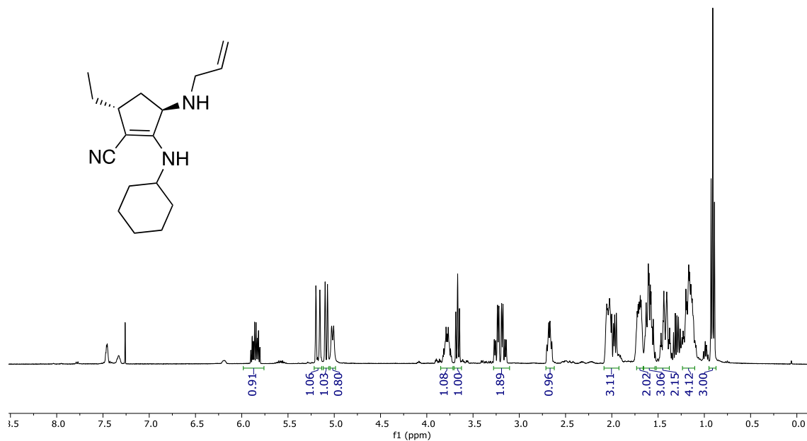
Figure 25. First submission 1 H NMR spectrum in CDCl 3 of compound 2f .
