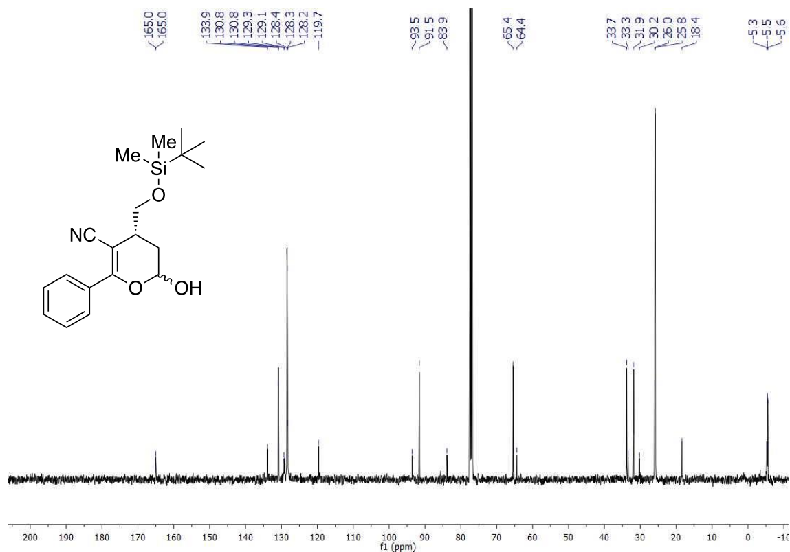
Figure 11. First submission 13 C NMR spectrum in CDCl 3 of compound 1g .
