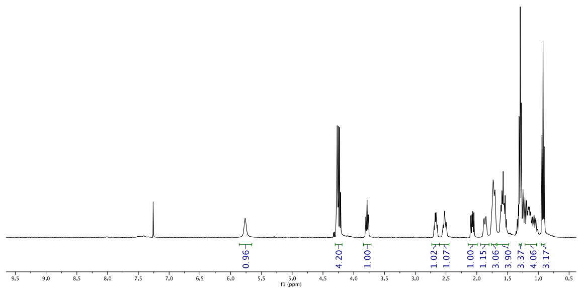
Figure 54. New submission 1 H NMR spectrum in CDCl 3 of compound 2ak .
