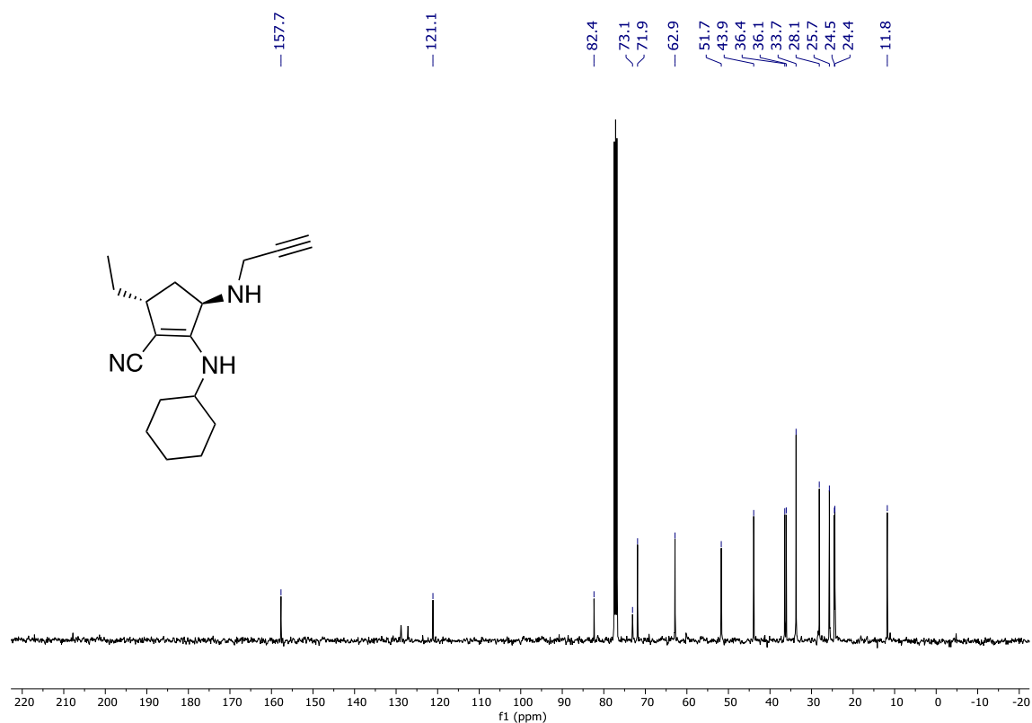
Figure 23. First submission 13 C NMR spectrum in CDCl 3 of compound 2e .
