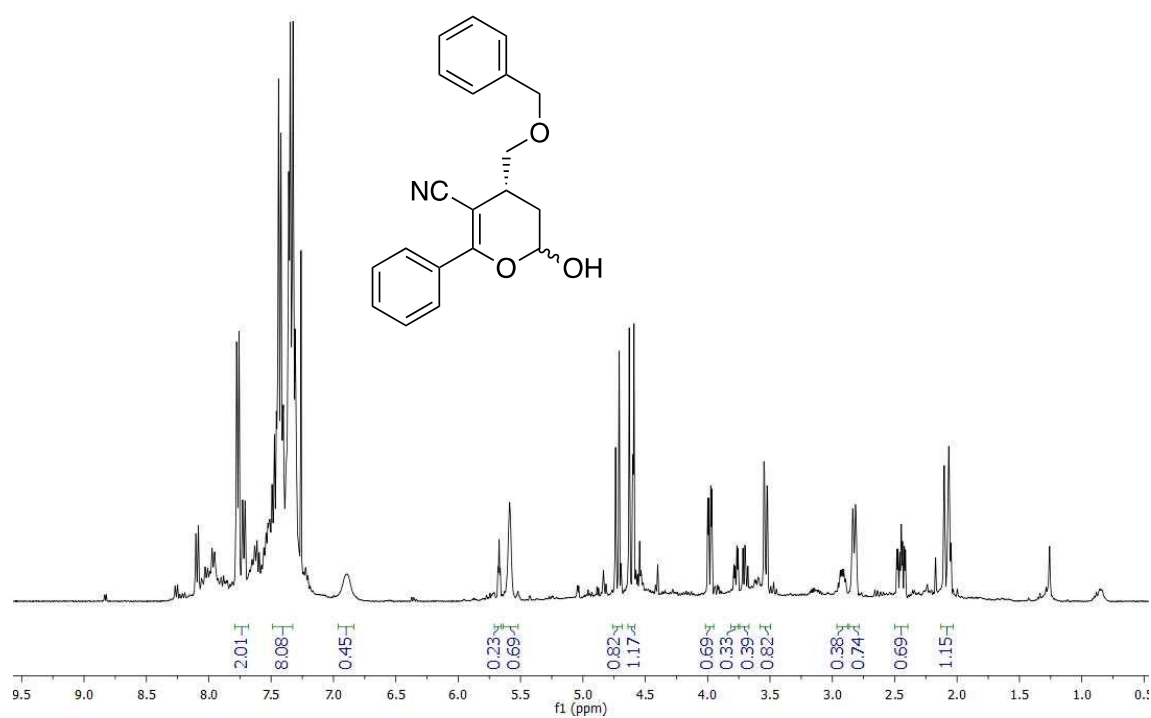
Figure 5. First submission 1 H NMR spectrum in CDCl 3 of compound 1f .
