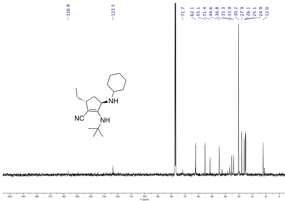
Figure 47. First submission 13 C NMR spectrum in CDCl 3 of compound 2ai .
