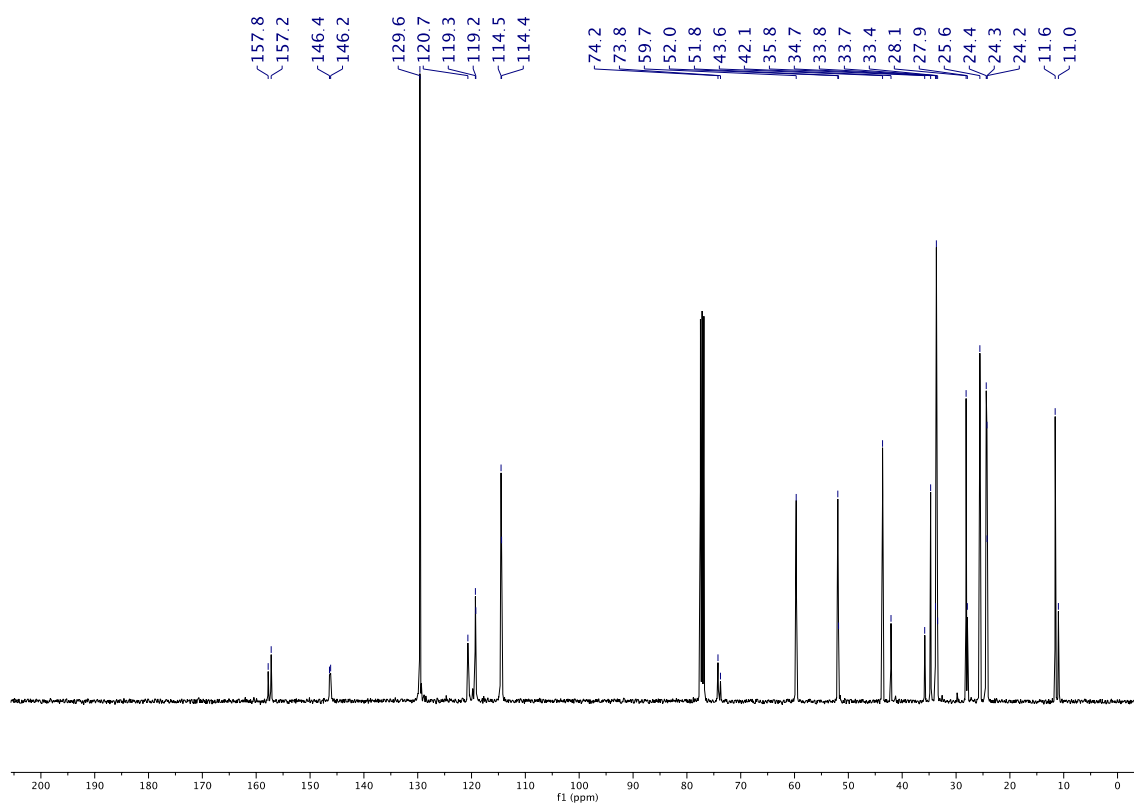
Figure 36. New submission 13 C NMR spectrum in CDCl 3 of compound 2k .
