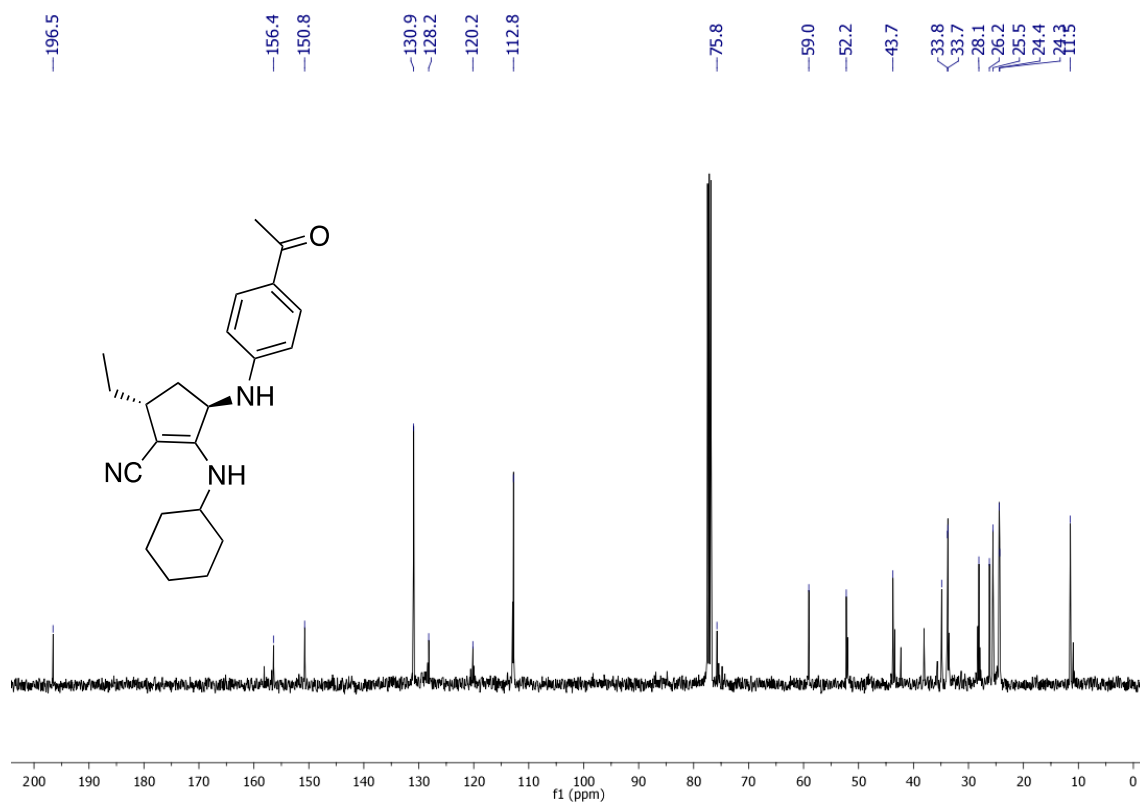
Figure 39. First submission 13 C NMR spectrum in CDCl 3 of compound 2p .
