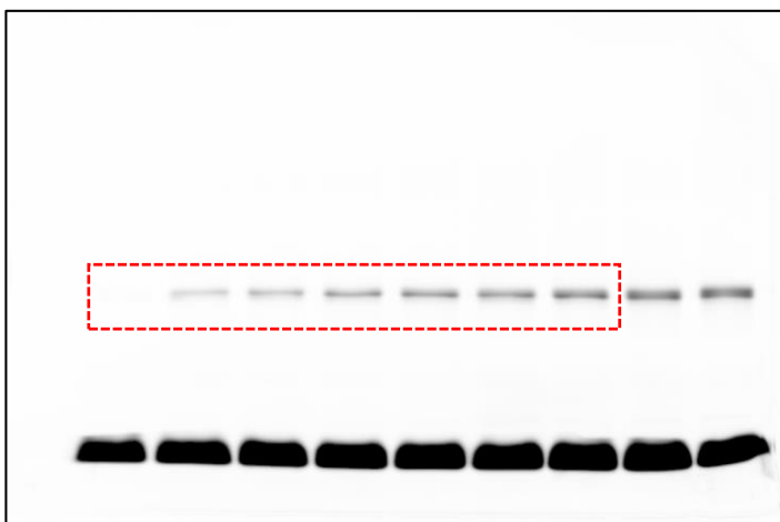
In-gel fluorescence
