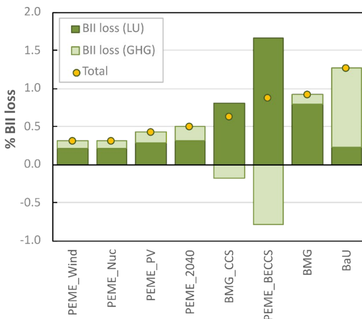
Figure A1 Contribution of the environmental stressors to the PB of biosphere integrity. The bars are arranged in ascending order of total impact. (BII: biodiversity intactness index; LU: land use stressor; GHG: greenhouse gas emissions stressor).
