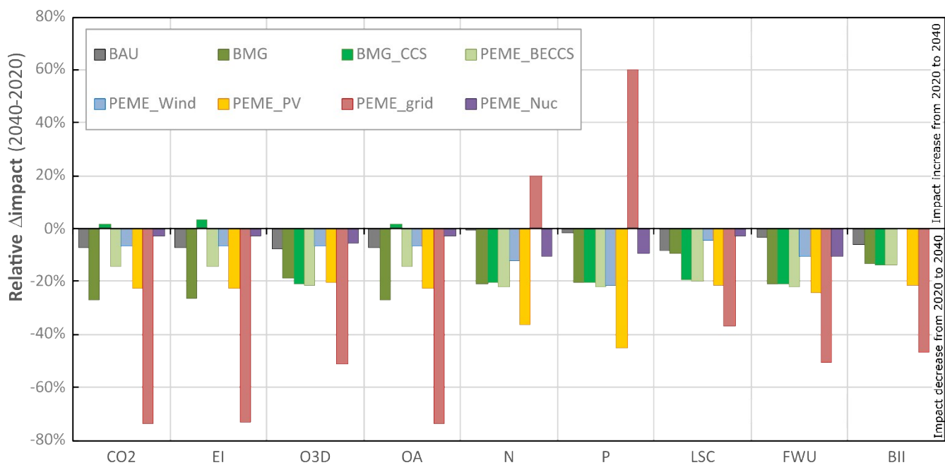
Figure A2 Relative impact variation between 2040 and 2020 scenarios. Negative values denote better performance for the 2040 scenario under the specific control variables of the PBs. (CO 2 : Atmospheric CO 2 concentration; EI: Energy imbalance at the top of atmosphere; O 3 D: Stratospheric ozone depletion; OA: Ocean acidification; P: Biogeochemical phosphorus flow, global; N: Biogeochemical nitrogen flow, global; LSC: Land-system change, global; FWU: Freshwater use, global; BII: Biosphere integrity).
