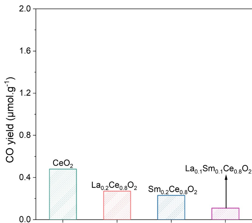
Fig. S2. CO 2 splitting performance of the support materials.
