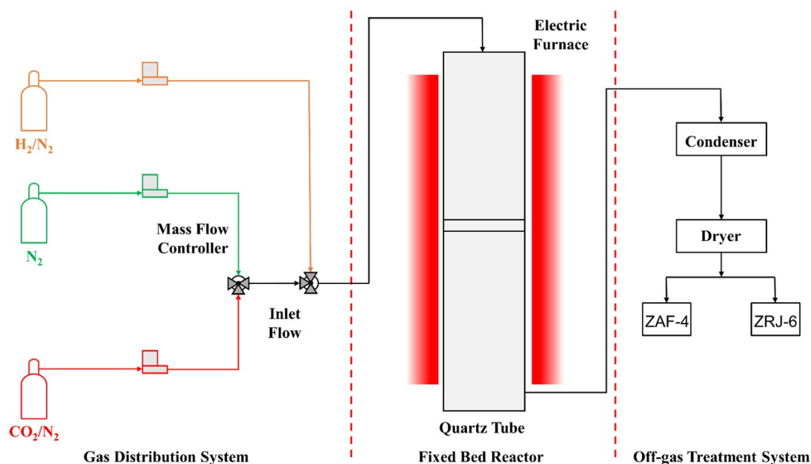
Fig. S1. Schematic of the fixed-bed reactor.
