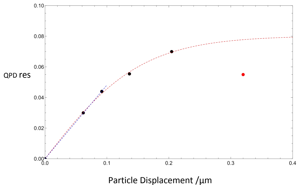
Supplementary Figure 1. Calibration line for the QPD voltage output versus particle position. Blue dashed line is for the line fitting at small displacement.
