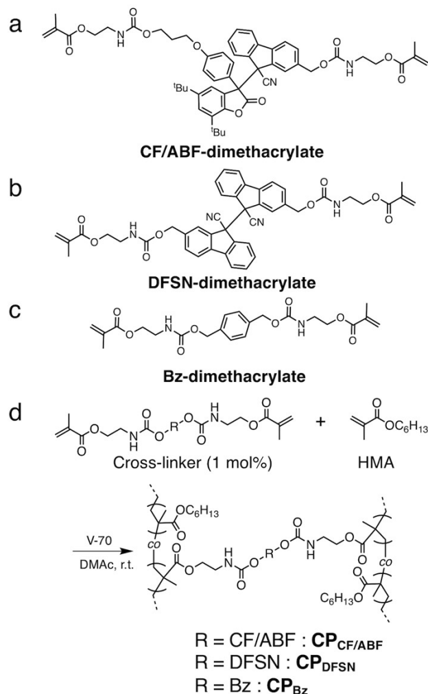
Fig. 2 Chemical structures of (a) CF/ABF-dimethacrylate, (b) DFSN-dimethacrylate and (c) Bz-dimethacrylate. (d) Synthetic route to CP_{CF/ABF} , CP_{DFS} and CP_{Bz} .
