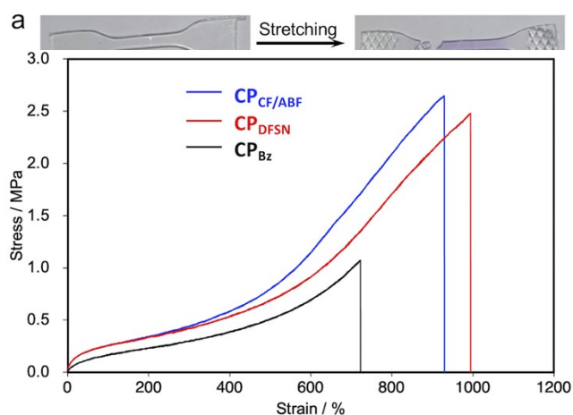
Fig. 5 Stress-strain curves of \text{CP}_{\text{CF/ABF}} (blue), \text{CP}_{\text{DFSN}} (red) and \text{CP}_{\text{Bz}} (black) films (100 mm/min, 30 °C).
