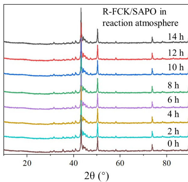
Fig. R1 In-situ XRD pattern of R-FCK/SAPO in reaction atmosphere
