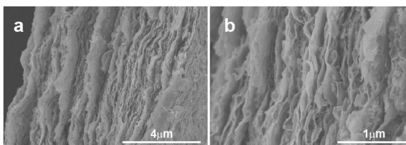
Figure s2. (a and b) SEM images of the used MXene/CNT@MnO 2 film electrode at
