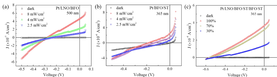
S2 (a-c) the J-V curves under the illumination of 365 and 500 nm with different power densities for Pt/LNO/BFO, Pt/BFO/ST, and Pt/LNO/BFO/ST/BFO/ST multilayer films.
