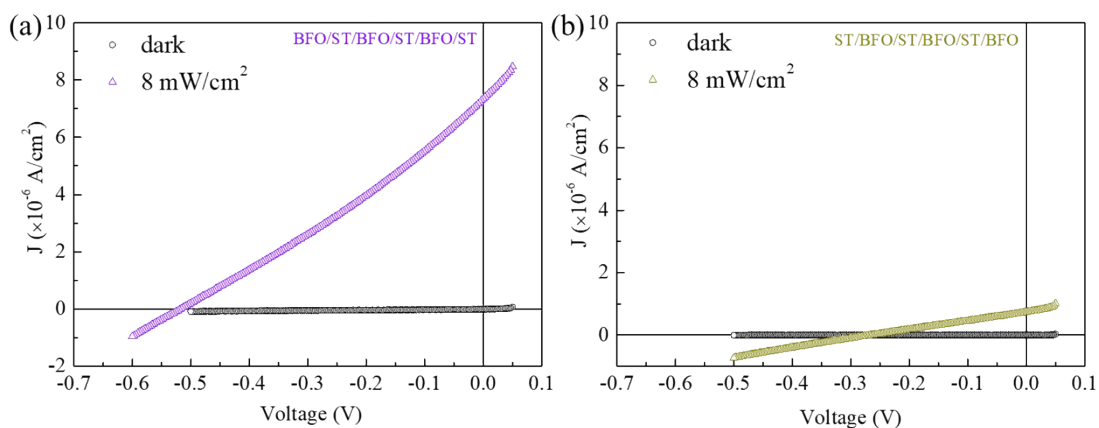
S1 (a-b) the J-V curves under the illumination of 365 nm with 8 mW/cm 2 for BFO/ST/BFO/ST/BFO/ST and ST/BFO/ST/BFO/ST/BFO multilayer films.
