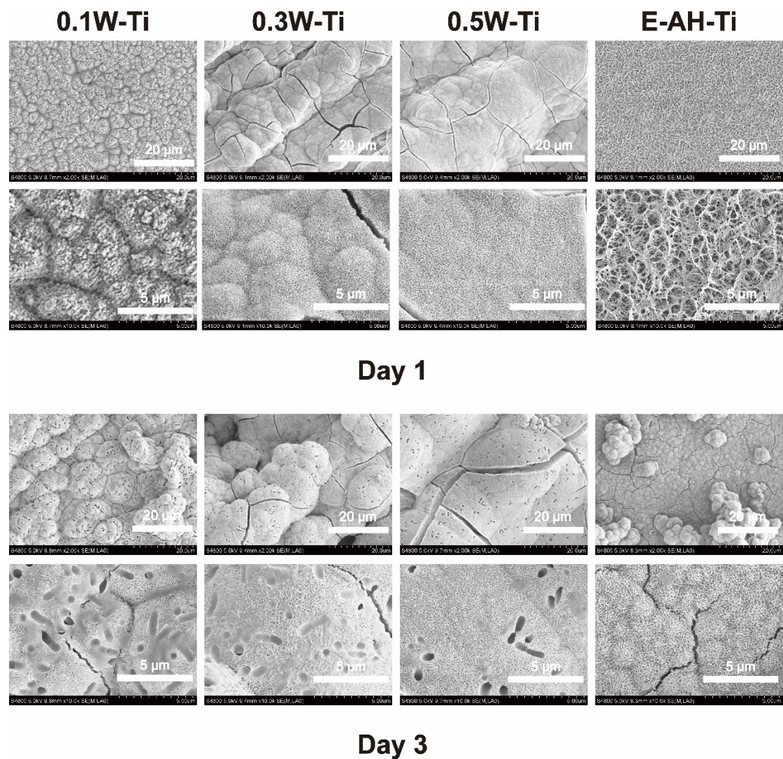
Figure S1. SEM micrographs with higher magnification of 0.1W-Ti, 0.3W-Ti, 0.5W-Ti and E-AH-Ti after soaking in SBF for 1 day and 3 days.
