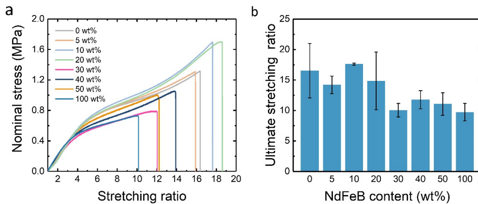
Figure S1. (a) Stress-strain curves and (b) ultimate stretching ratio for magnetic hydrogels with different NdFeB concentrations. The curves for 0, 5, 10, and 20 wt% have been shown in Figure 3b.
