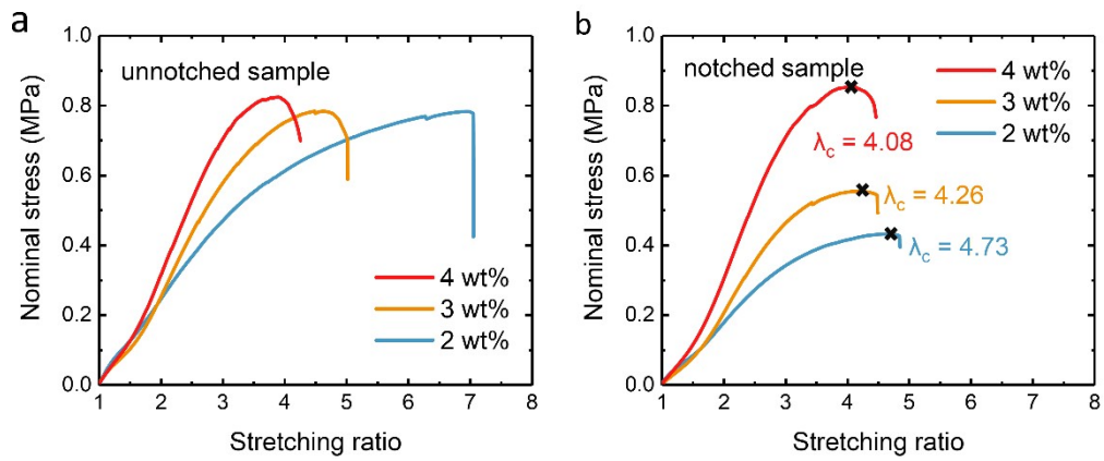
Figure S2. Stress-strain curves of the pure-shear test for magnetic hydrogels with different microgel content.
