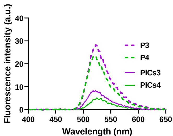
Figure S10. Fluorescence emission spectra of FITC labelled BSA-PDMAEMA conjugates (P3 and P4) and their respective PICs nanoparticles (PICs3 and PICs4) ( \lambda_{\text{ex}}/\lambda_{\text{em}} = 490 \text{ nm}/530 \text{ nm} ) in HEPES buffer
