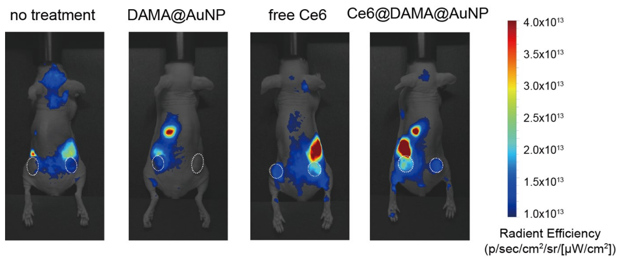
Figure S3. In vivo fluorescence images of A549 tumor-bearing mice treated with no treatment, DAMA@AuNPs, free Ce6, and Ce6@DAMA@AuNPs after 9 h post injection.
