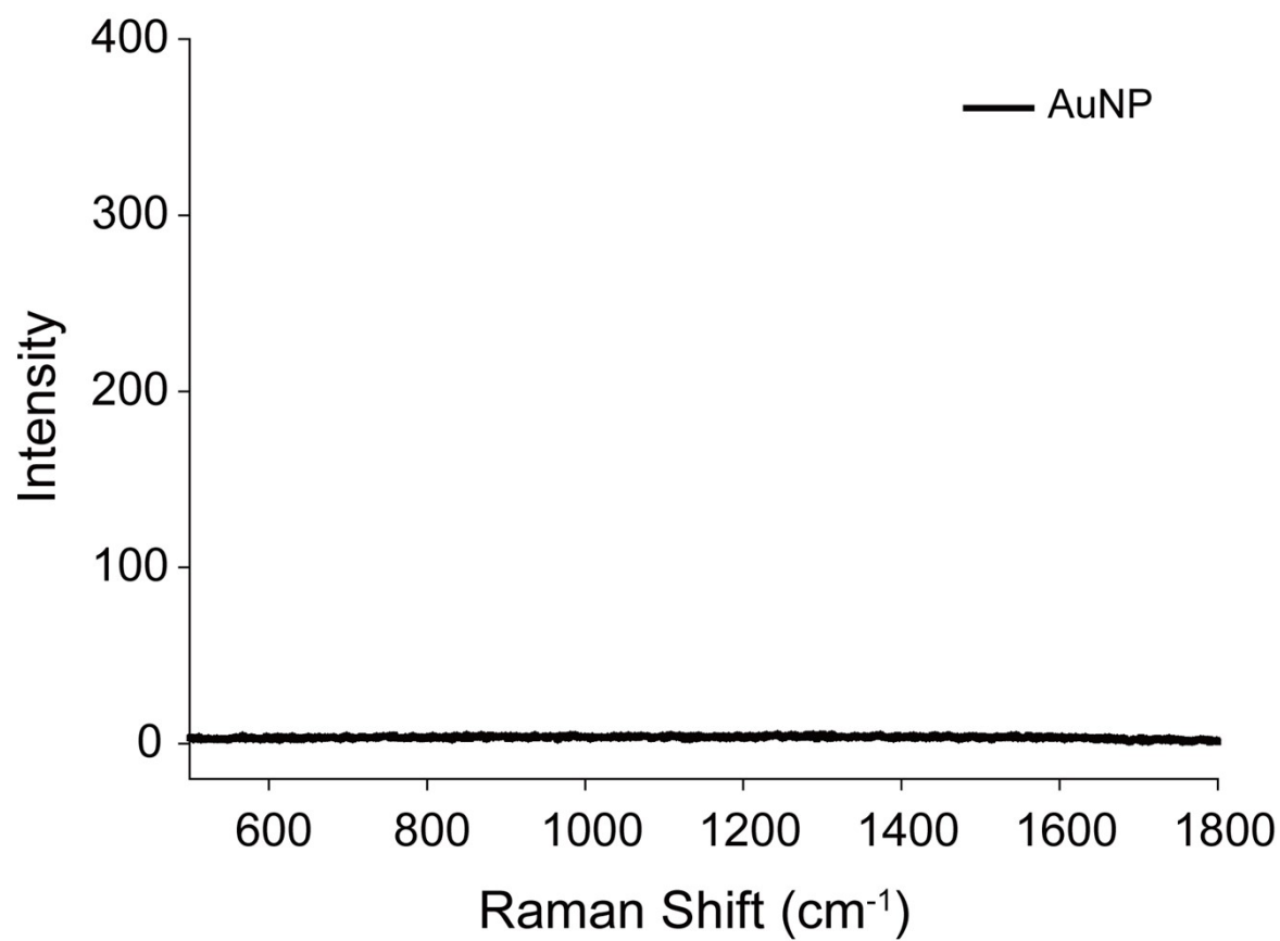
Figure S1. Raman spectrum of AuNP.
