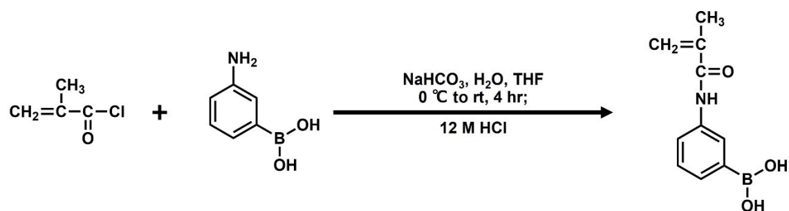
Scheme S1. Synthesis of 3-methacrylamidophenylboronic acid (MAPBA).
