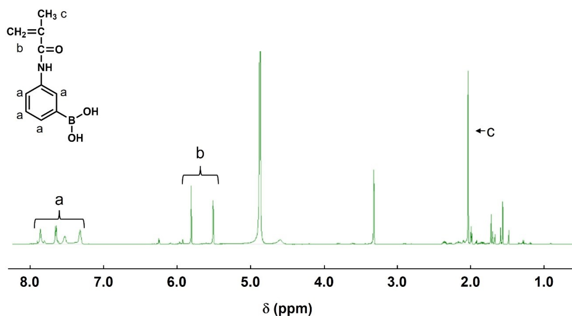
Figure S1. ^1\text{H-NMR} spectrum of MAPBA in methanol- d_4 .
