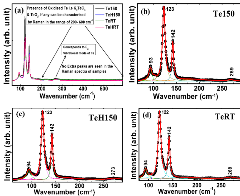
Fig. S2 (a) Raman spectra range 50-600 \text{cm}^{-1} and Multipeak Lorentzian fitting of (b) Te150, (c) TeH150 and (d) TeRT.
