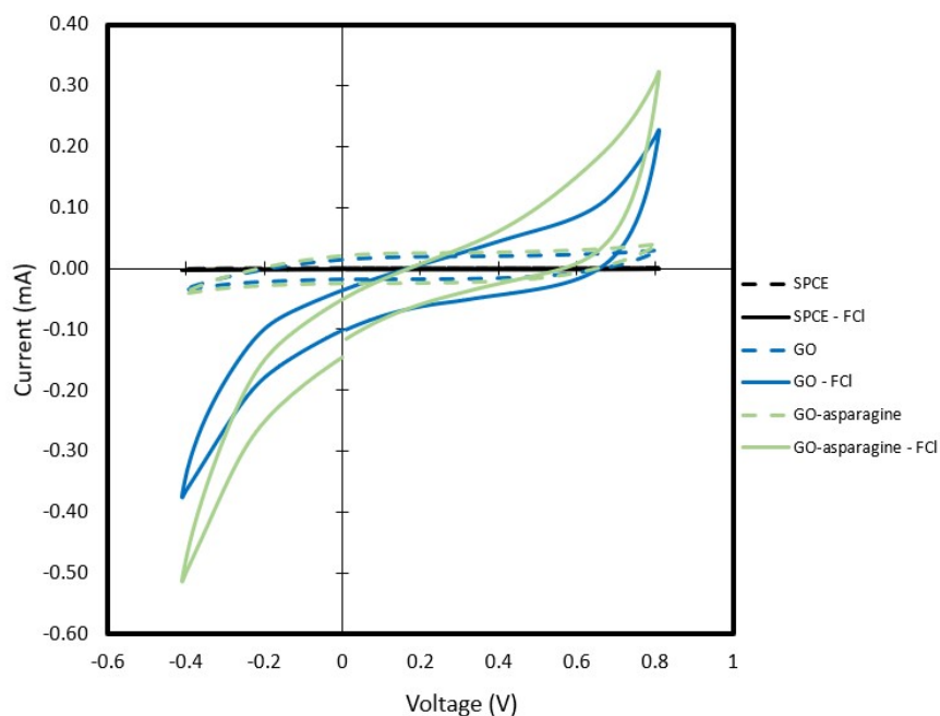
Fig. S1: Voltammetric Behavior of SPCE (black), SPCE/GO (blue), SPCE/GO-asparagine (green) where the dashed lines represent the absence of free chlorine and solid lines represent the addition of ~220 ppm free chlorine.
