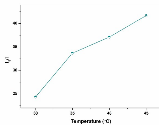
Fig S3: Temperature effect on fluorescence quenching of \beta -NAC
