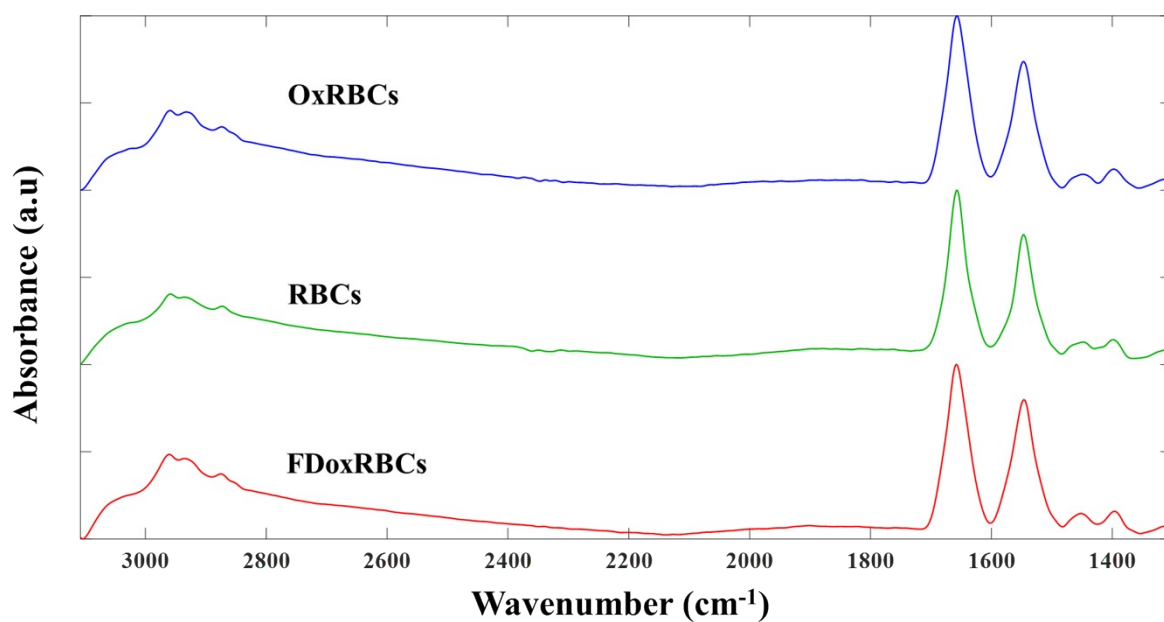
Figure S1: Baseline corrected averaged spectra from RBCs, OxRBCs, and FDox RBCs over 3100 – 1300 cm -1 region.
